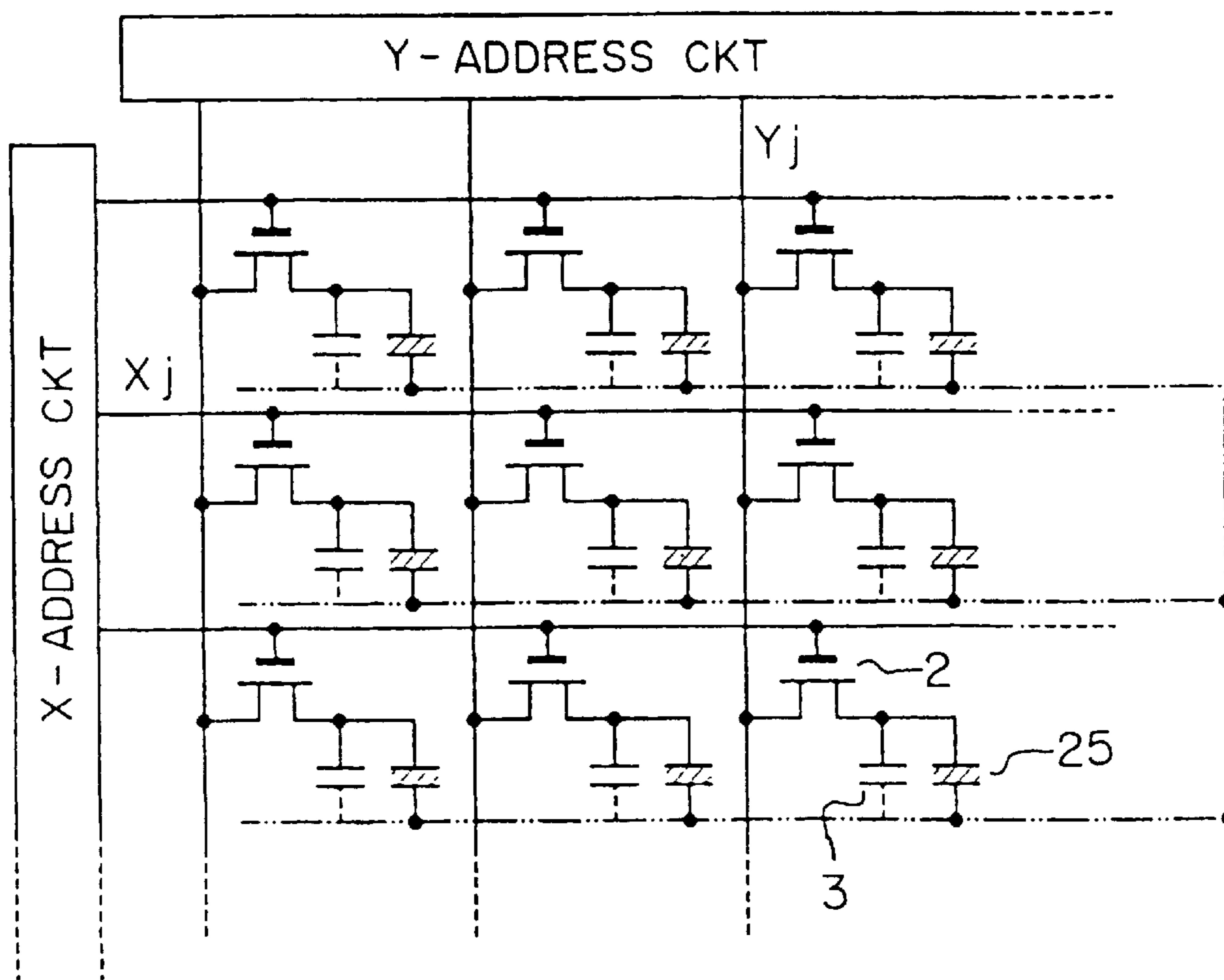
FIG. 2 (PRIOR ART)
