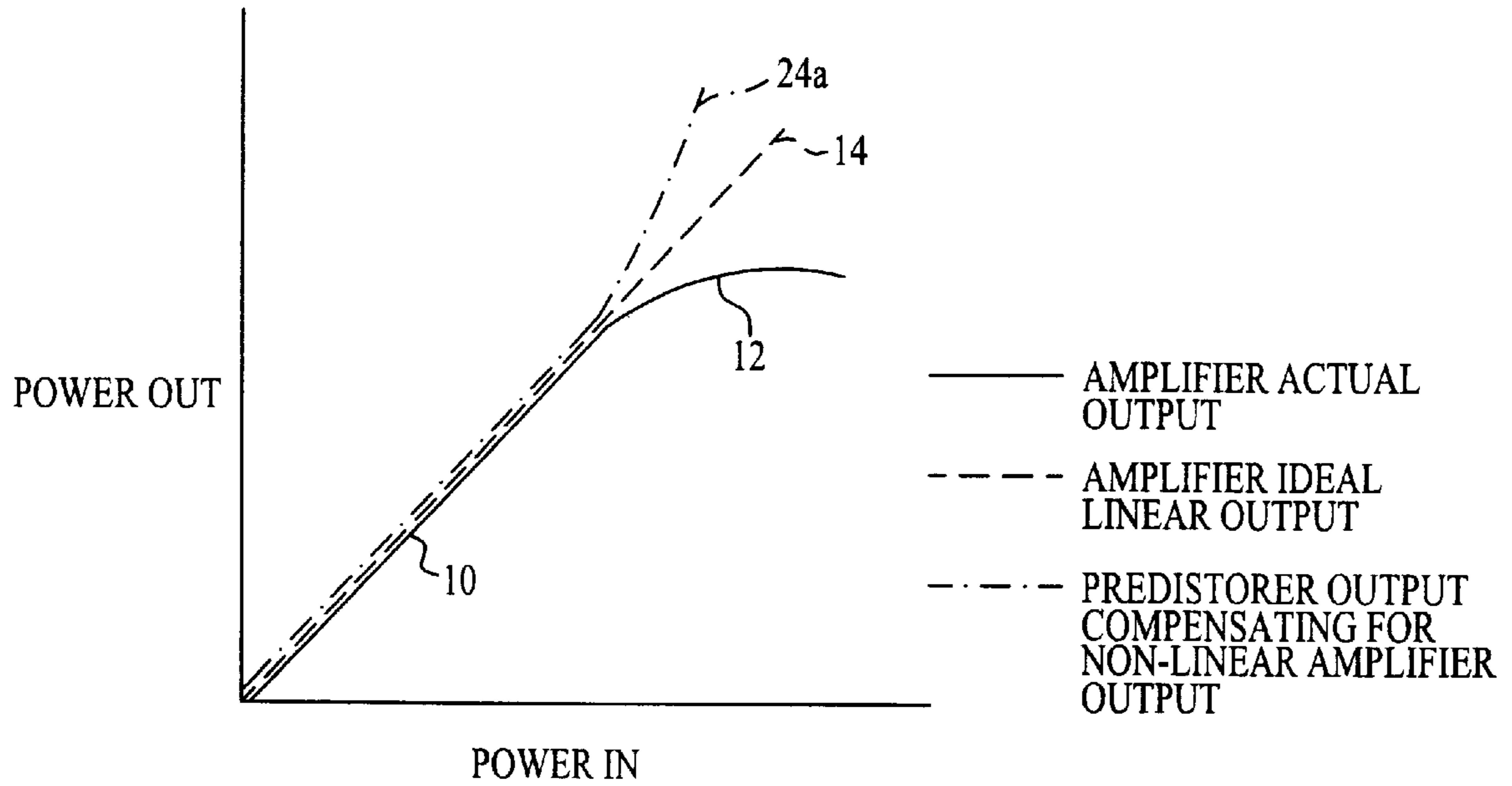
FIG. 1 (PRIOR ART)
