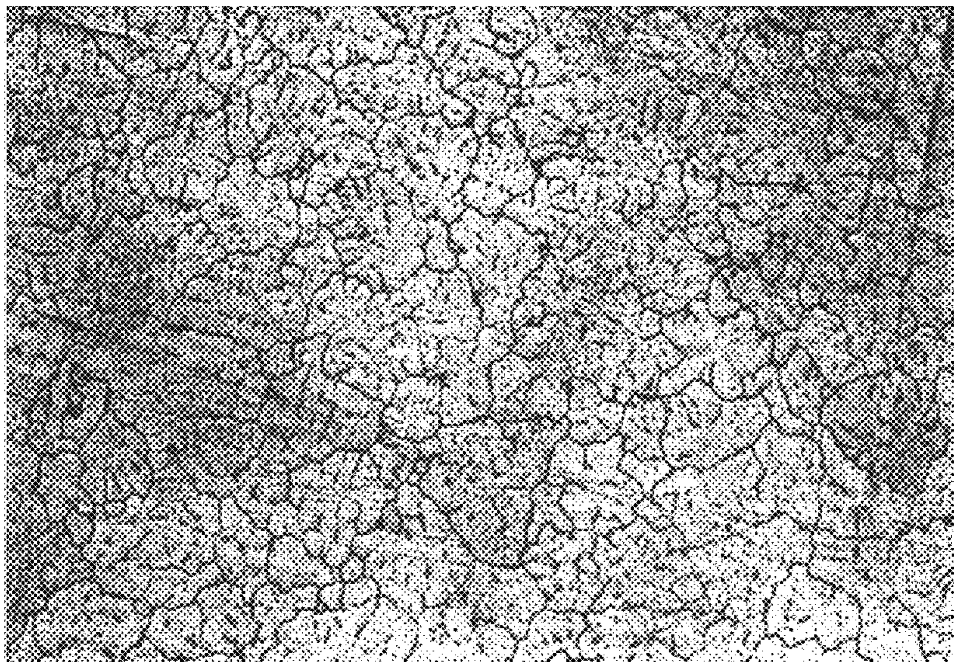
50X CENTRIFUGAL CAST AND HIPPED JC6061-T6C
