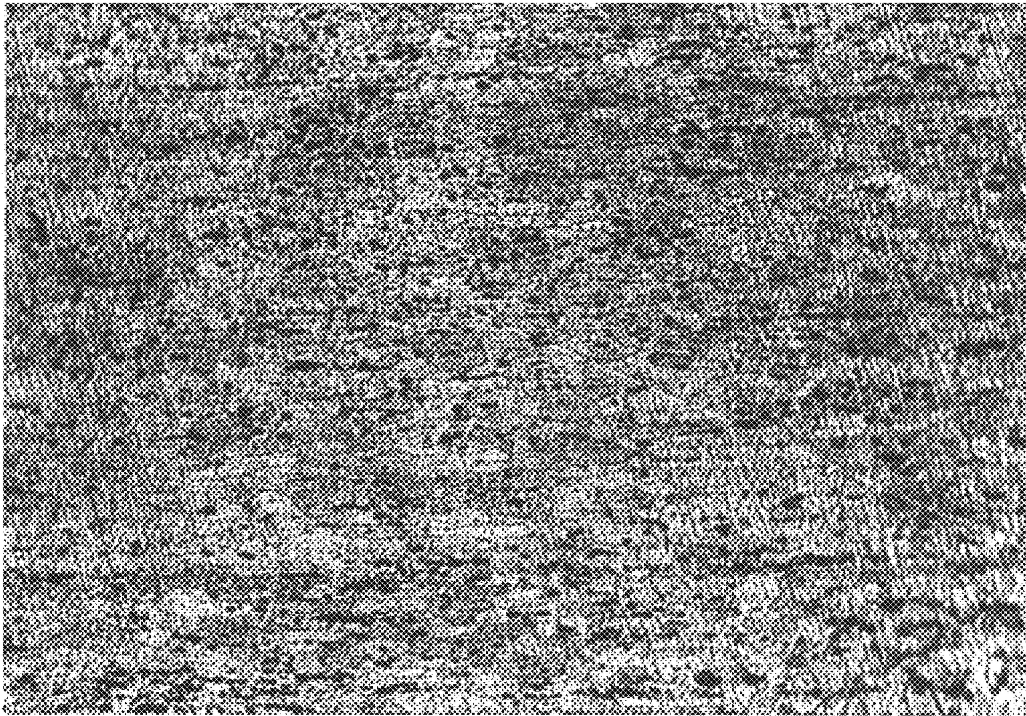
100X 6061-T651 WROUGHT PLATE
