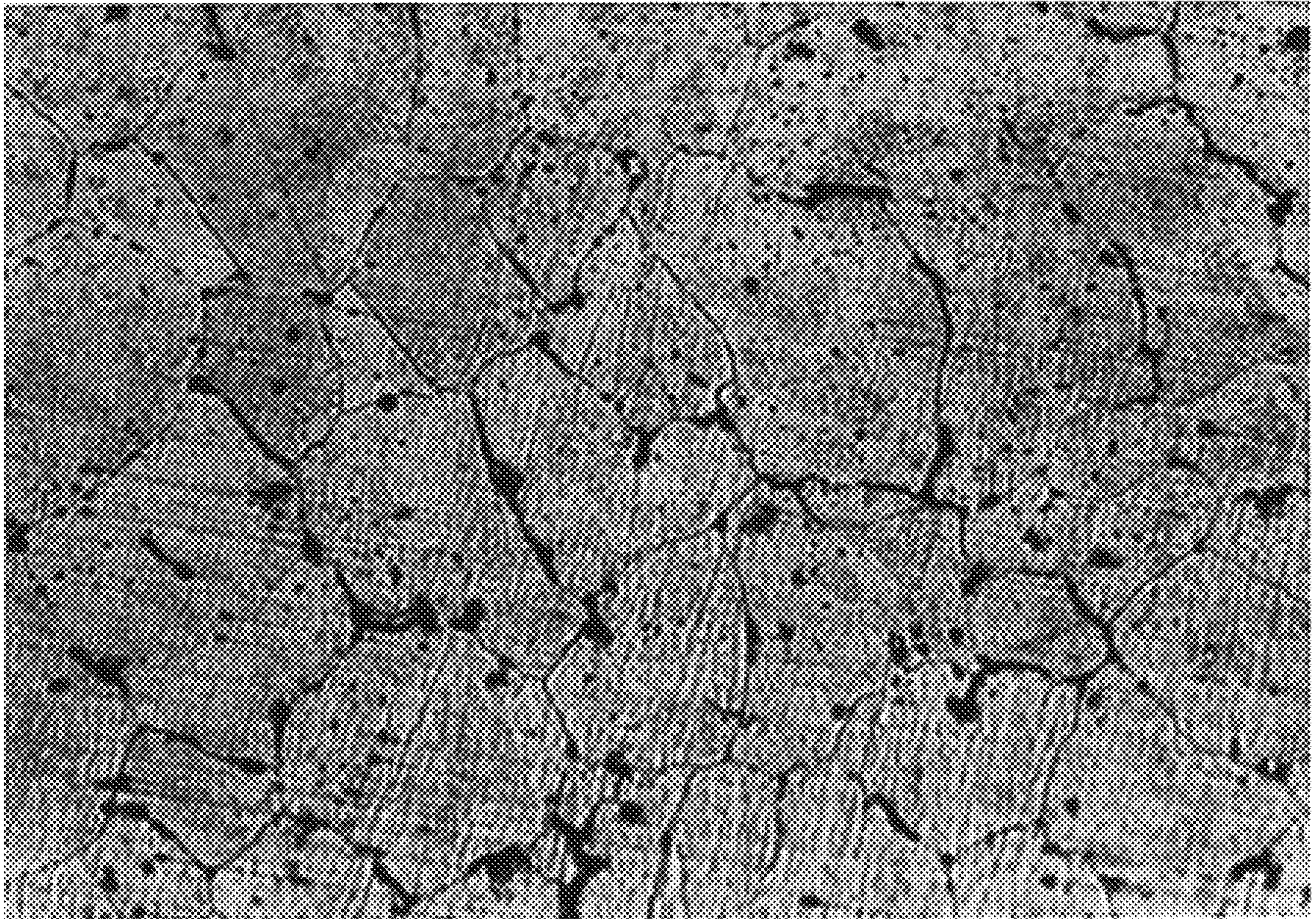
200X CENTRIFUGAL CAST AND HIPPED JC6061-T6C
