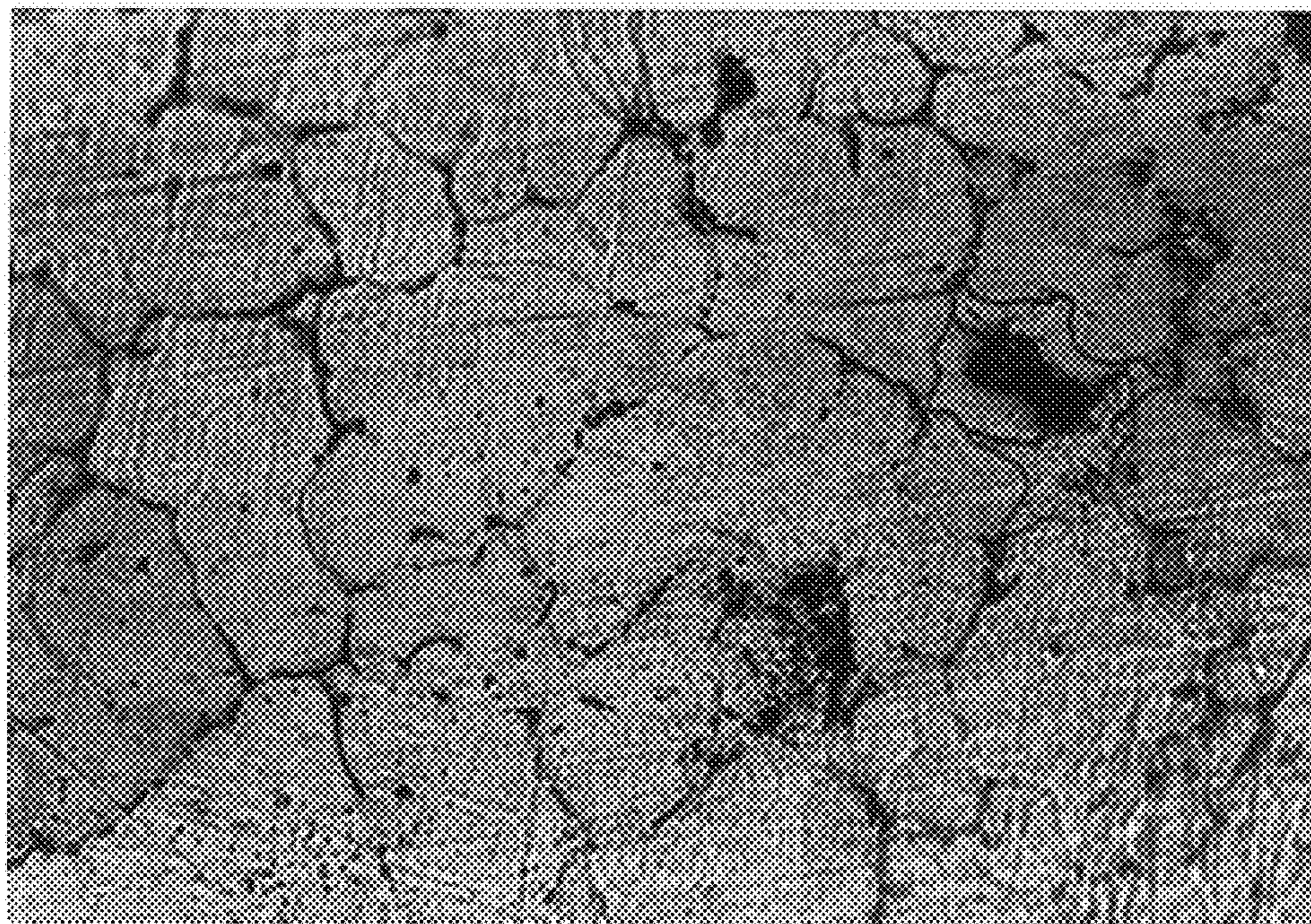
200X UNHIPPED CENTRIFUGAL CAST JC6061-T6C
