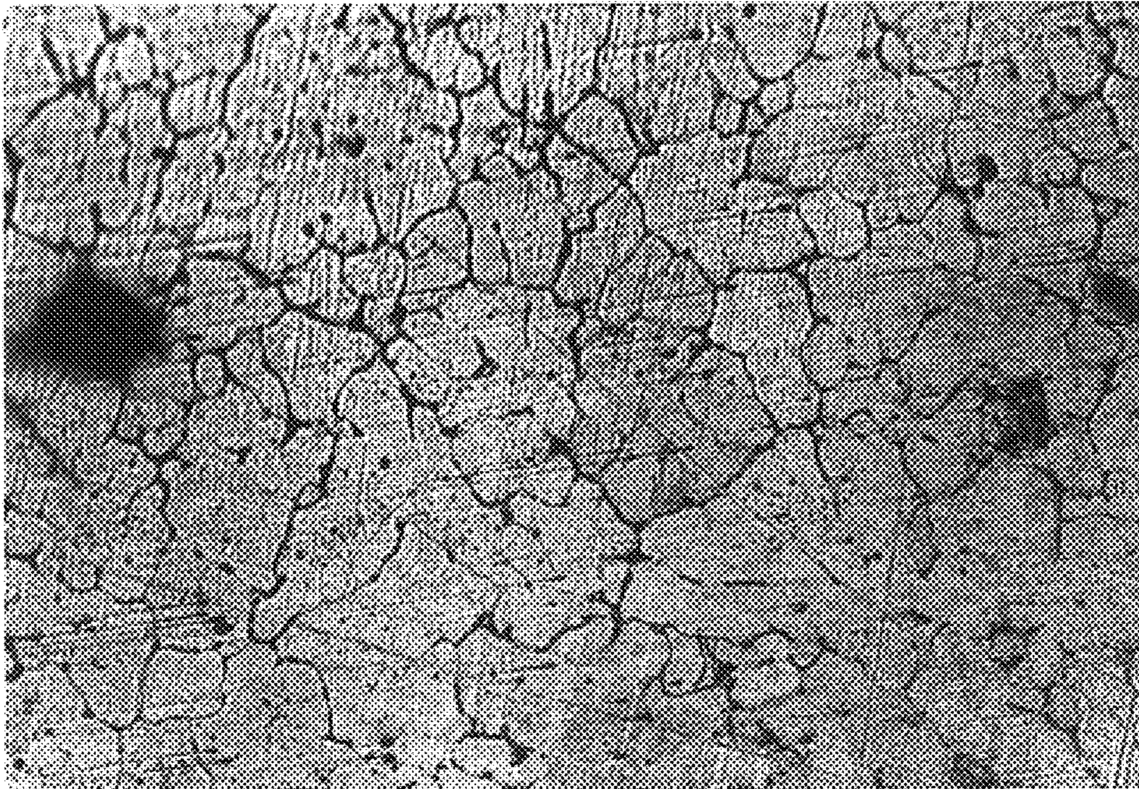
100X UNHIPPED CENTRIFUGAL CAST JC6061-T6C
