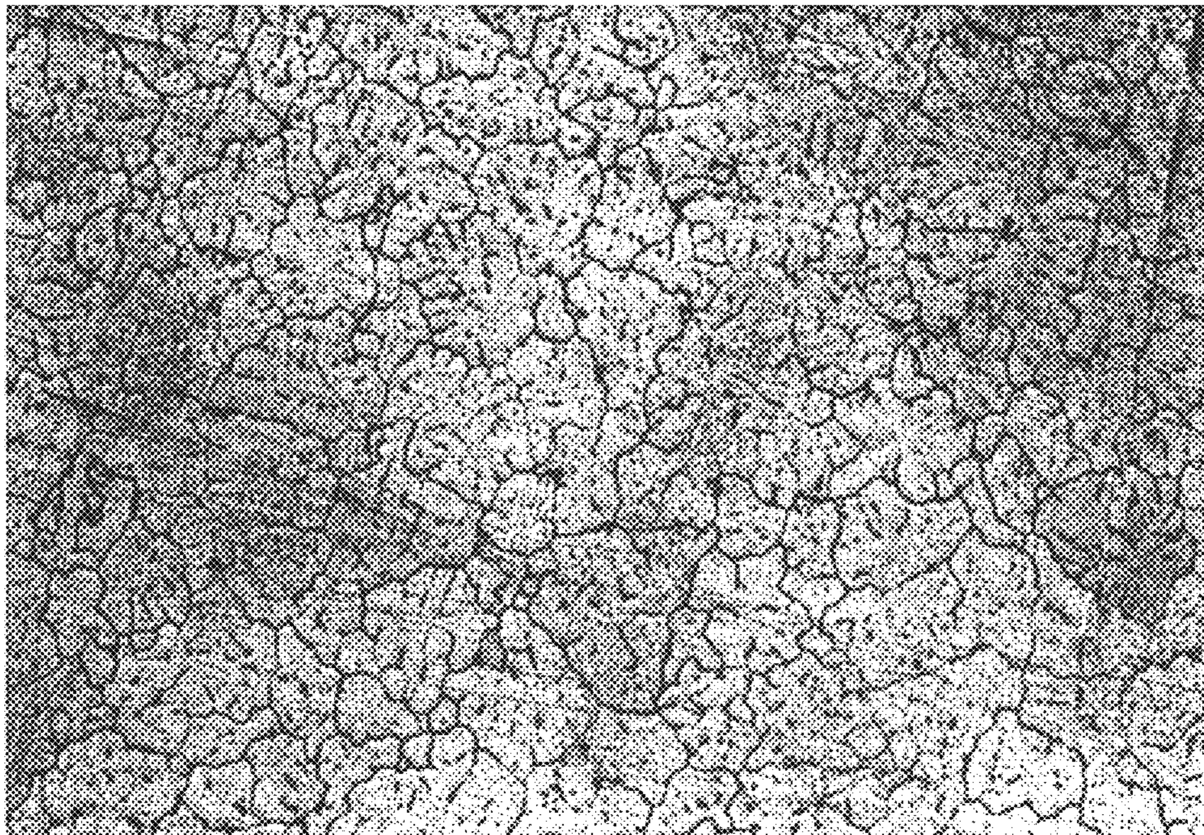
50X CENTRIFUGAL CAST AND HIPPED JC6061-T6C
