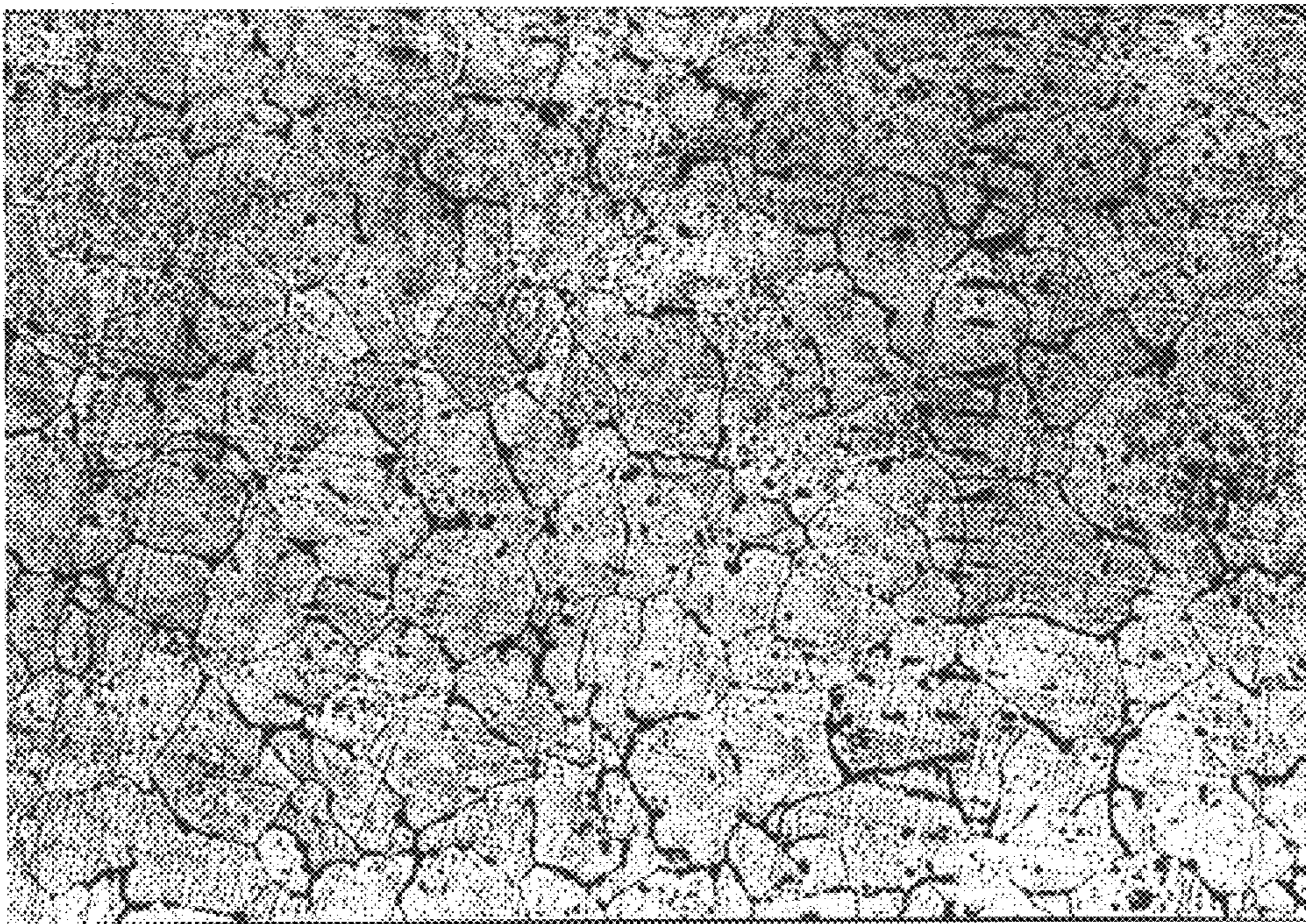
100X CENTRIFUGAL CAST AND HIPPED JC6061-T6C
