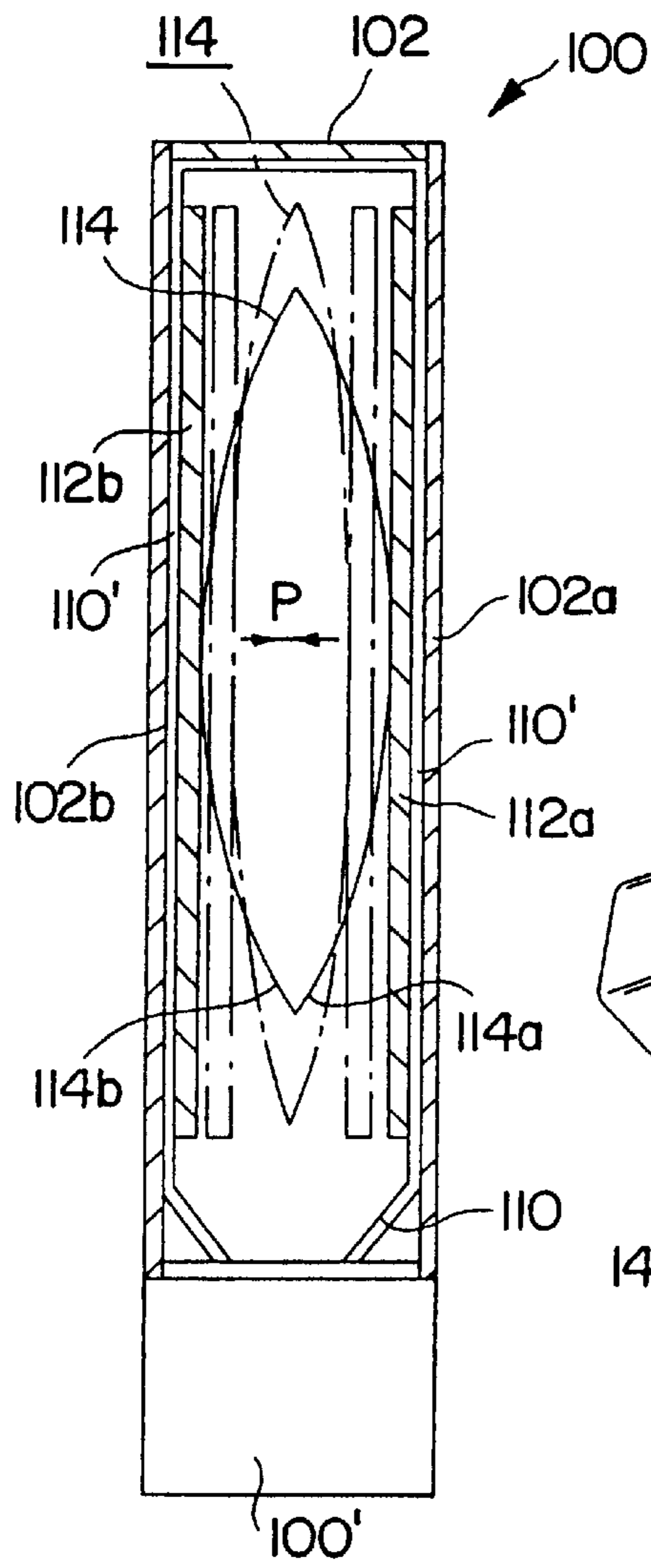
FIG. 9 PRIOR ART
