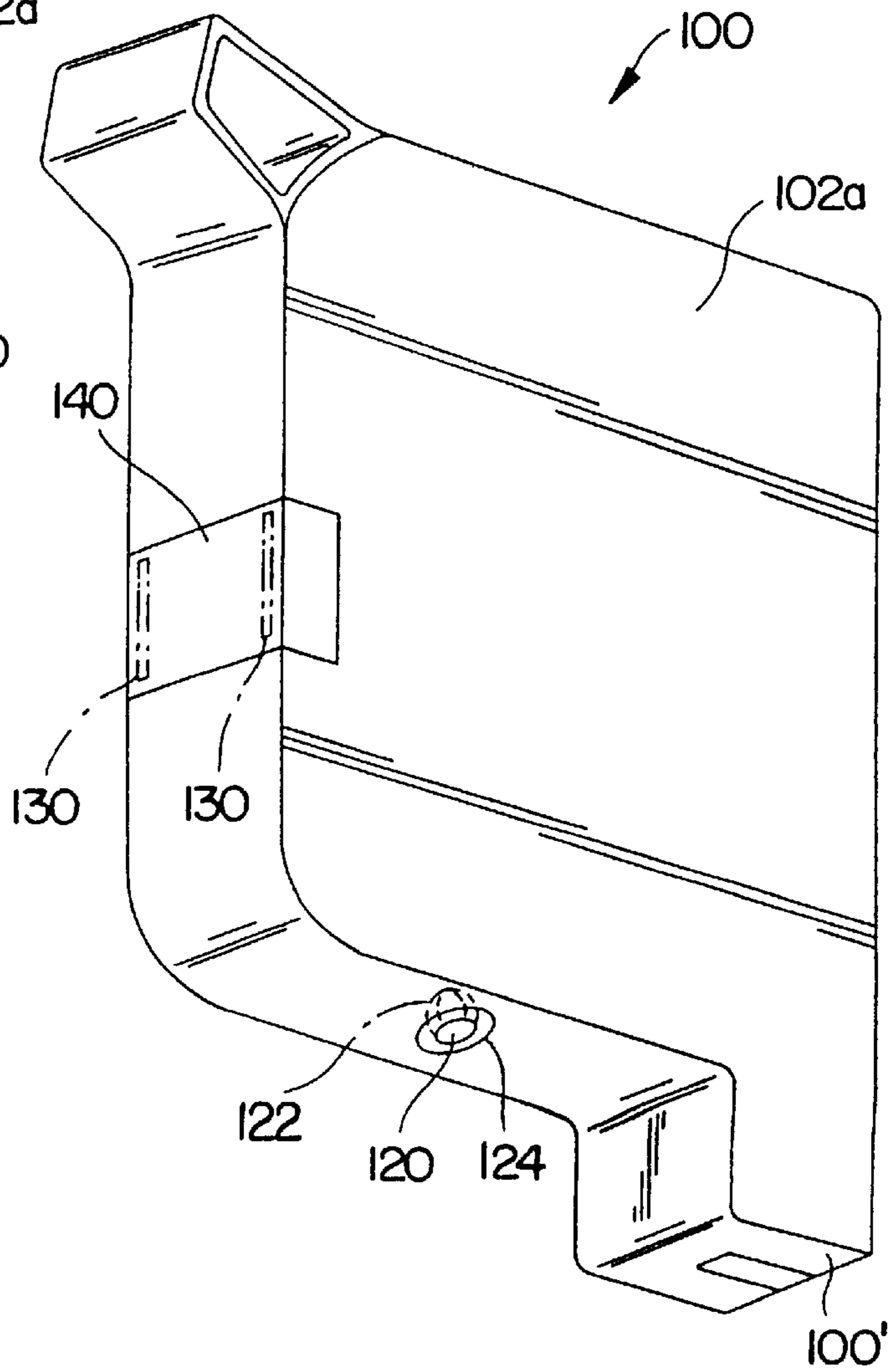
FIG. 10 PRIOR ART
