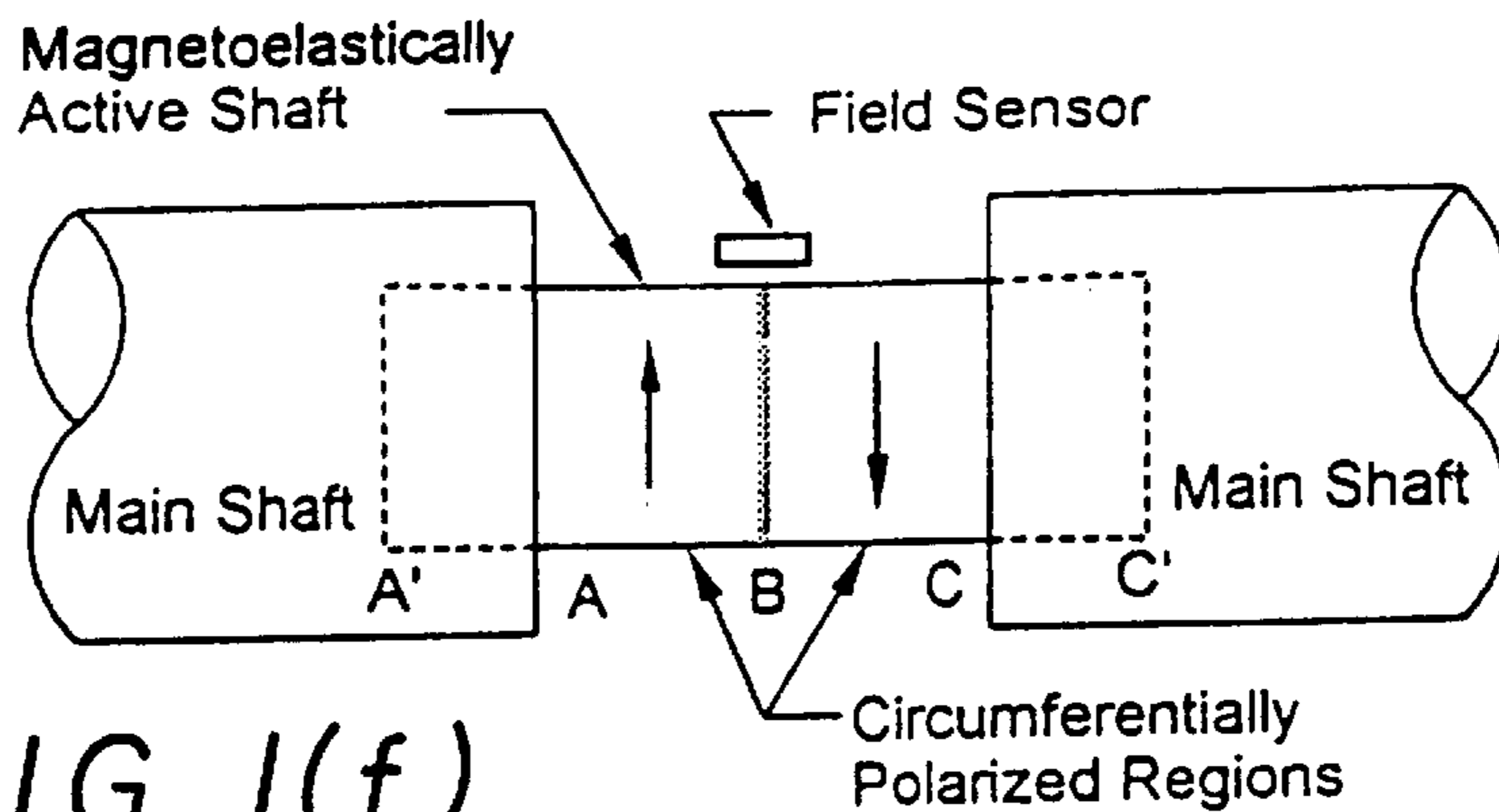
FIG. 1(e) Circumferentially Polarized Regions
