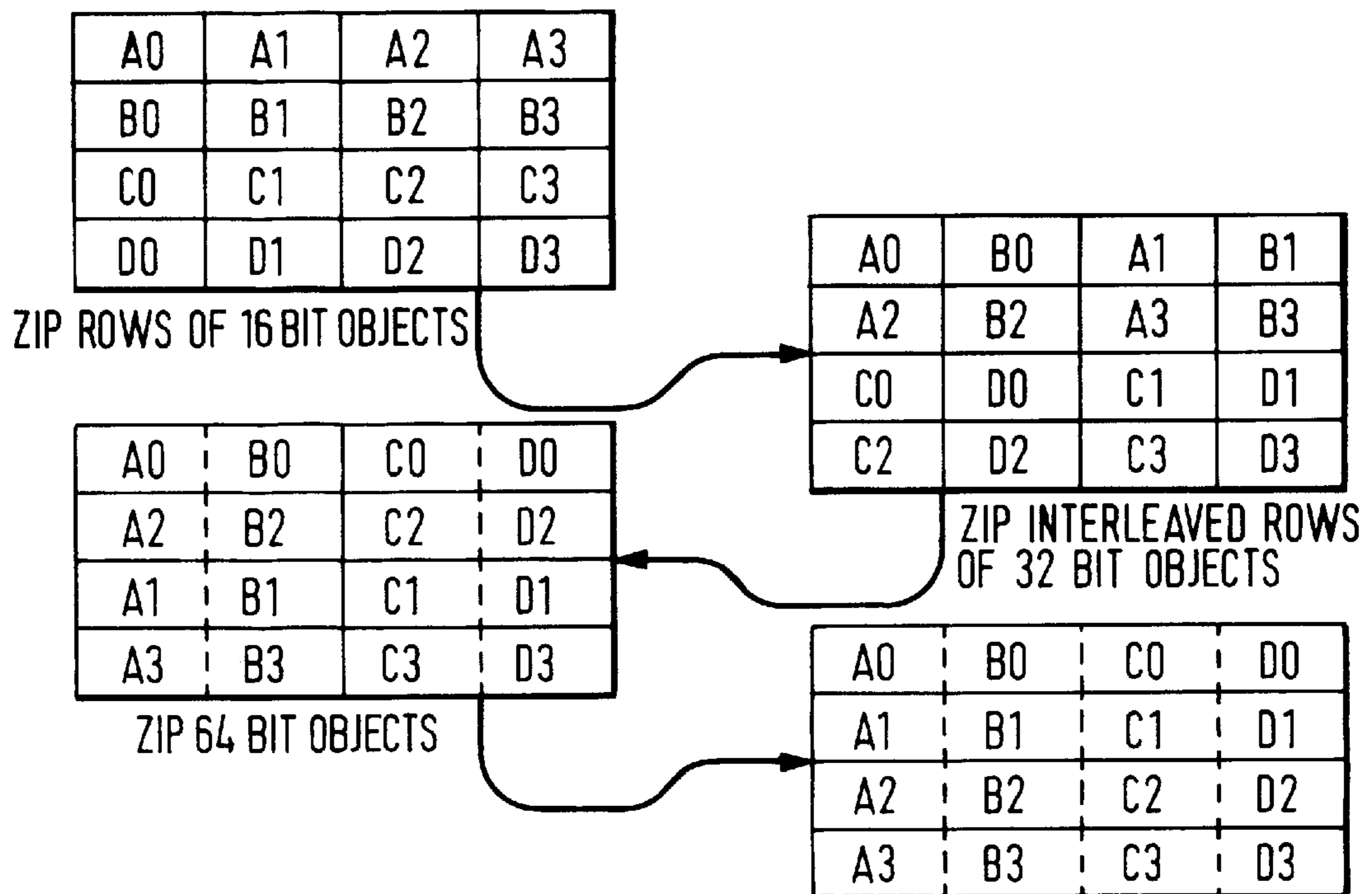
FIG. 15 4 BY 4 MATRIX TRANSPOSE USING ZIPS
