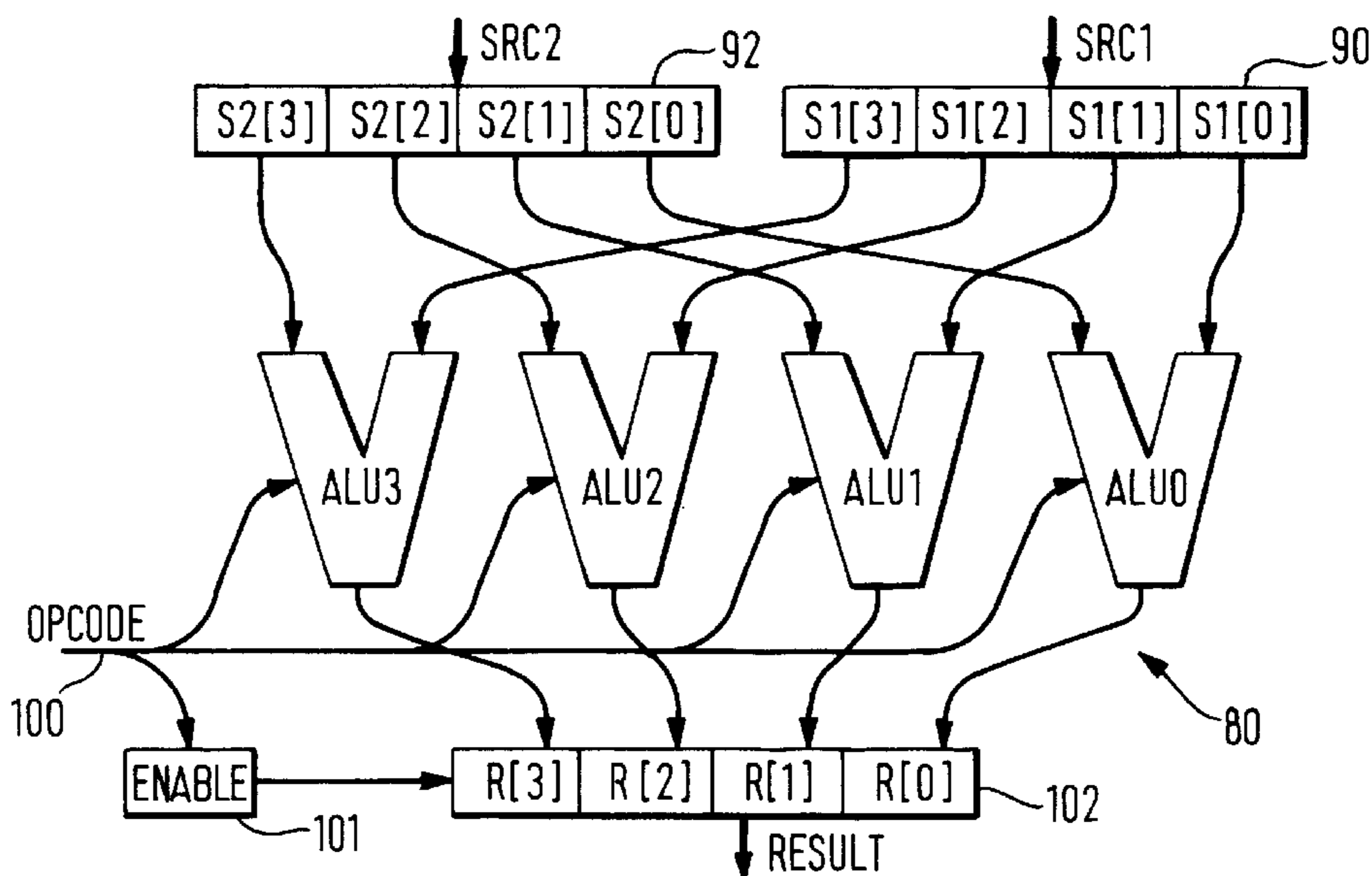
OBVIOUS PACKED ARITHMETIC
