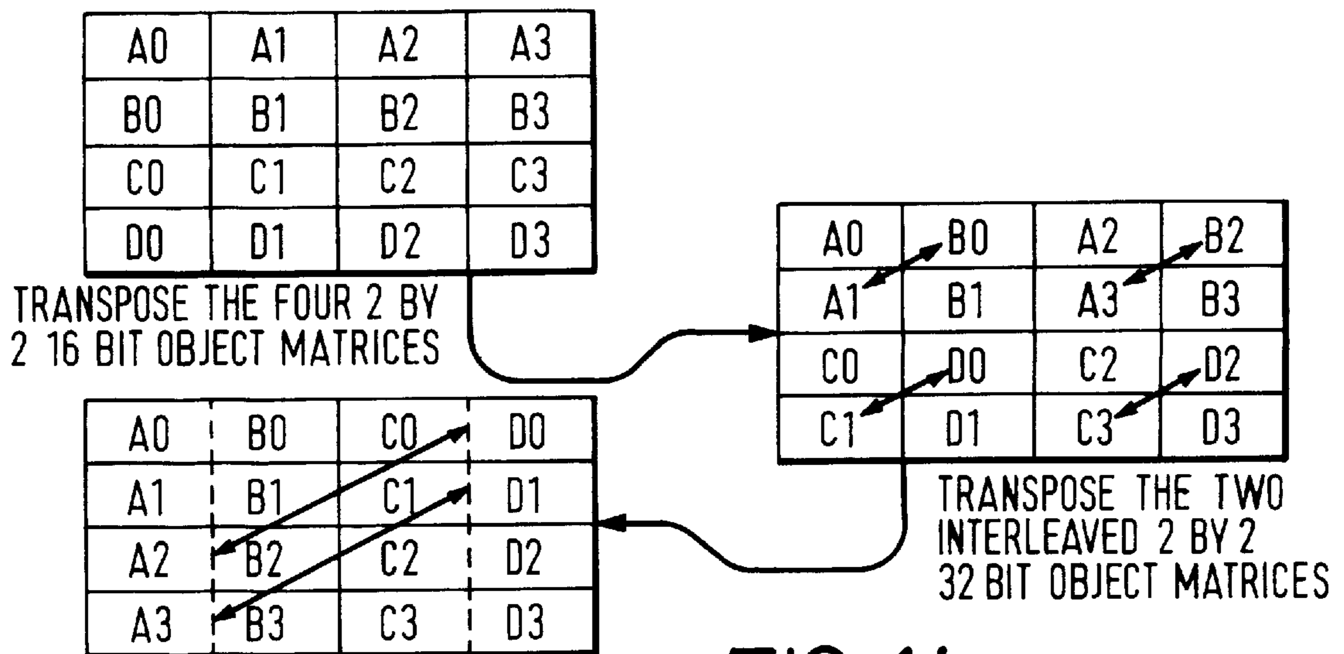
FIG. 14 4 BY 4 MATRIX TRANSPOSE USING FLIPS
