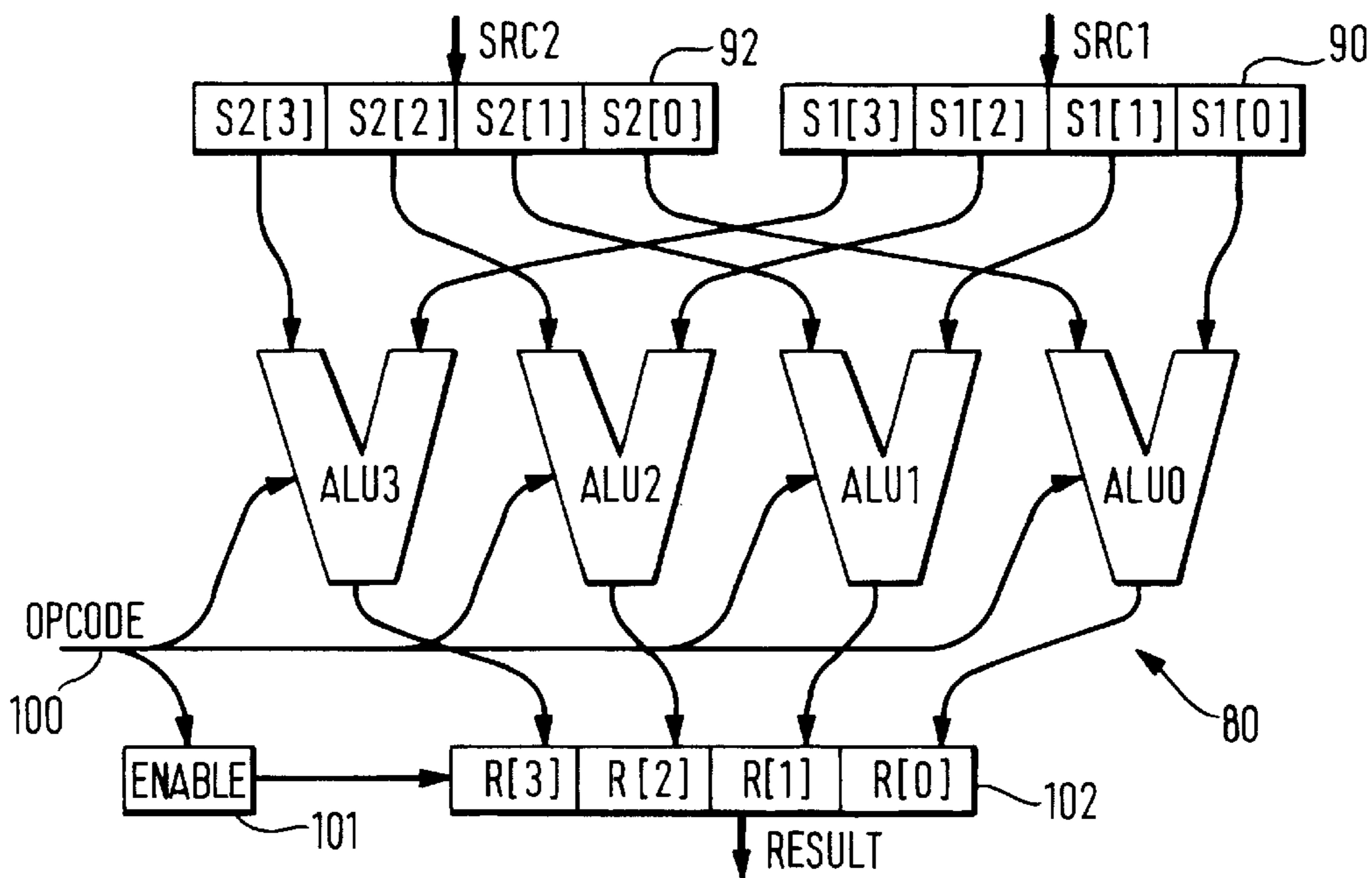
FIG. 4 OBVIOUS PACKED ARITHMETIC
