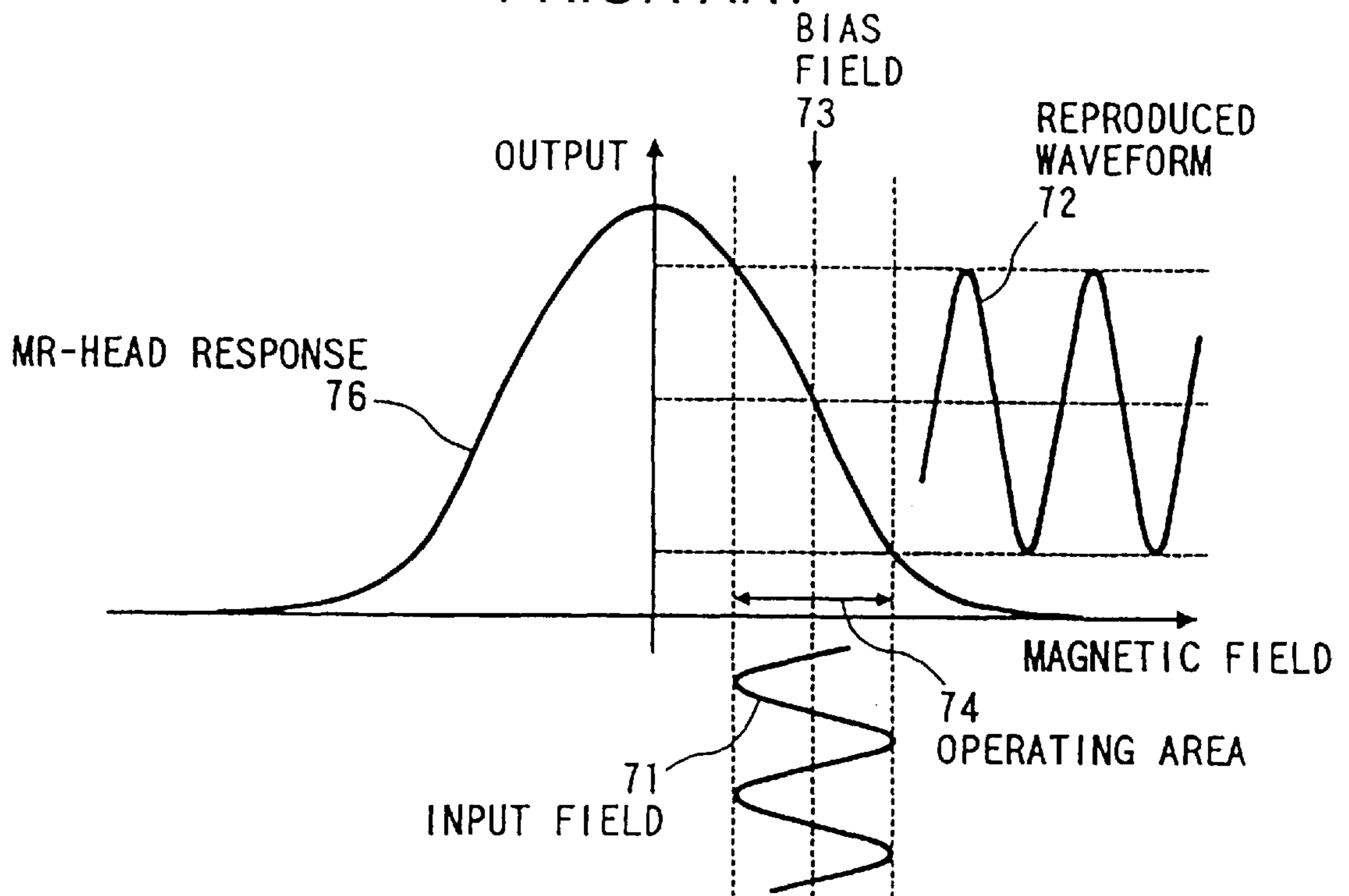
FIG. 11 PRIOR ART
