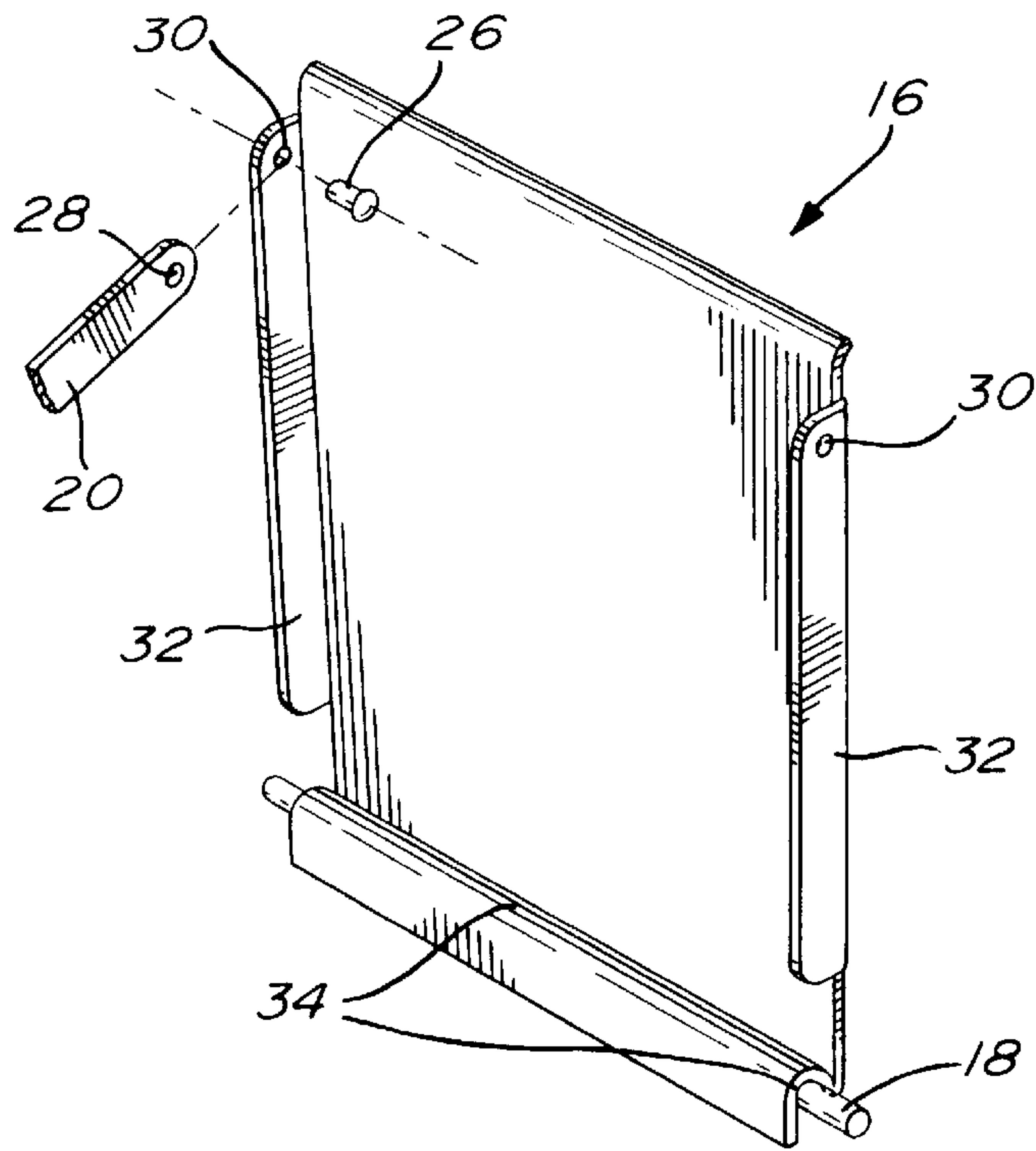
FIG. 3 (PRIOR ART)
