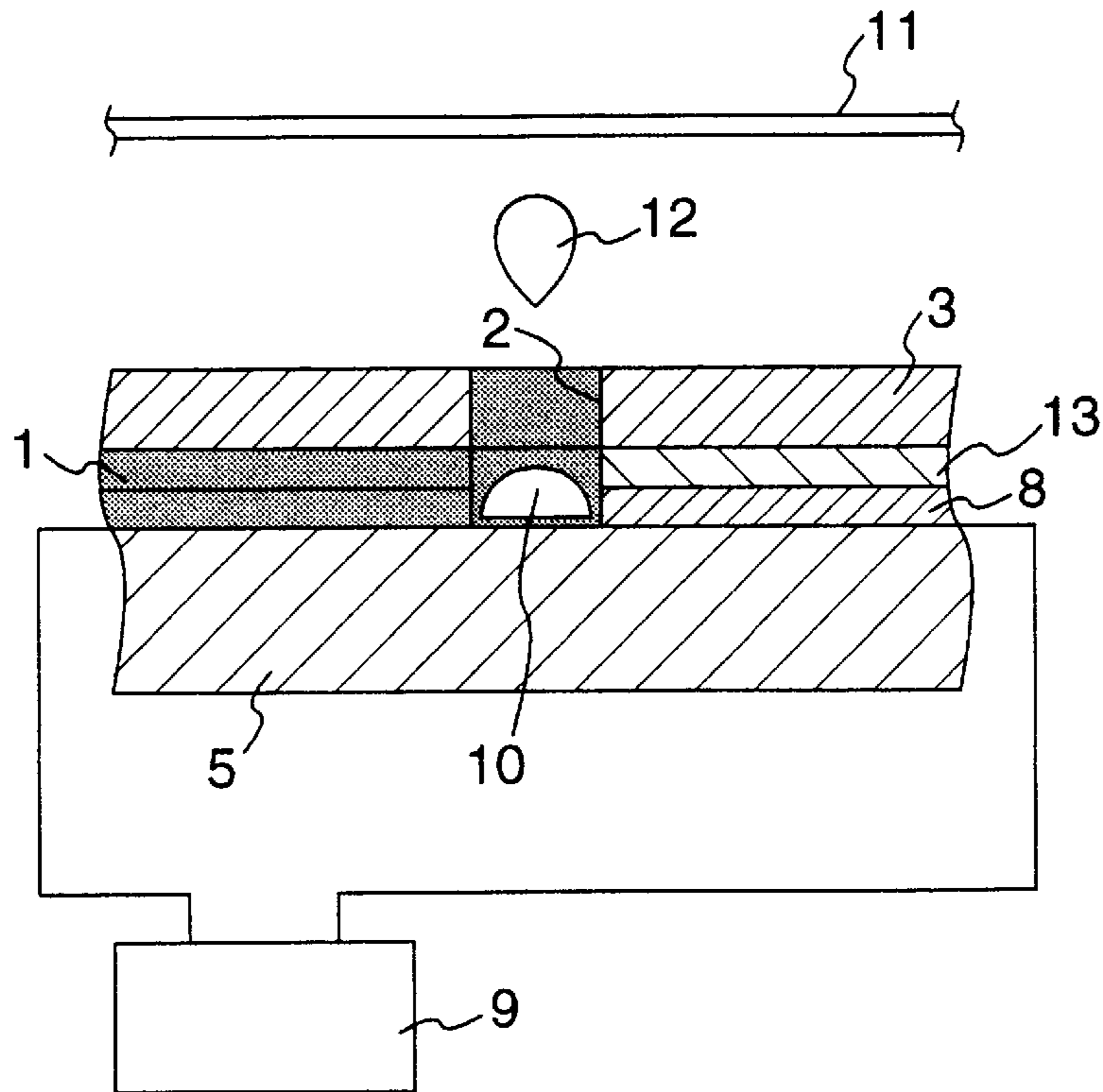
FIG. 4 PRIOR ART
