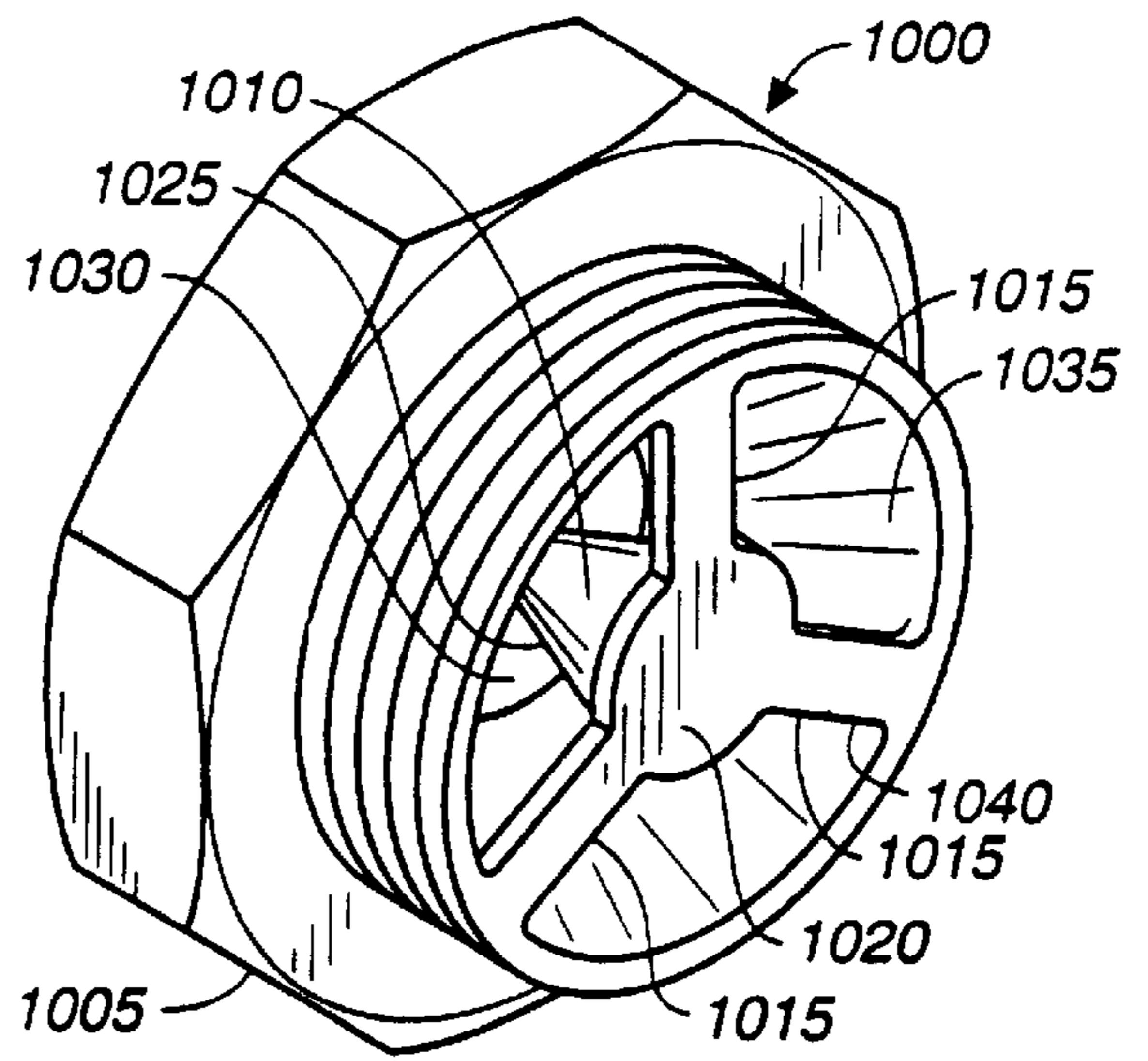
FIG. 10 (PRIOR ART)
