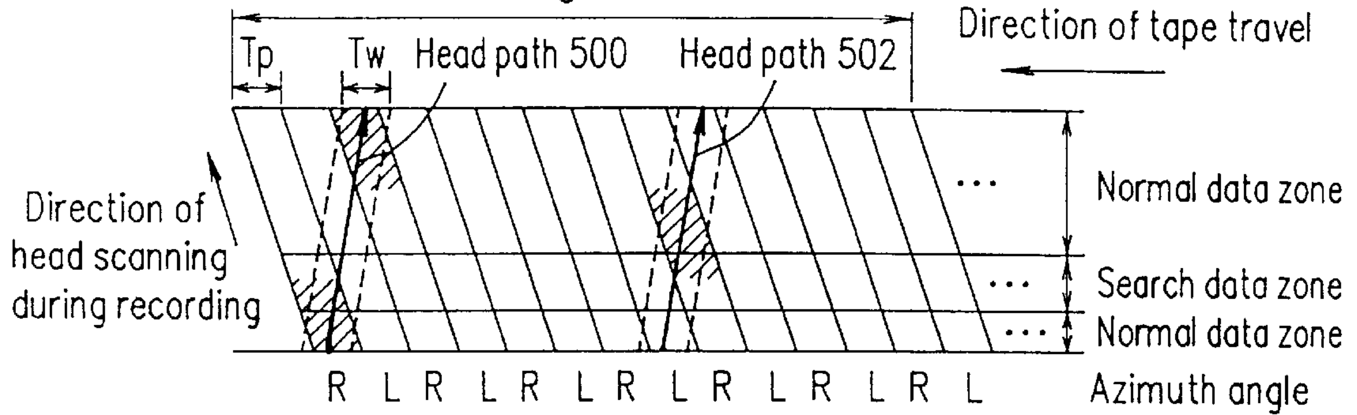
FIG. 5A Track pattern ( T_w = T_p )
