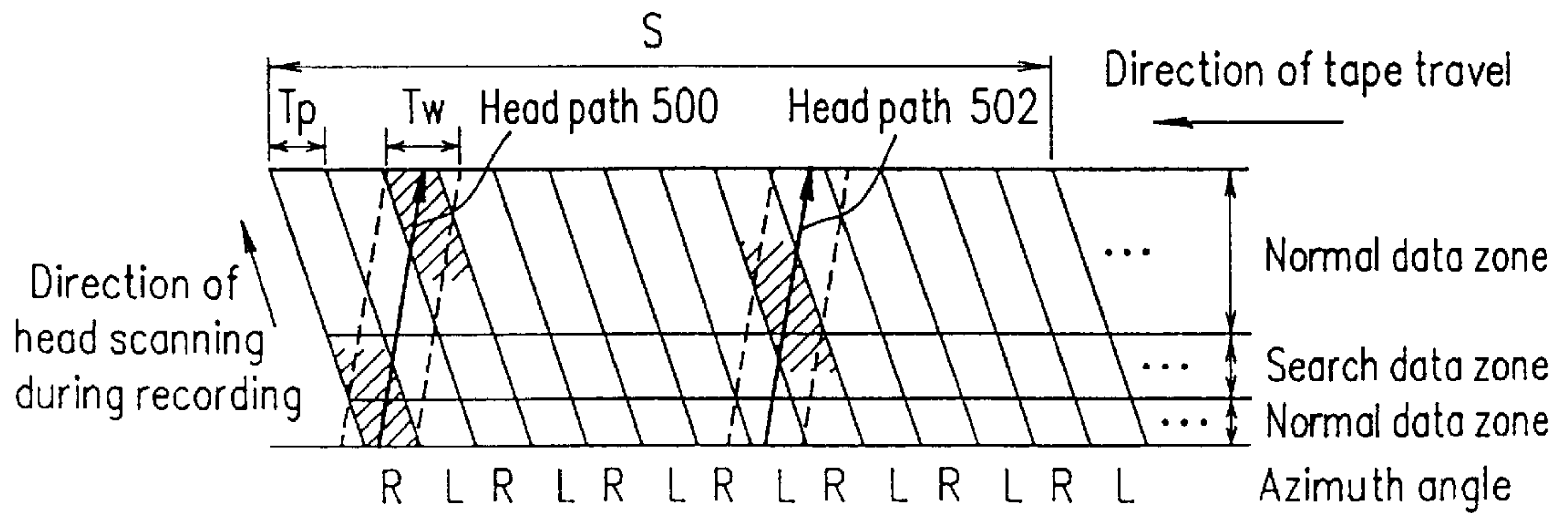
FIG. 5D Search data regions in an enlarged view ( T_w > T_p )
