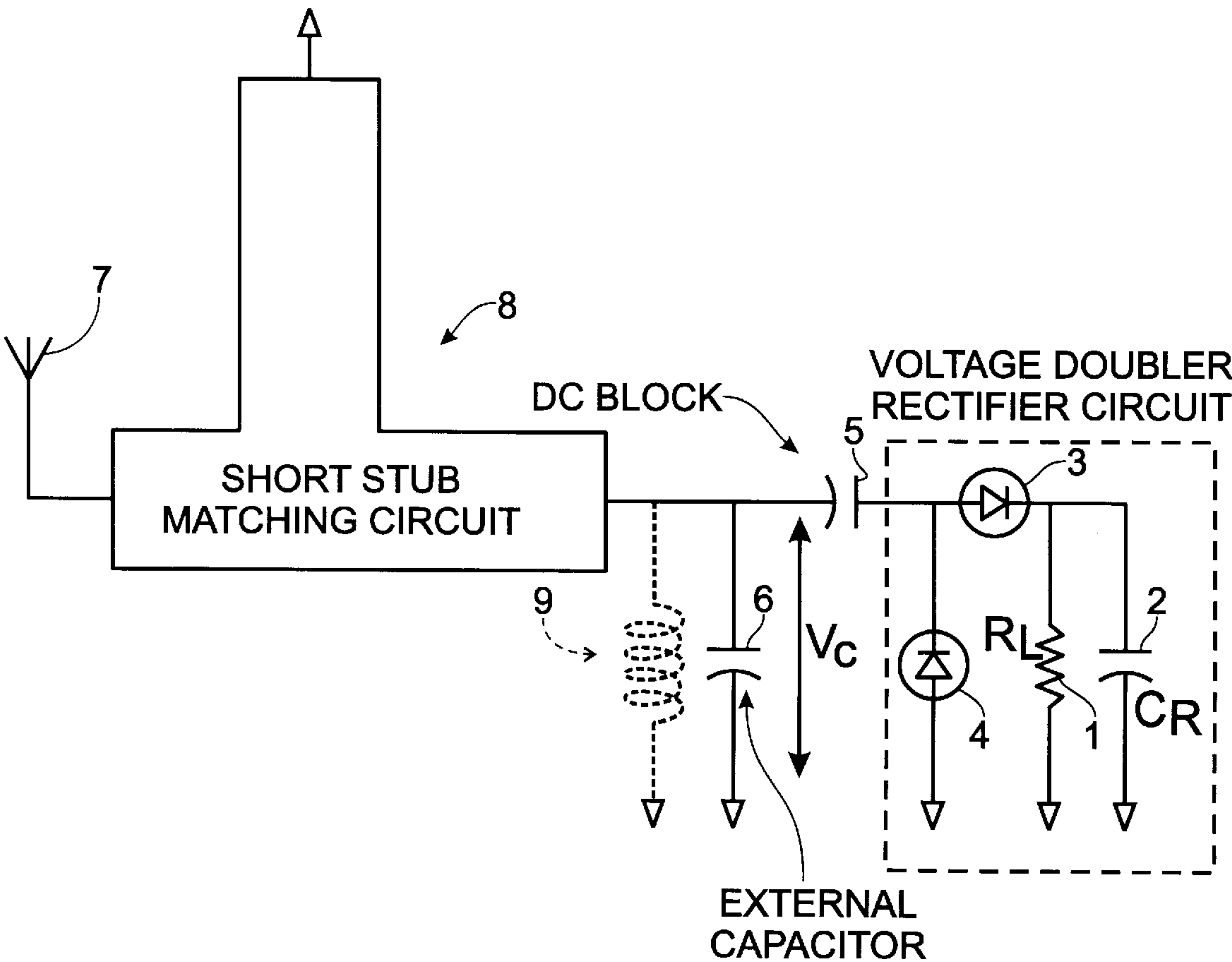
Fig. 3 MICROSTRIP MATCHING RECTENNA CIRCUIT USING EXTERNAL CAPACITOR
