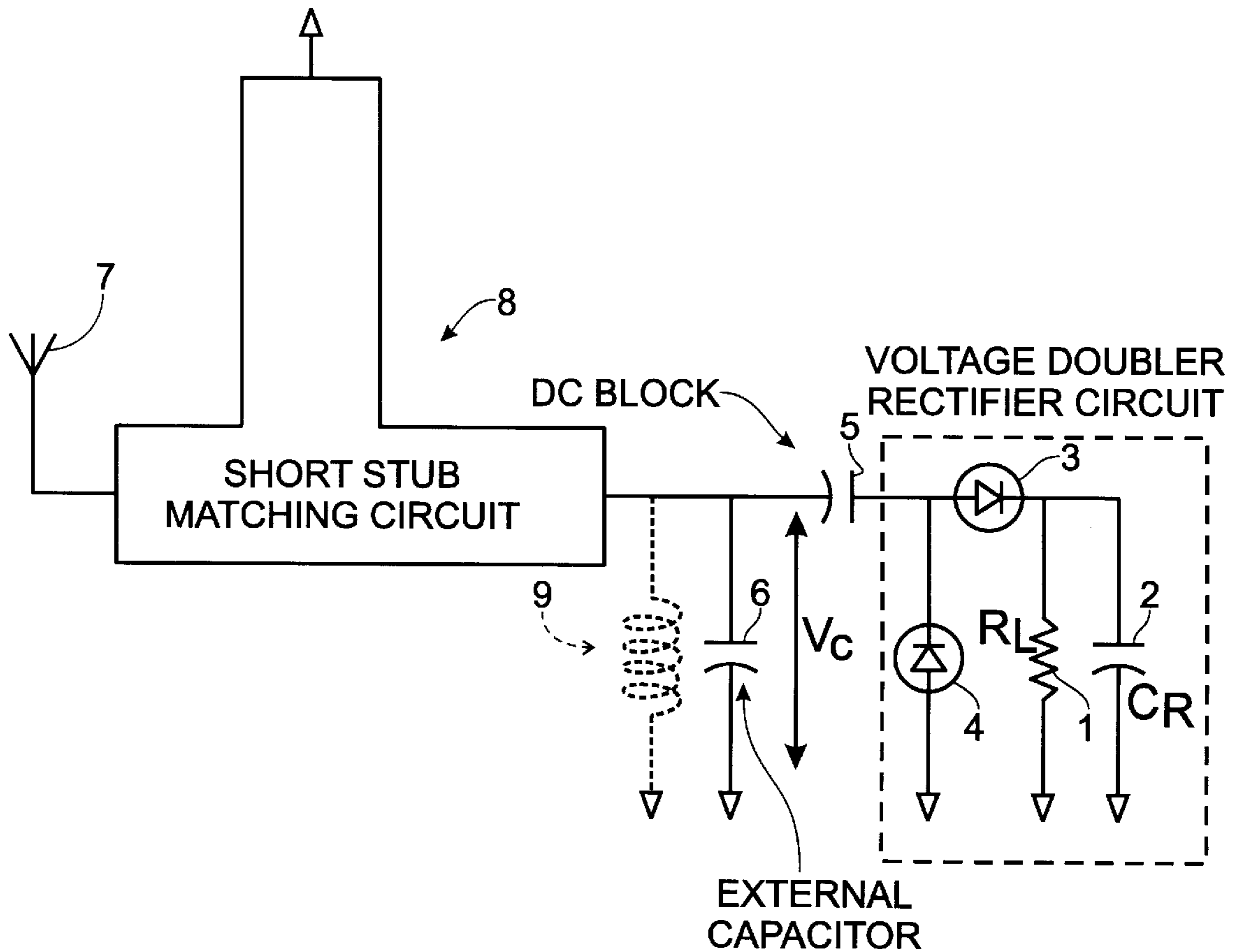
Fig. 3 MICROSTRIP MATCHING RECTENNA CIRCUIT USING EXTERNAL CAPACITOR
