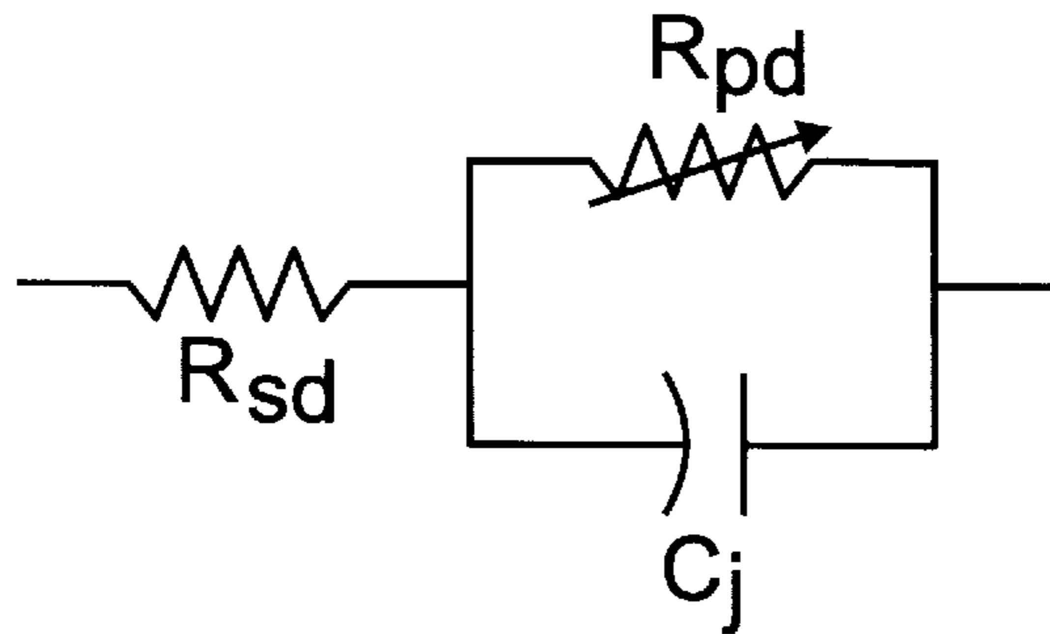
Fig. 1 DIODE EQUIVALENT CIRCUIT
