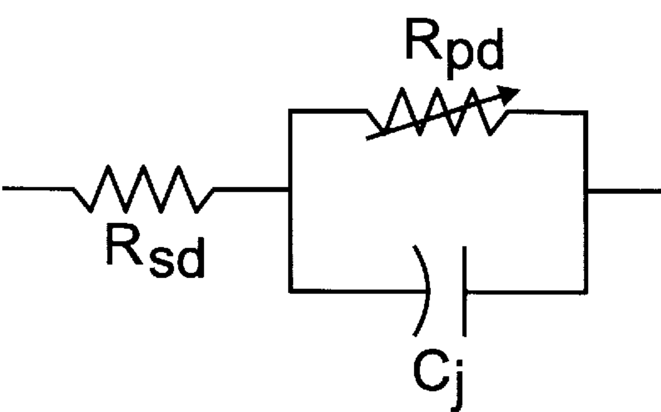
Fig. 1 DIODE EQUIVALENT CIRCUIT
