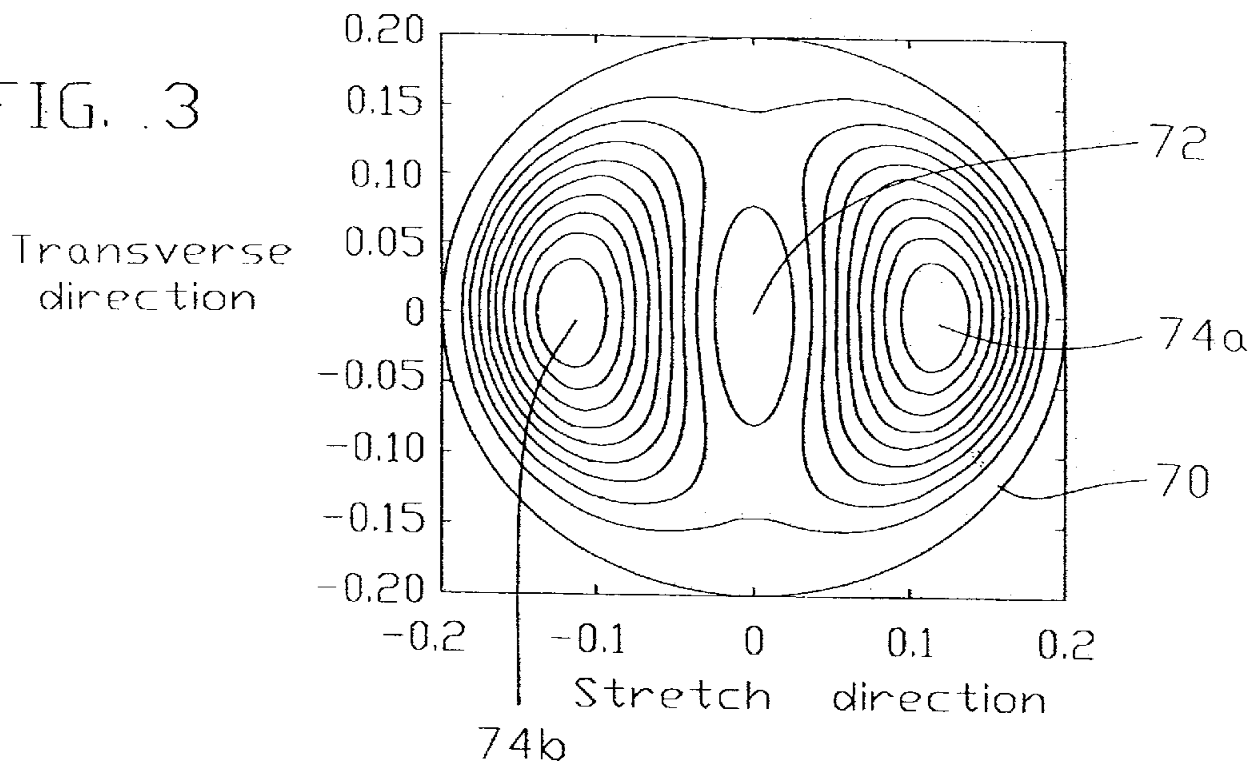
Charge contribution on a PVDF disk
