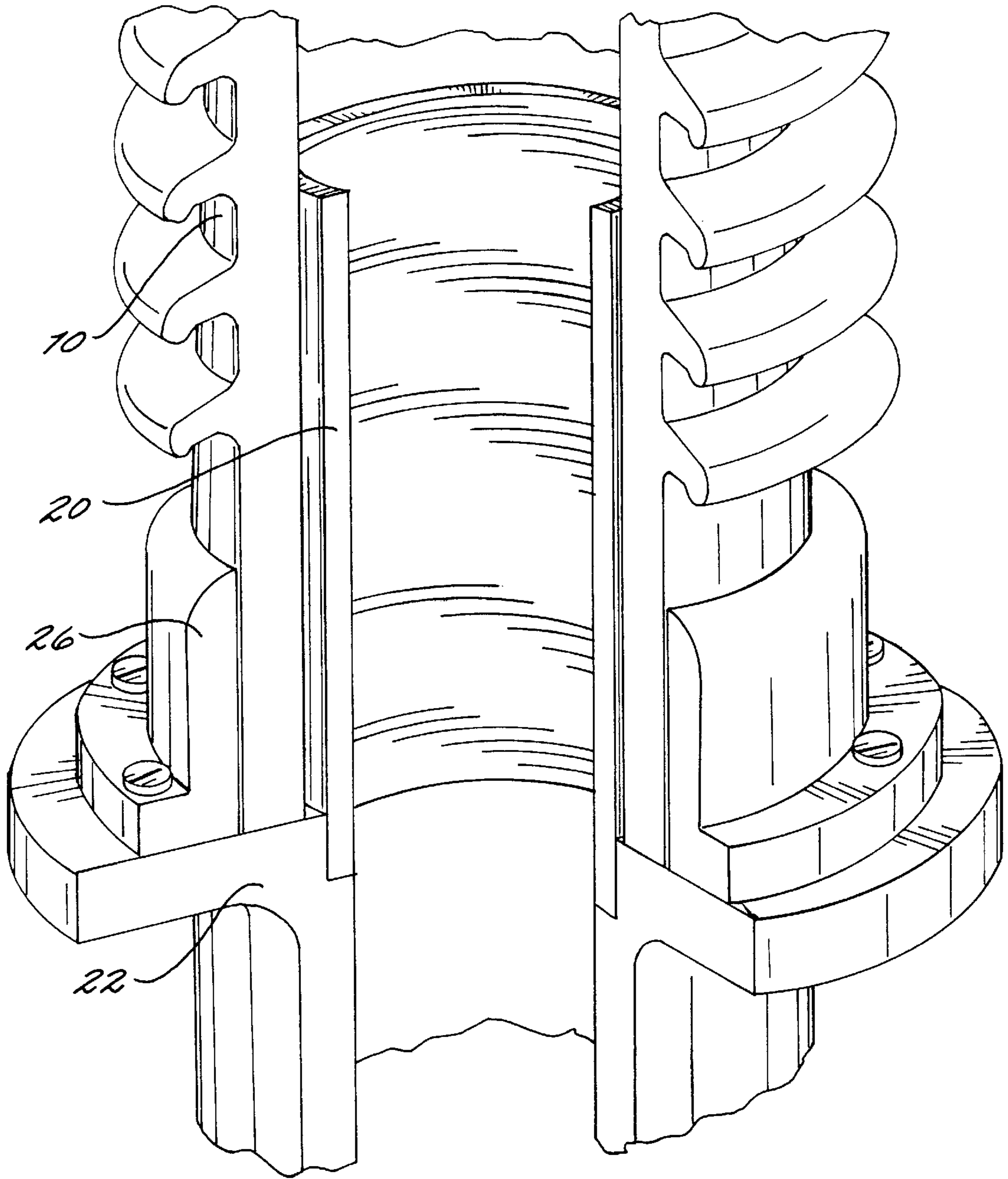
FIG. 2. (PRIOR ART)
