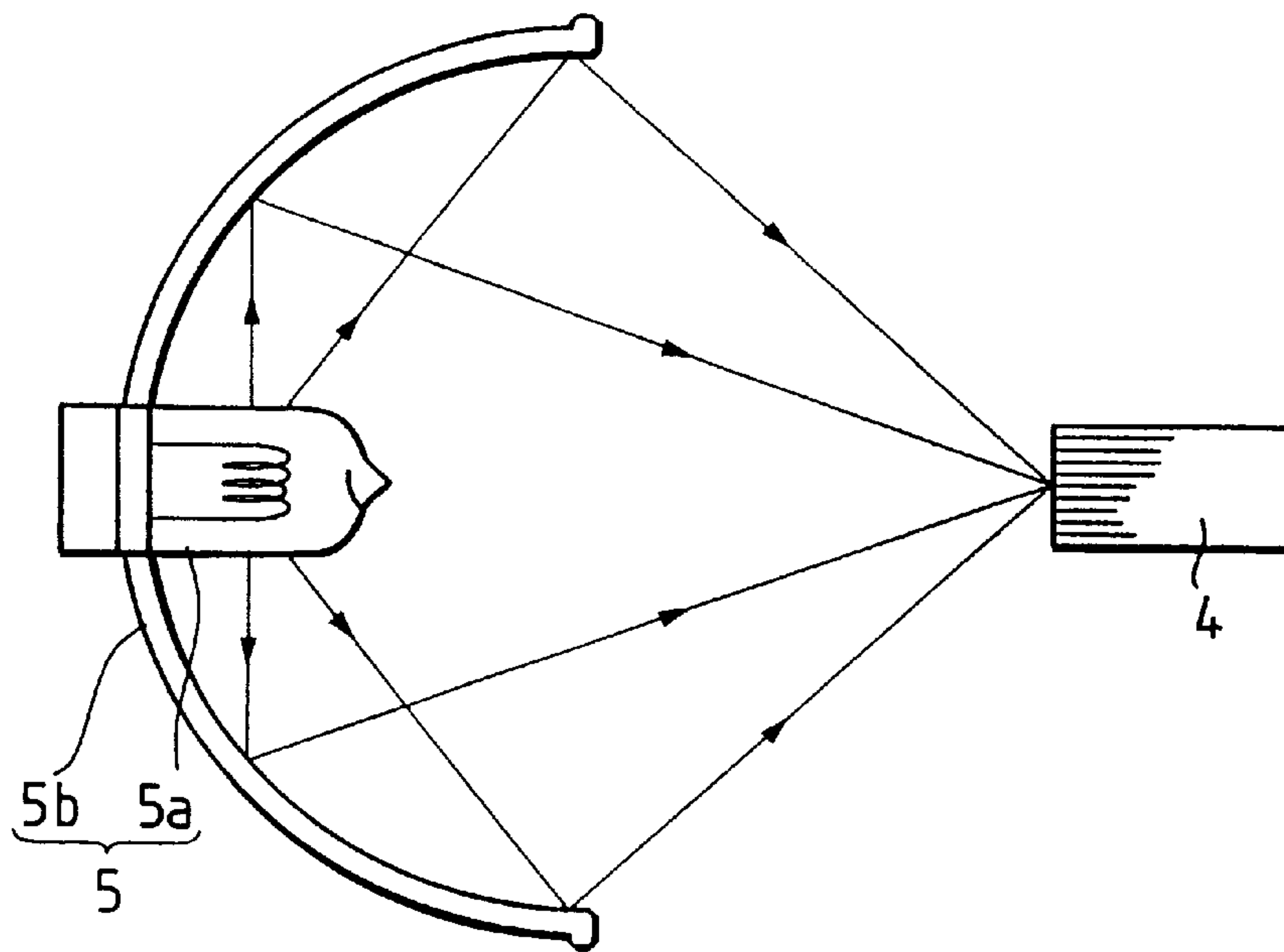
FIG. 2 PRIOR ART
