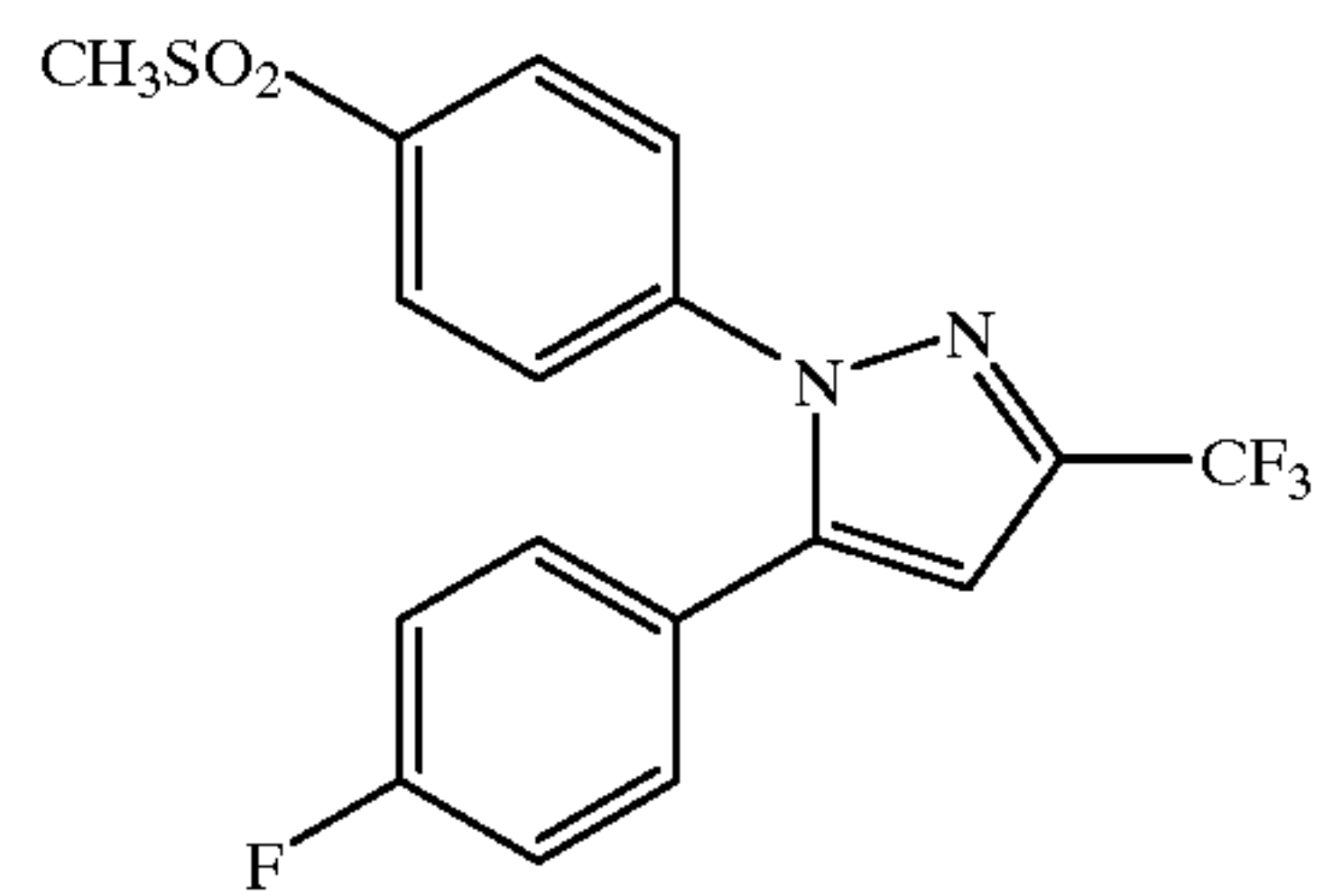
SC-58125
