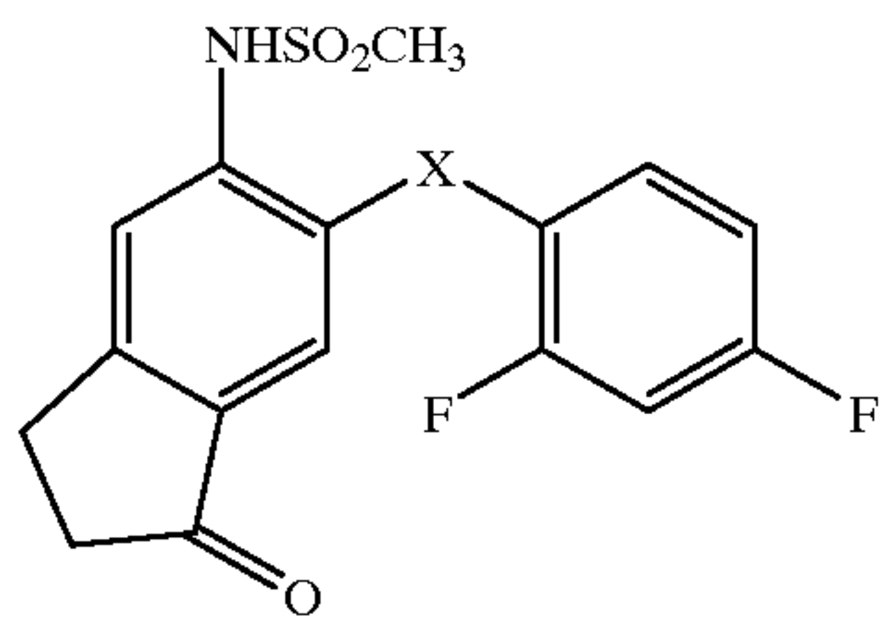
(i), X = S Flosulide, X = O
