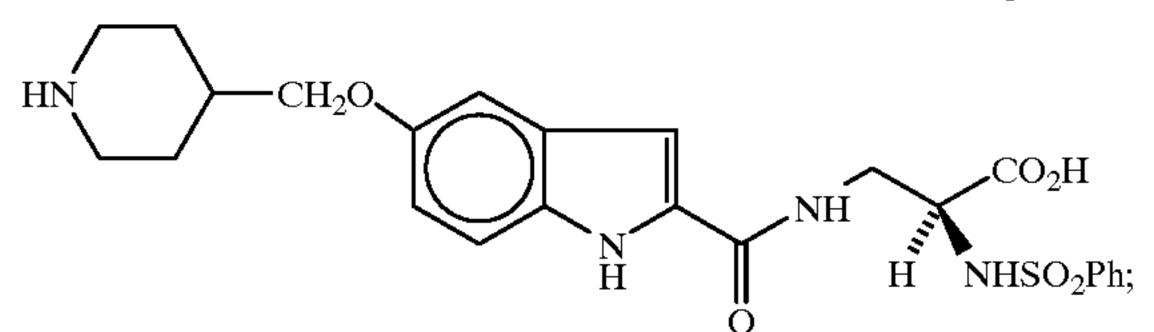
Compound B
