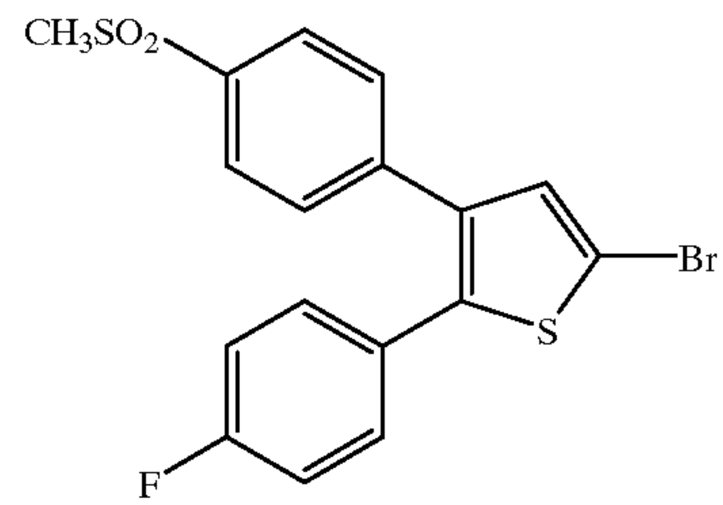
DuP 697
