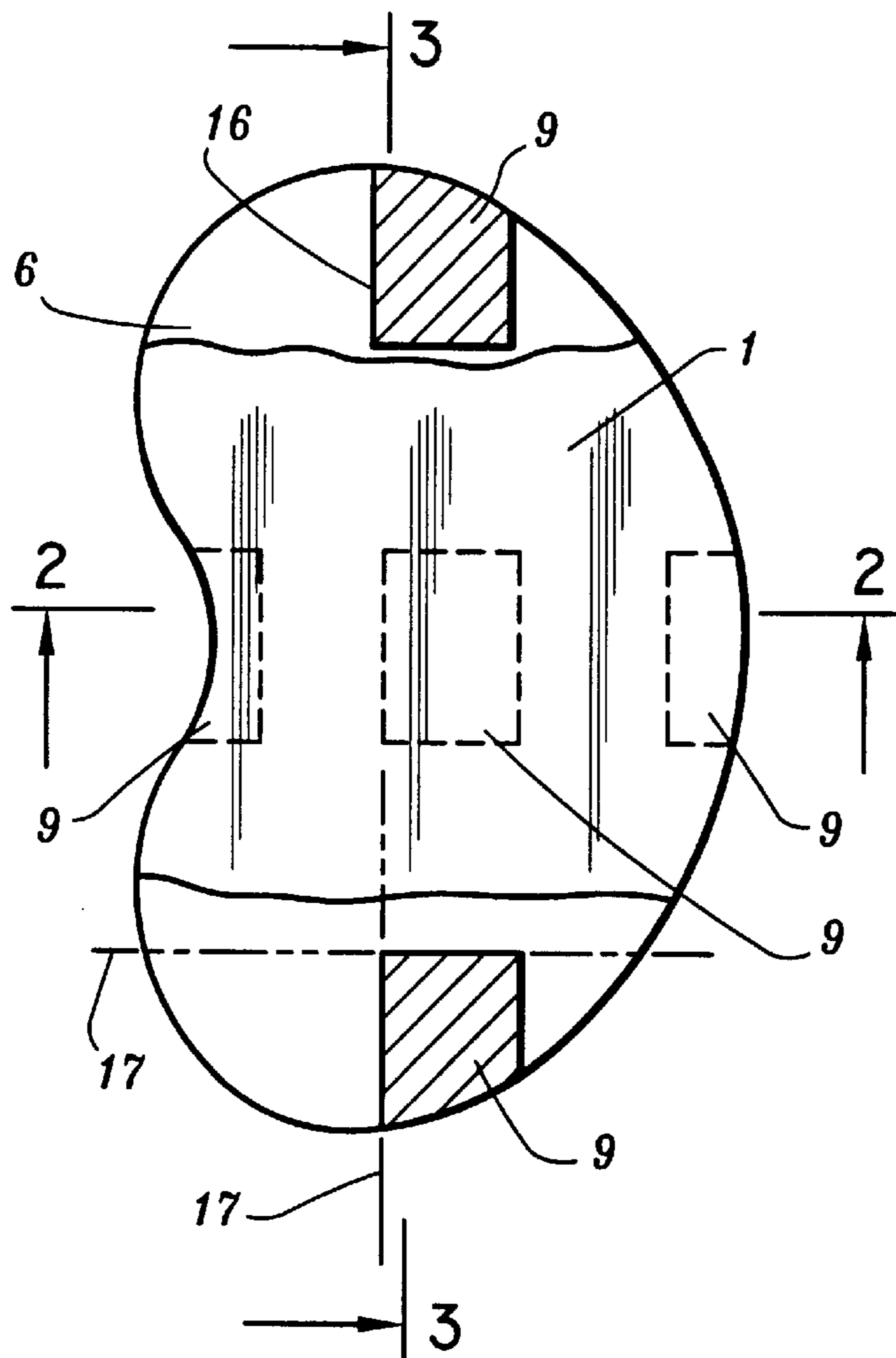
FIG. 1 (PRIOR ART)
