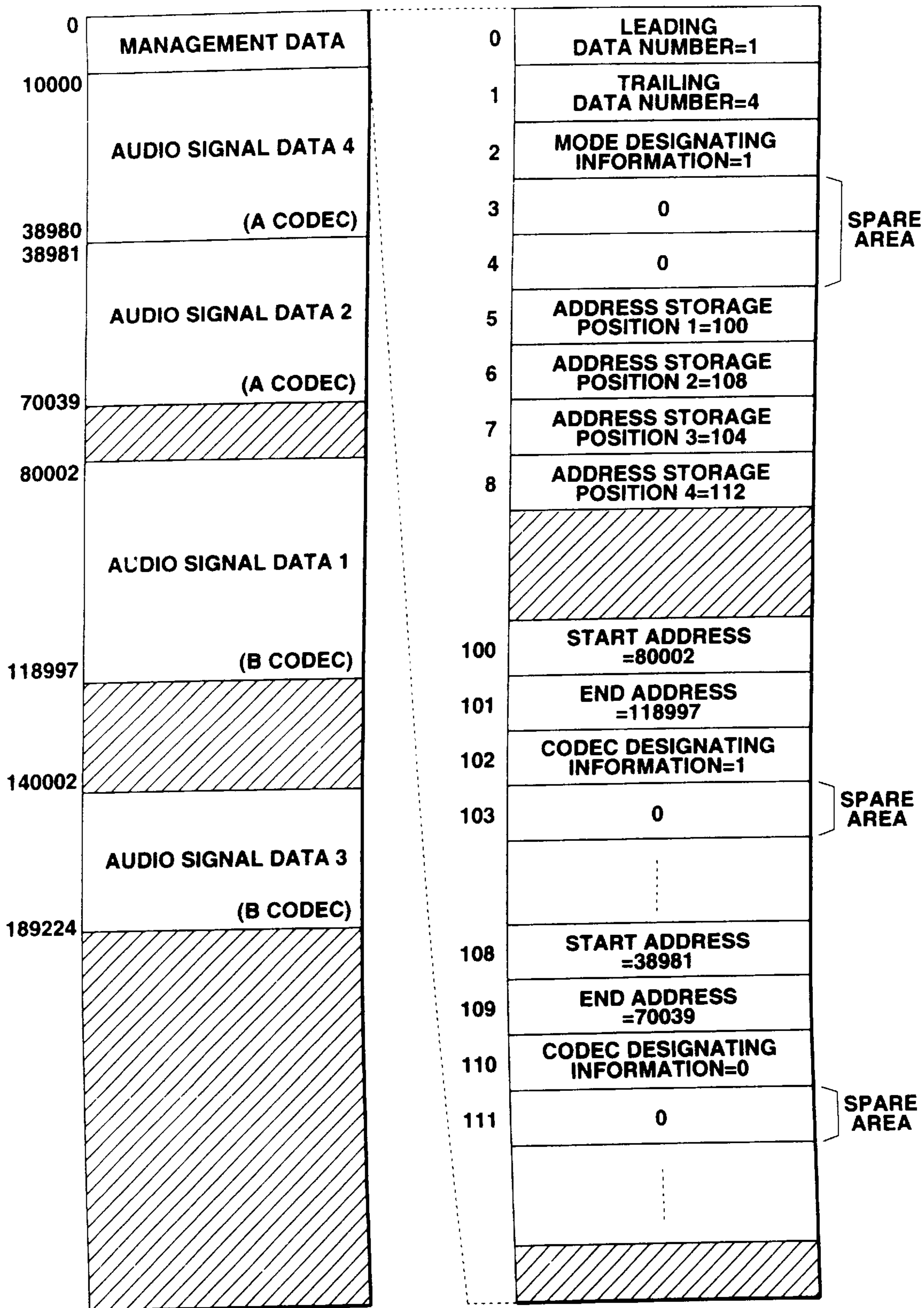
FIG.3 (PRIOR ART)
