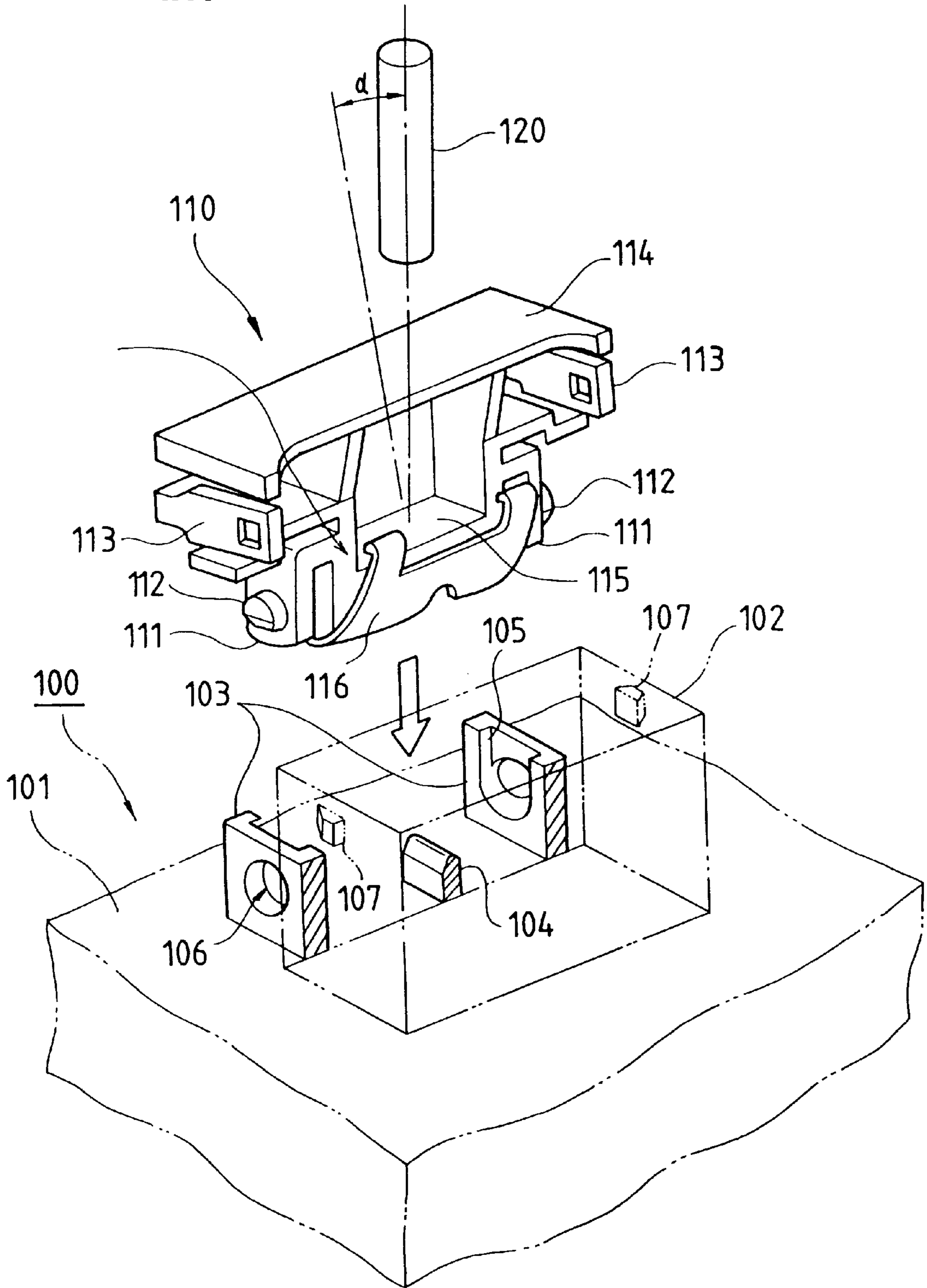
FIG. 7 PRIOR ART
