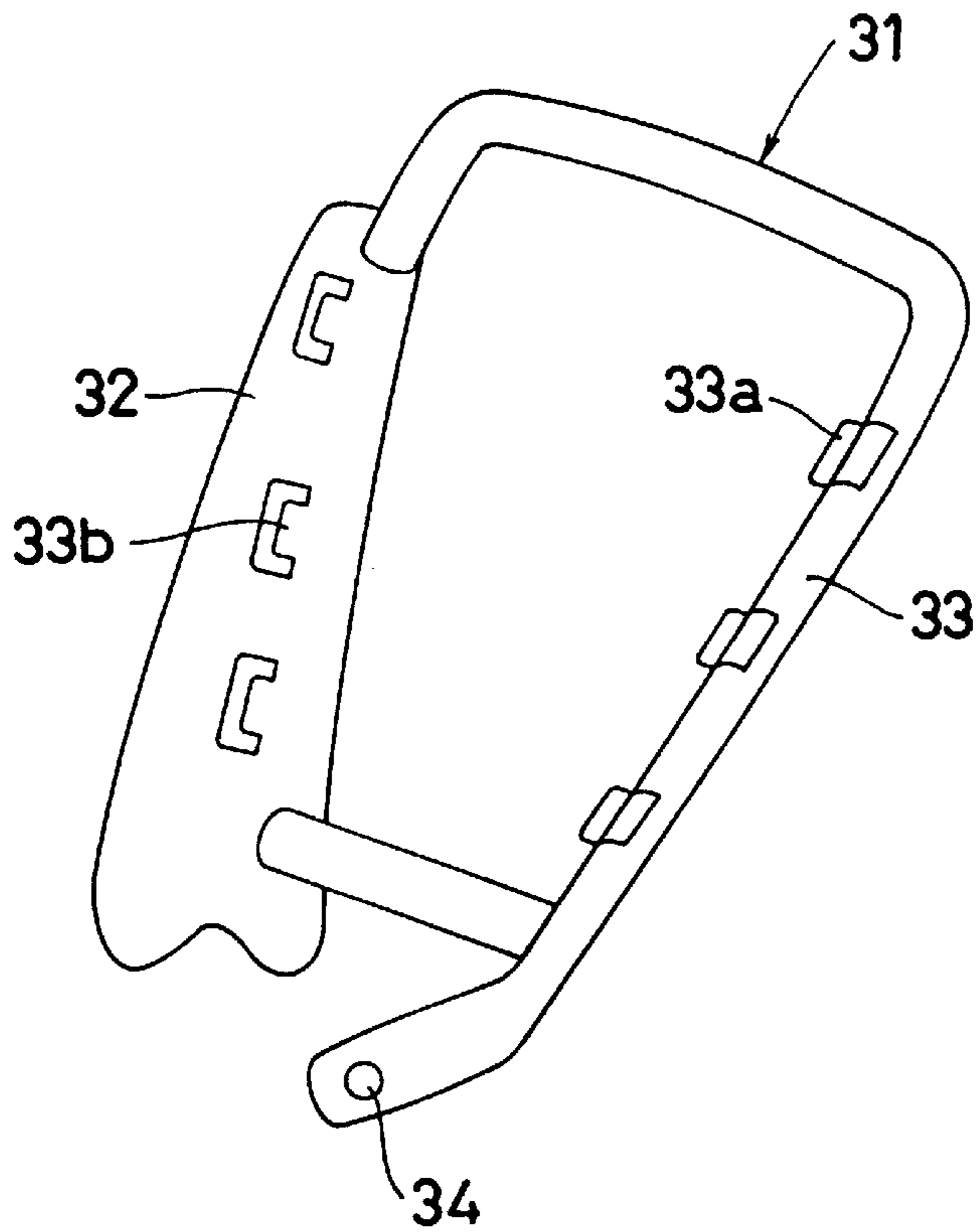
FIG 16 (RELATED ART)
