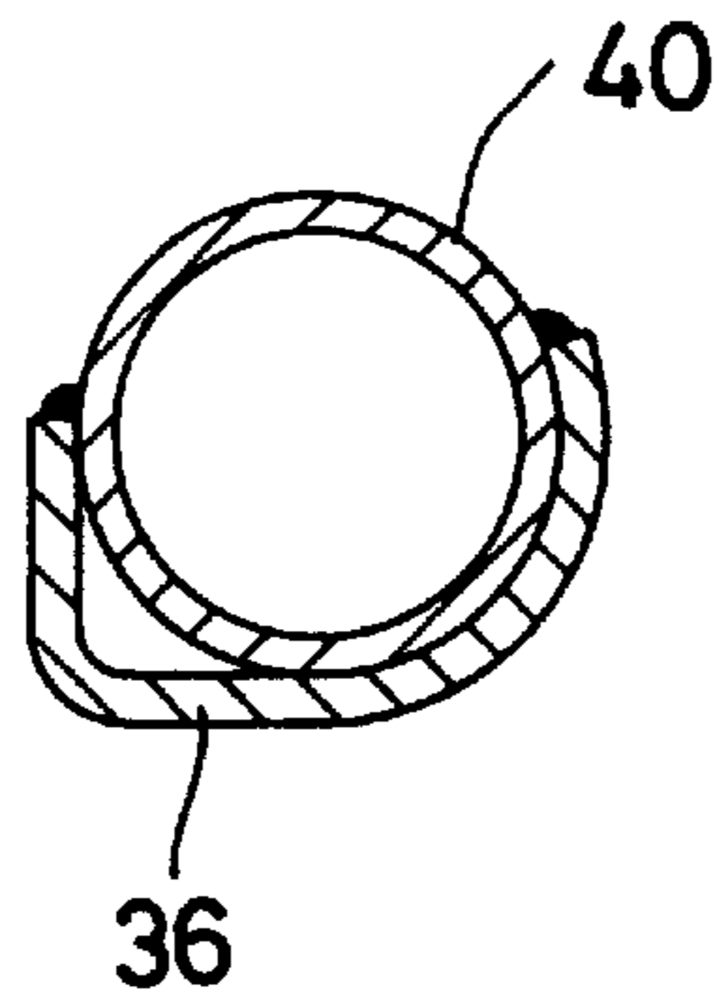
FIG.18 (RELATED ART)
