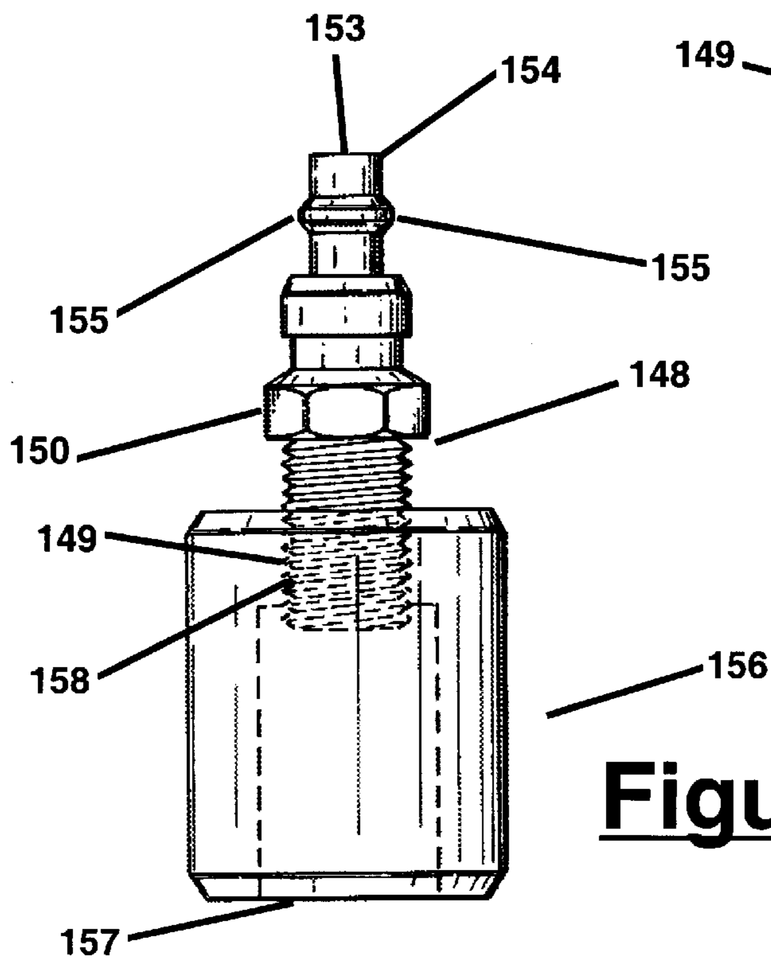
Figure 31 (PRIOR ART)
