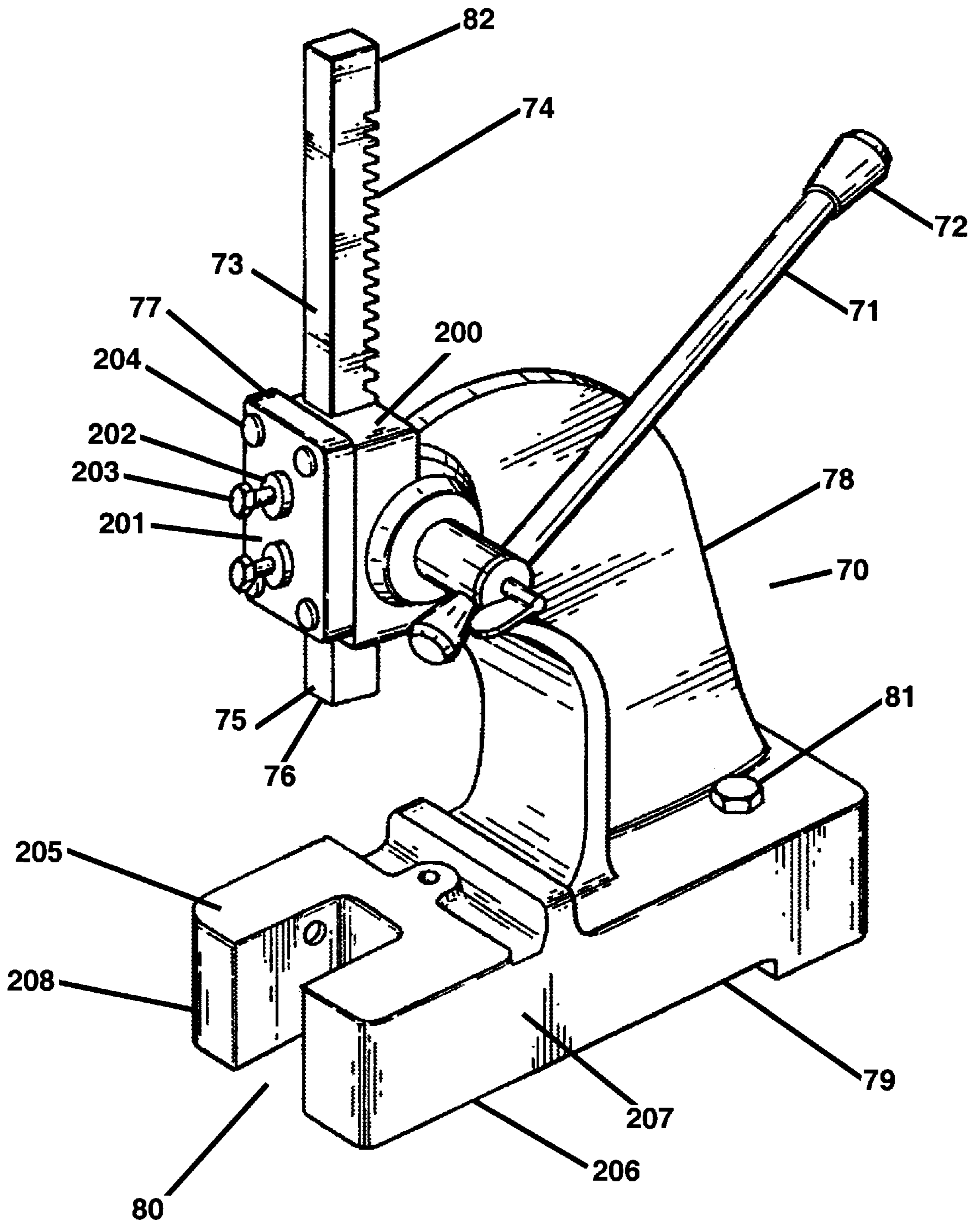
Figure 11 (PRIOR ART)
