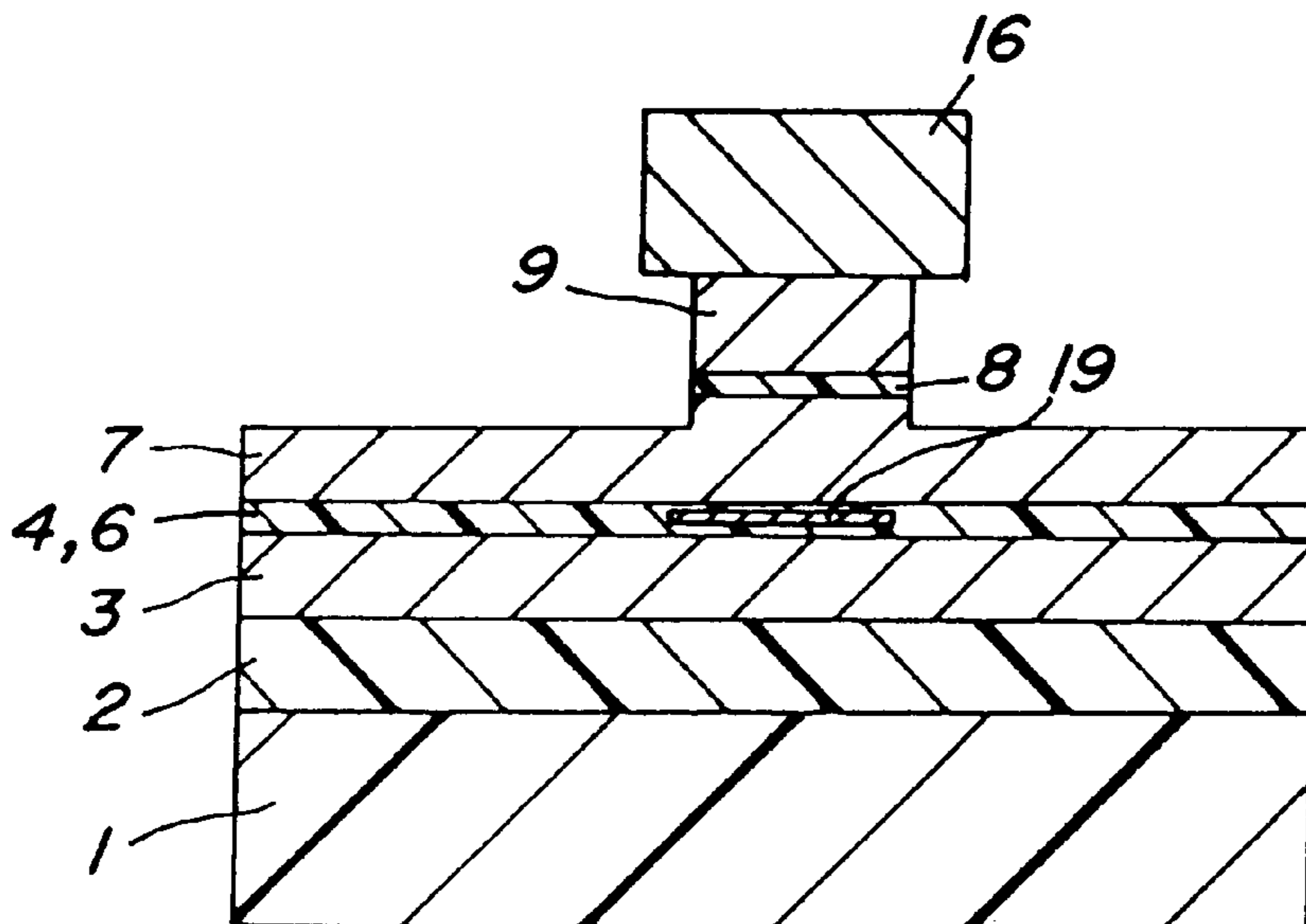
FIG. 11 PRIOR ART
