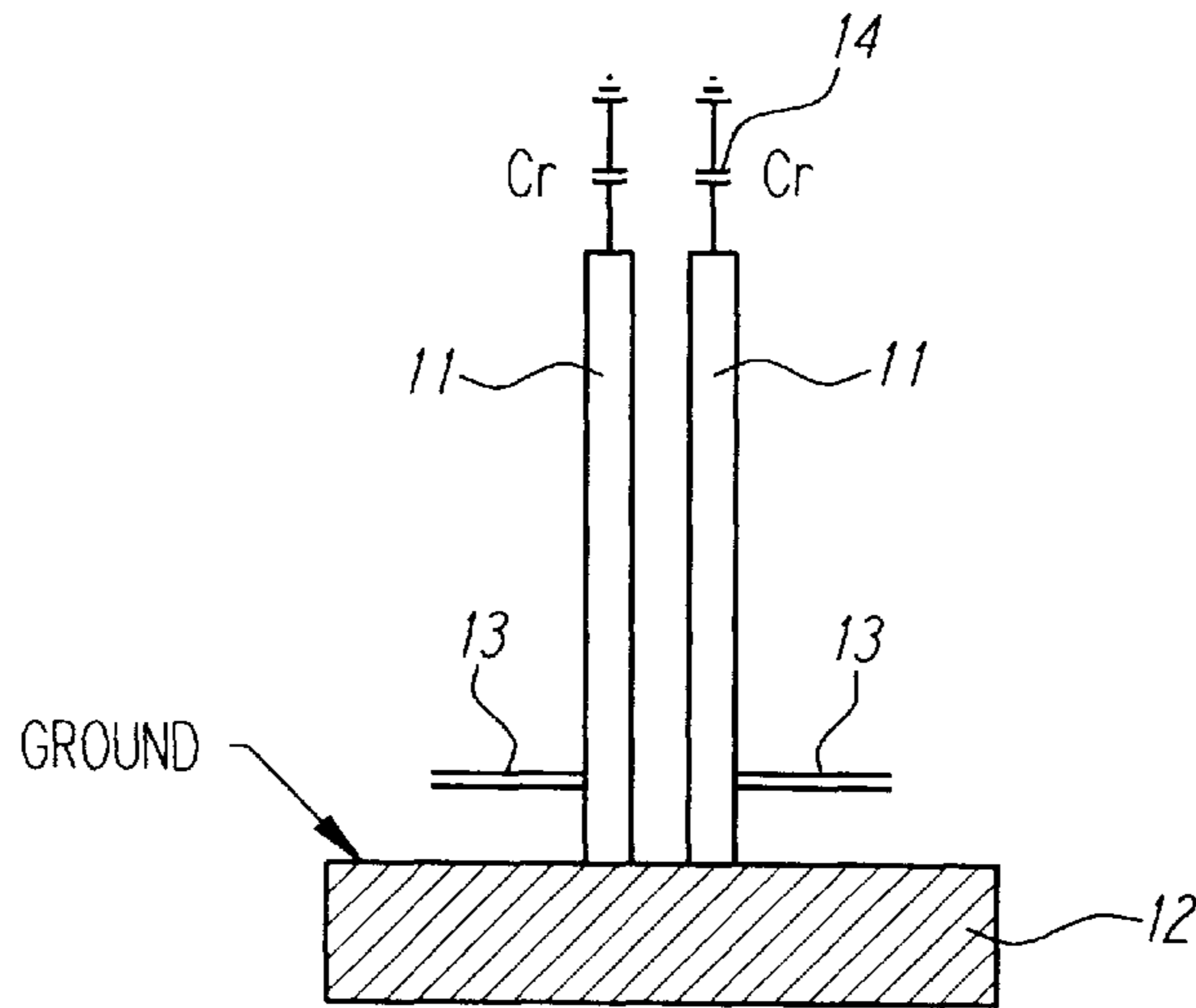
FIG. 1 (PRIOR ART)
