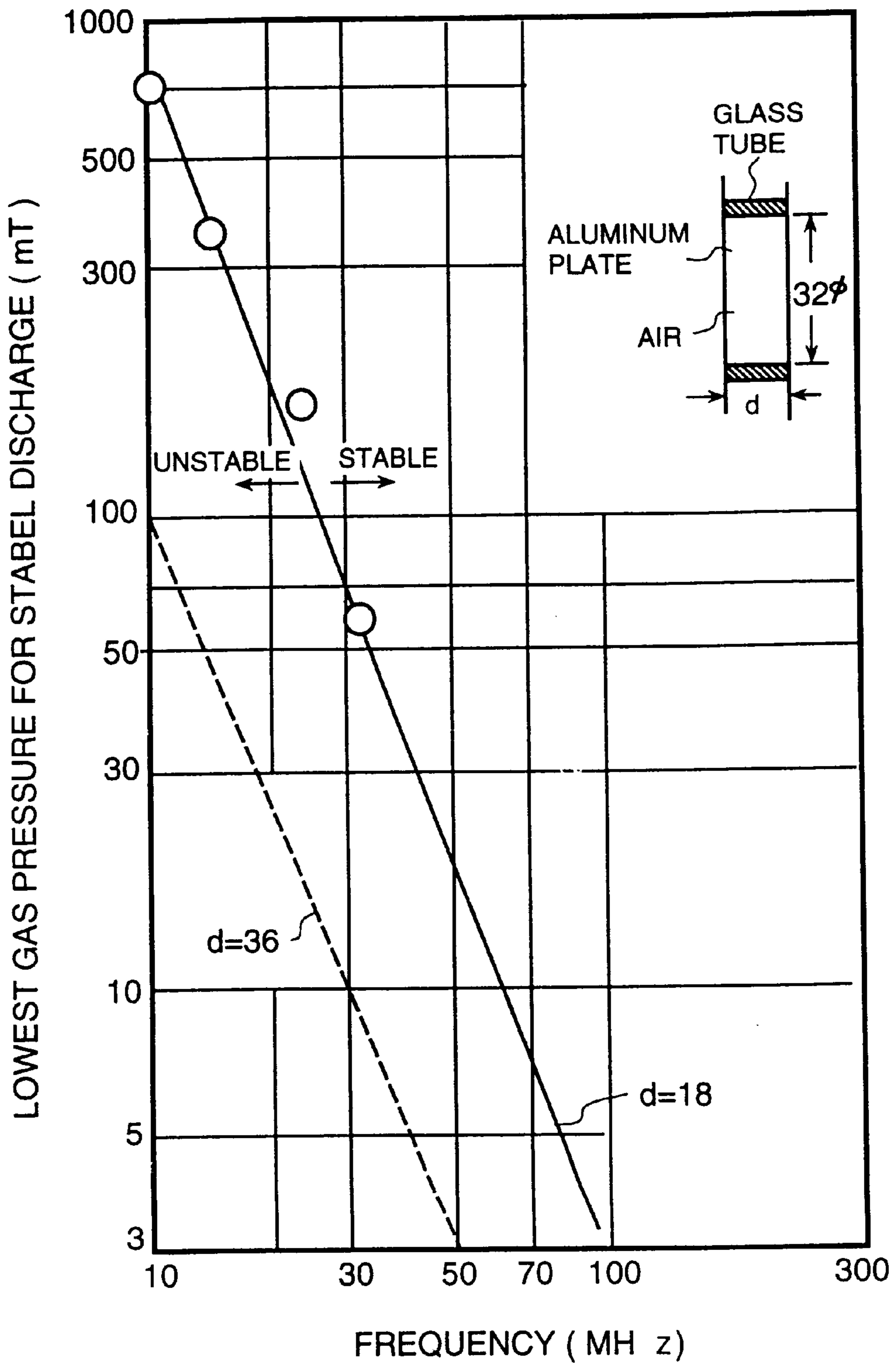
FREQUENCY-LOWEST GAS PRESSURE FOR STABLE DISCHARGE CHARACTERISTIC
