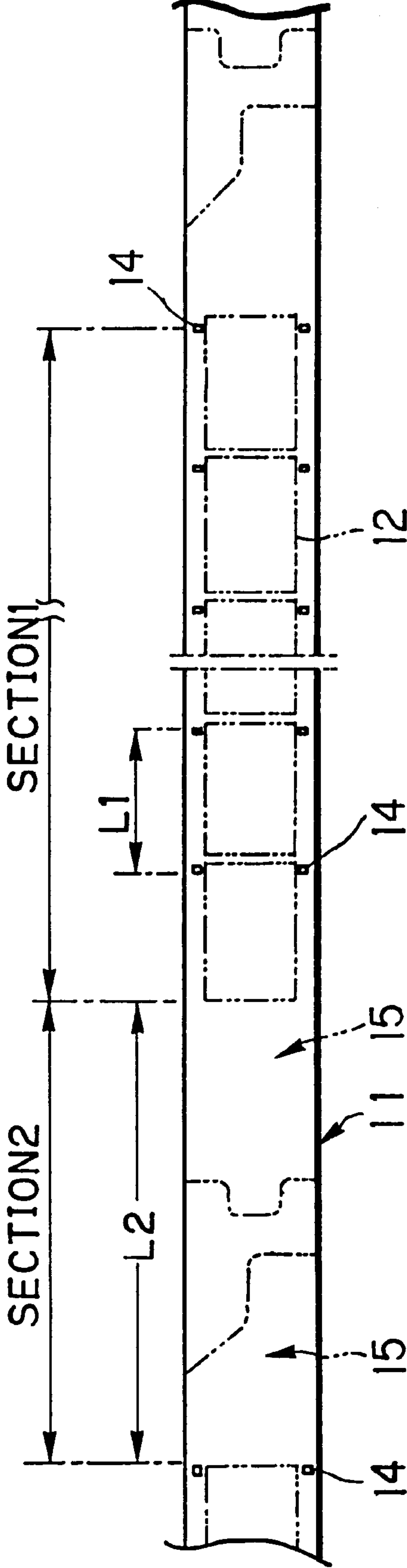
FIG. 26 PRIOR ART
