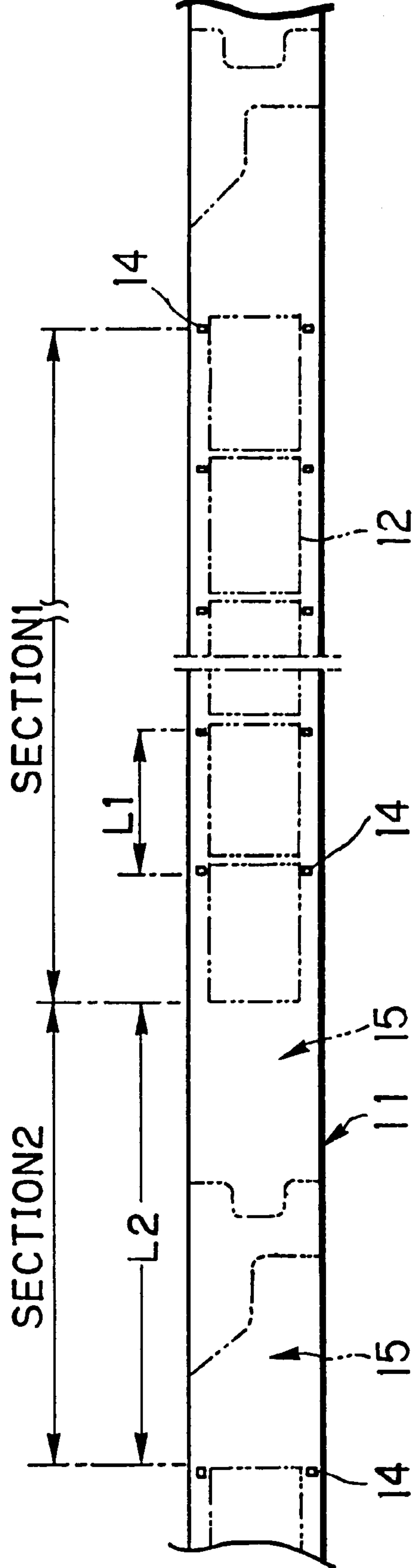
FIG. 26 PRIOR ART
