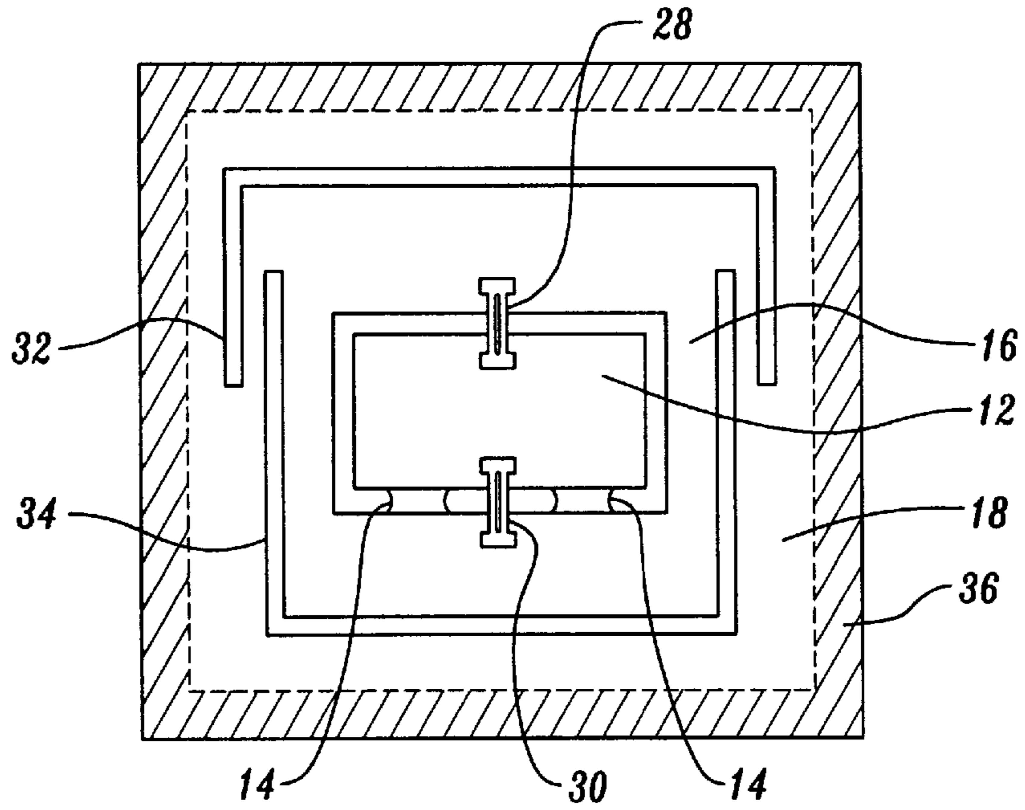
Fig. 2 (PRIOR ART)
