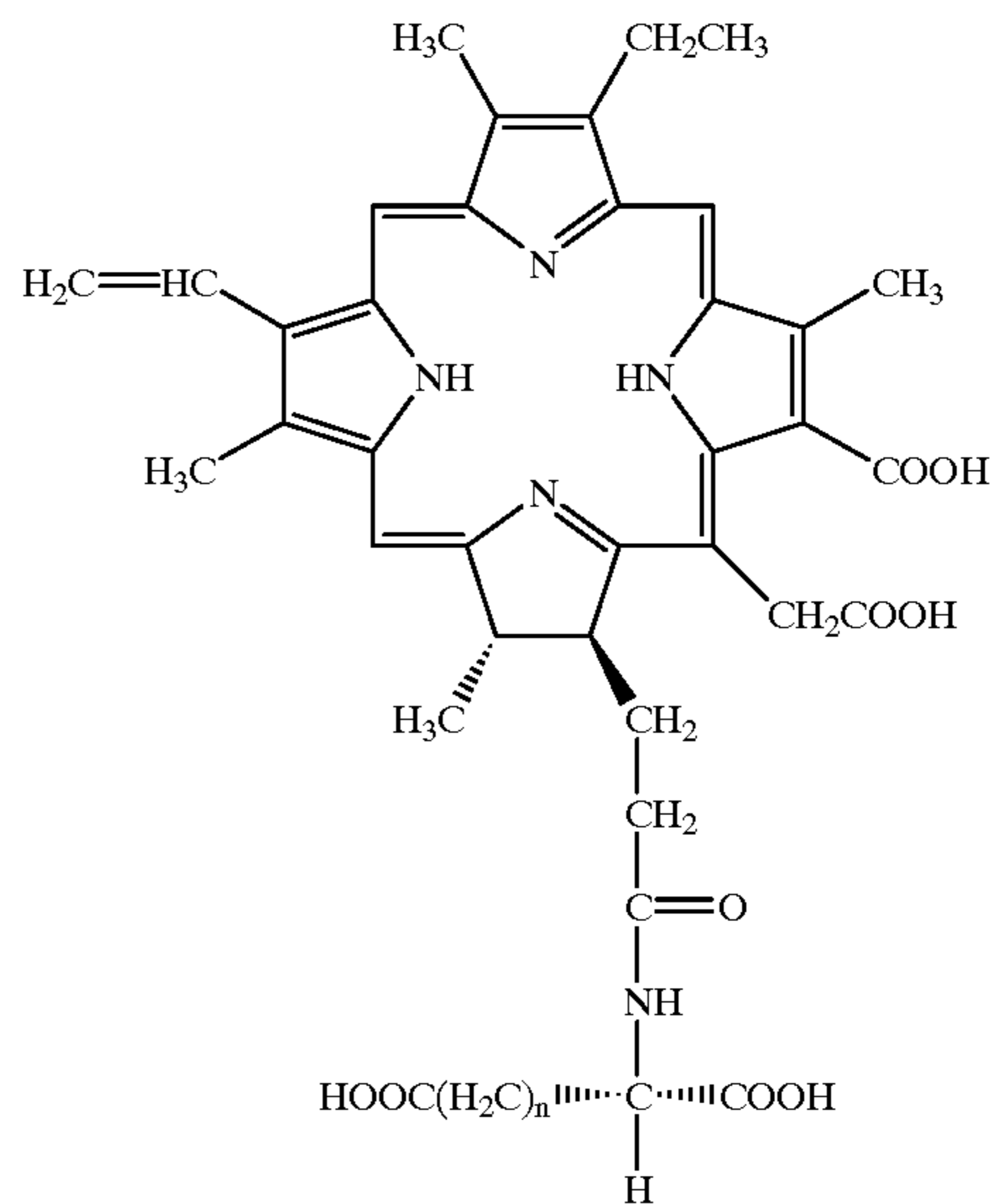
[CHEMICAL FORMULA 4]
