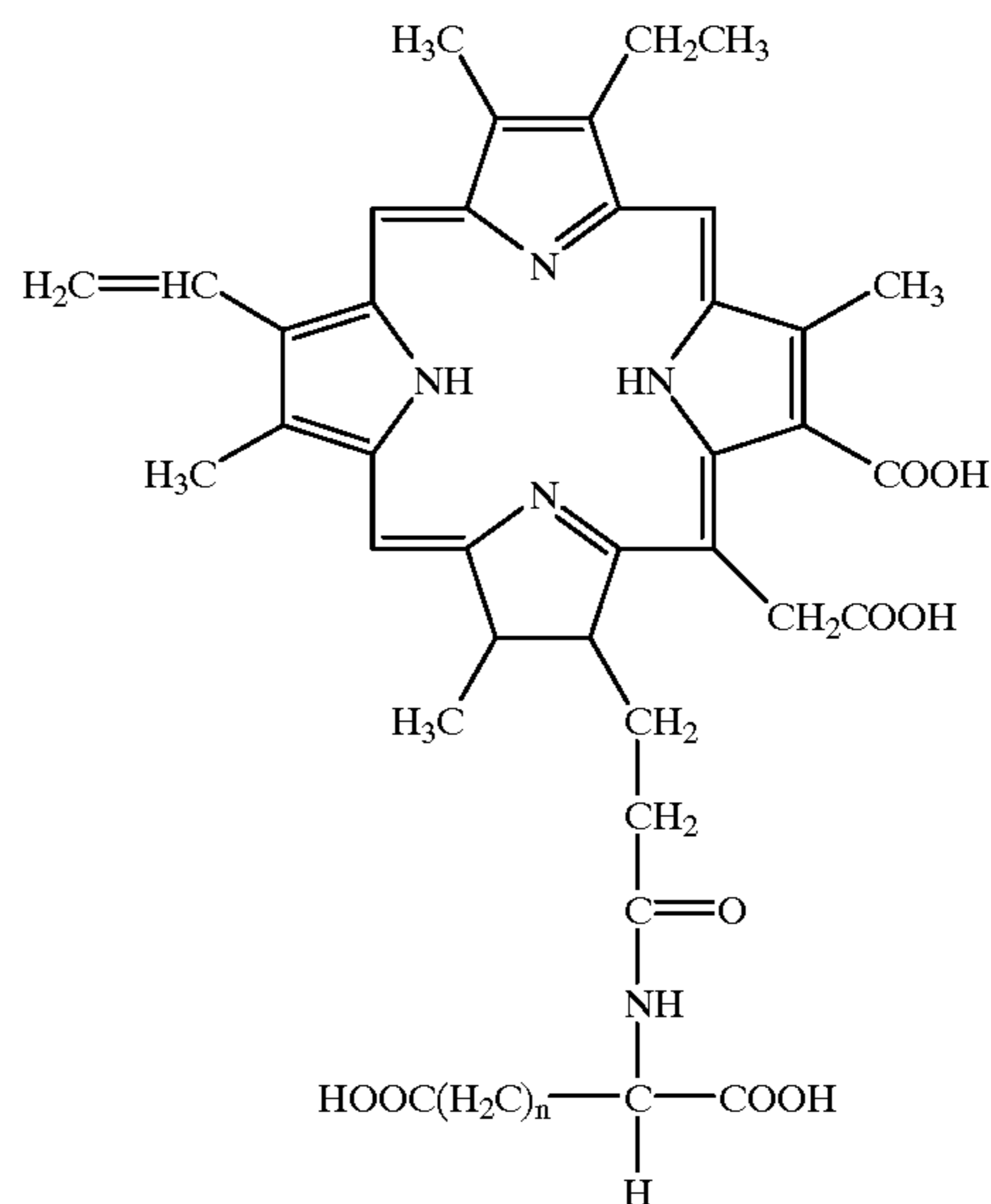
[CHEMICAL FORMULA 3]
