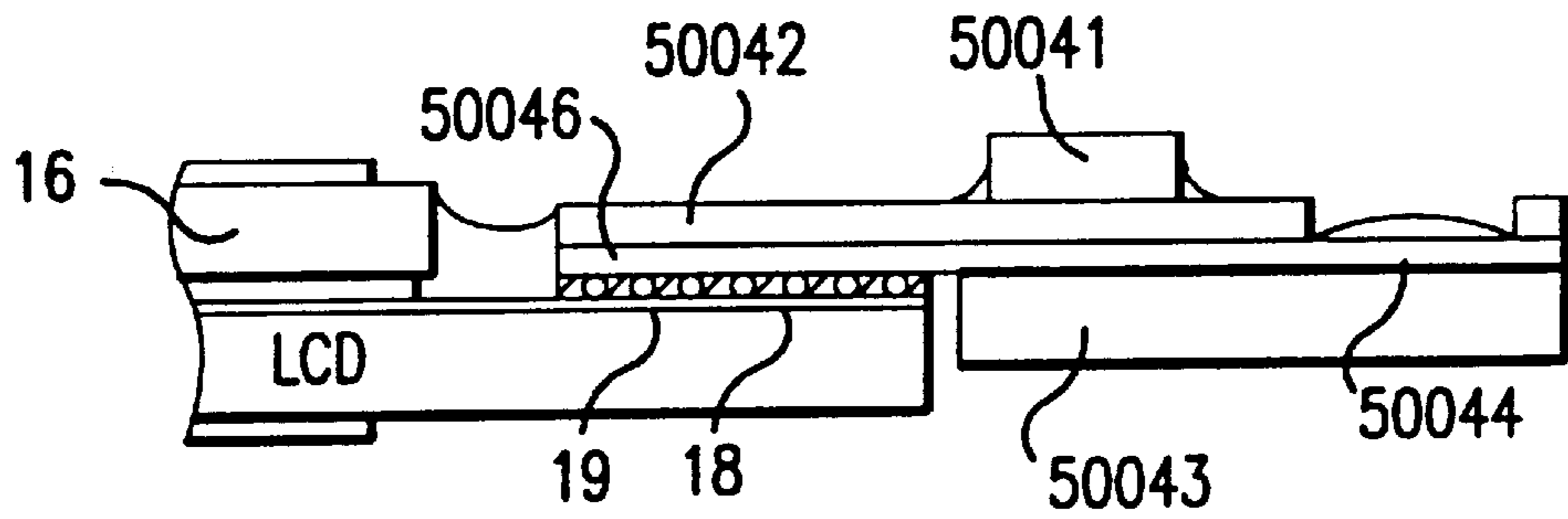
FIG.92 PRIOR ART
