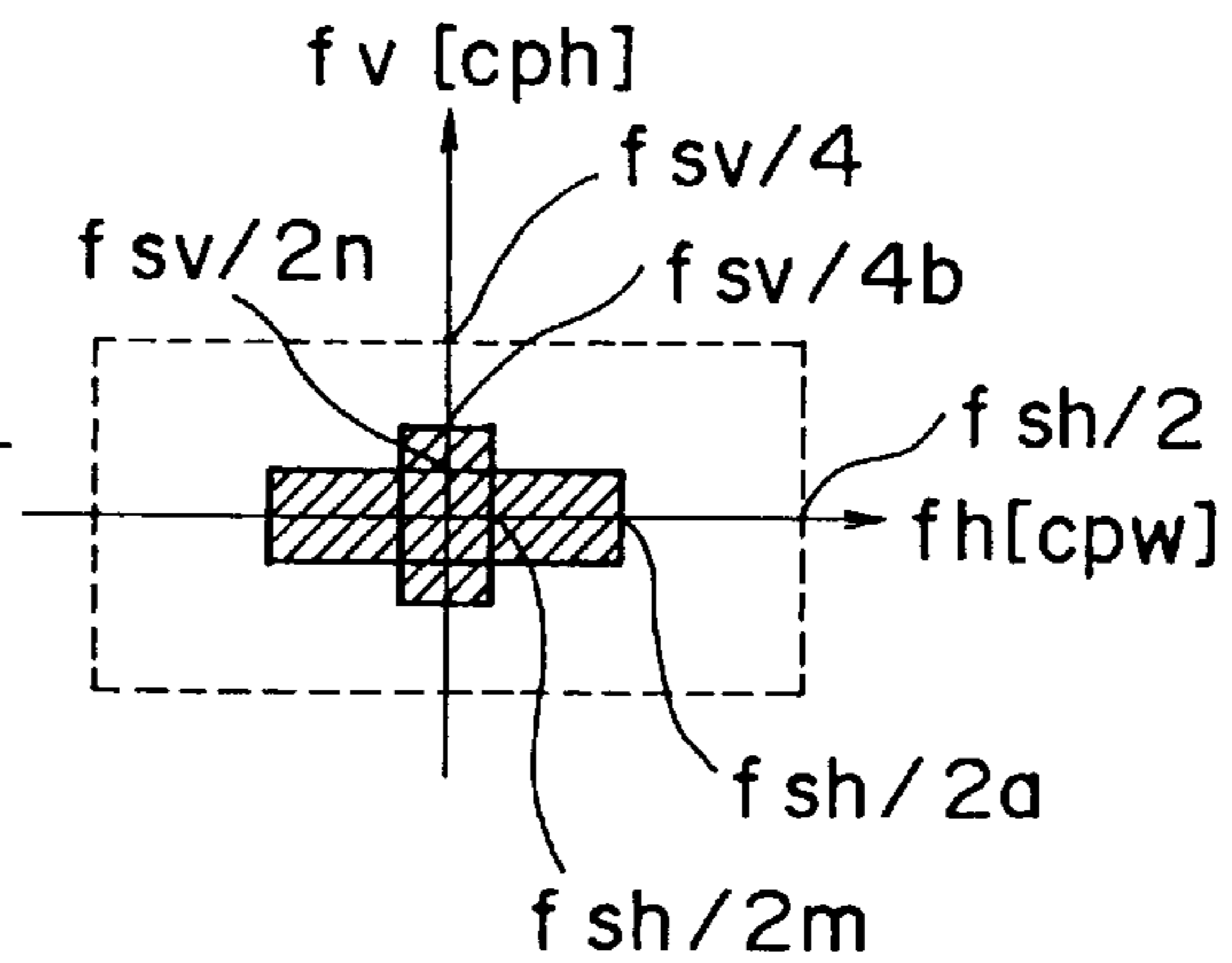
TWO-DIMENSIONAL FREQUENCY COMPONENT
