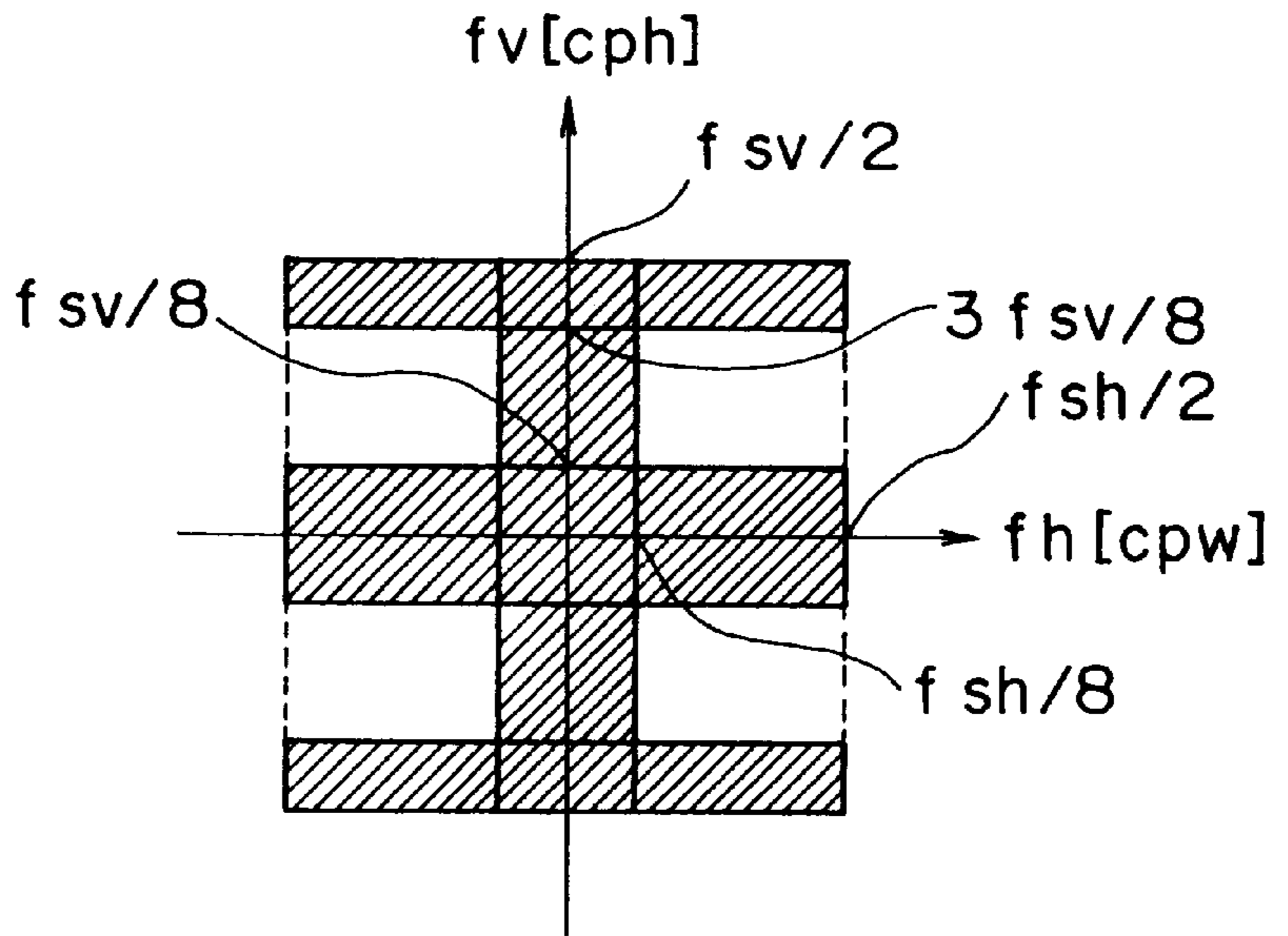
FRAME MATCHING ELEMENT FIG. 19A
