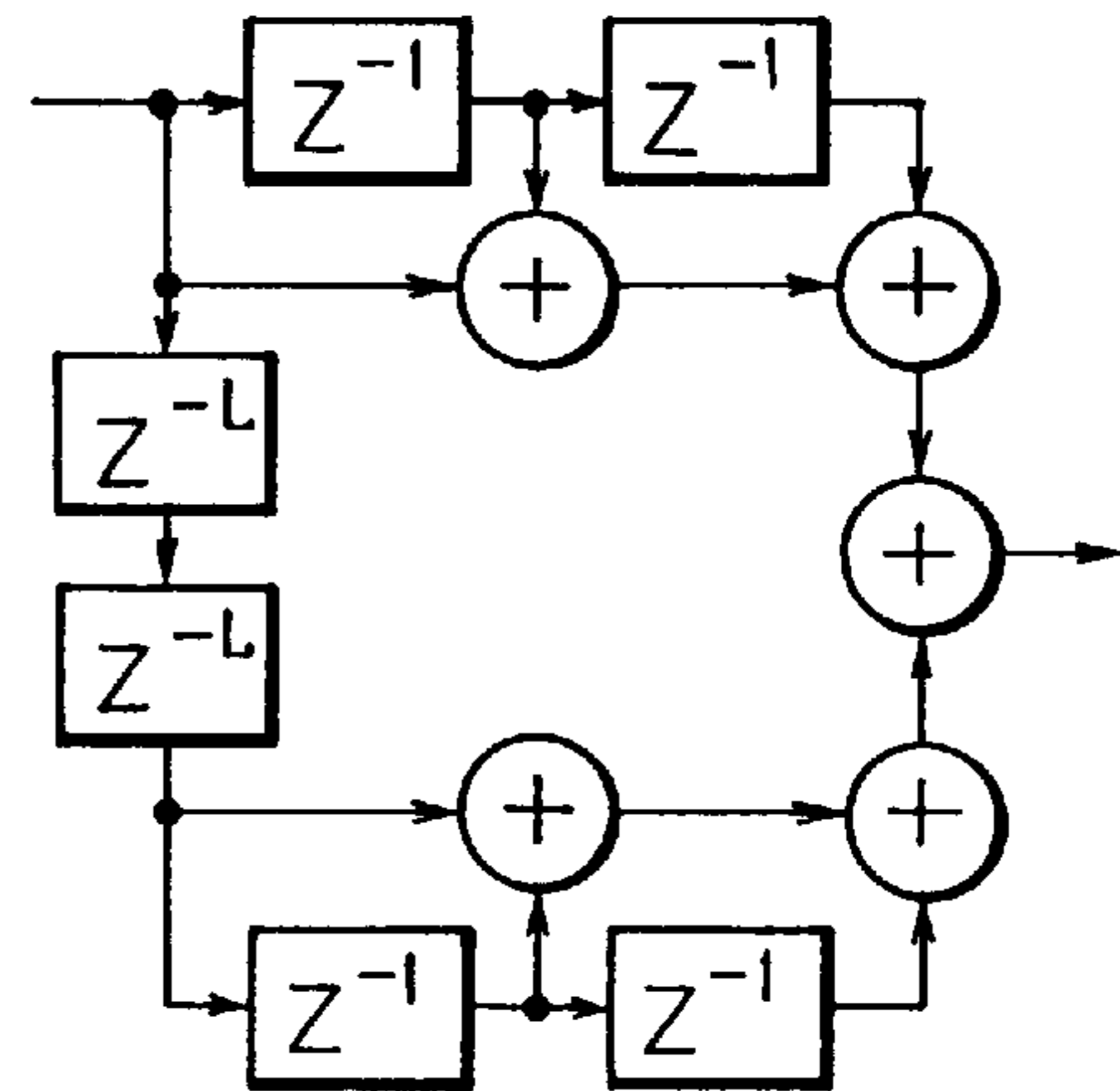
TWO-DIMENSIONAL FILTER (LPF)
