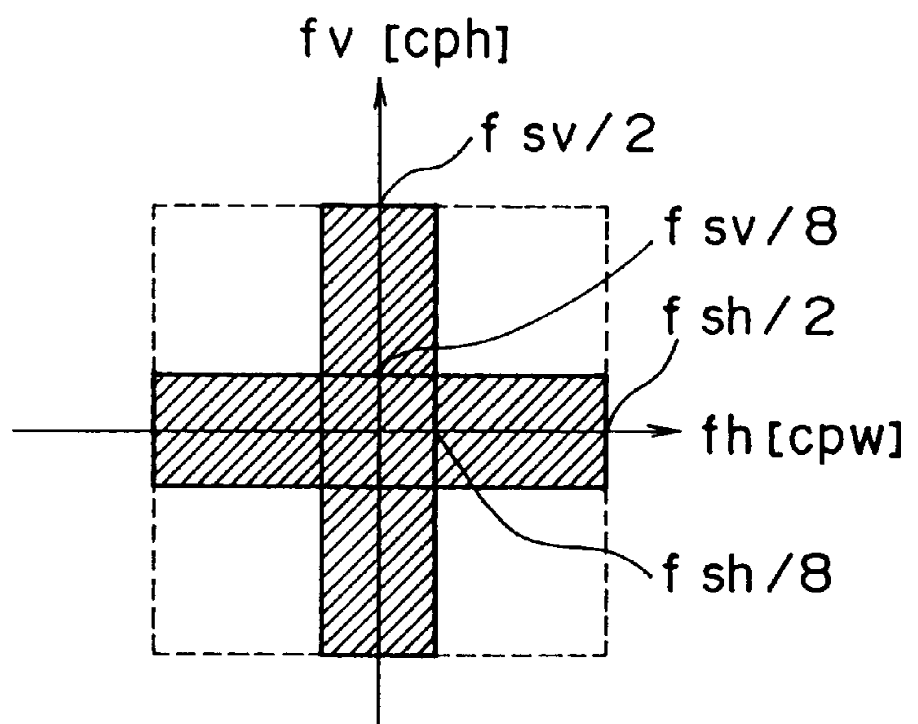
TWO-DIMENSIONAL FREQUENCY COMPONENT FIG. 16D
