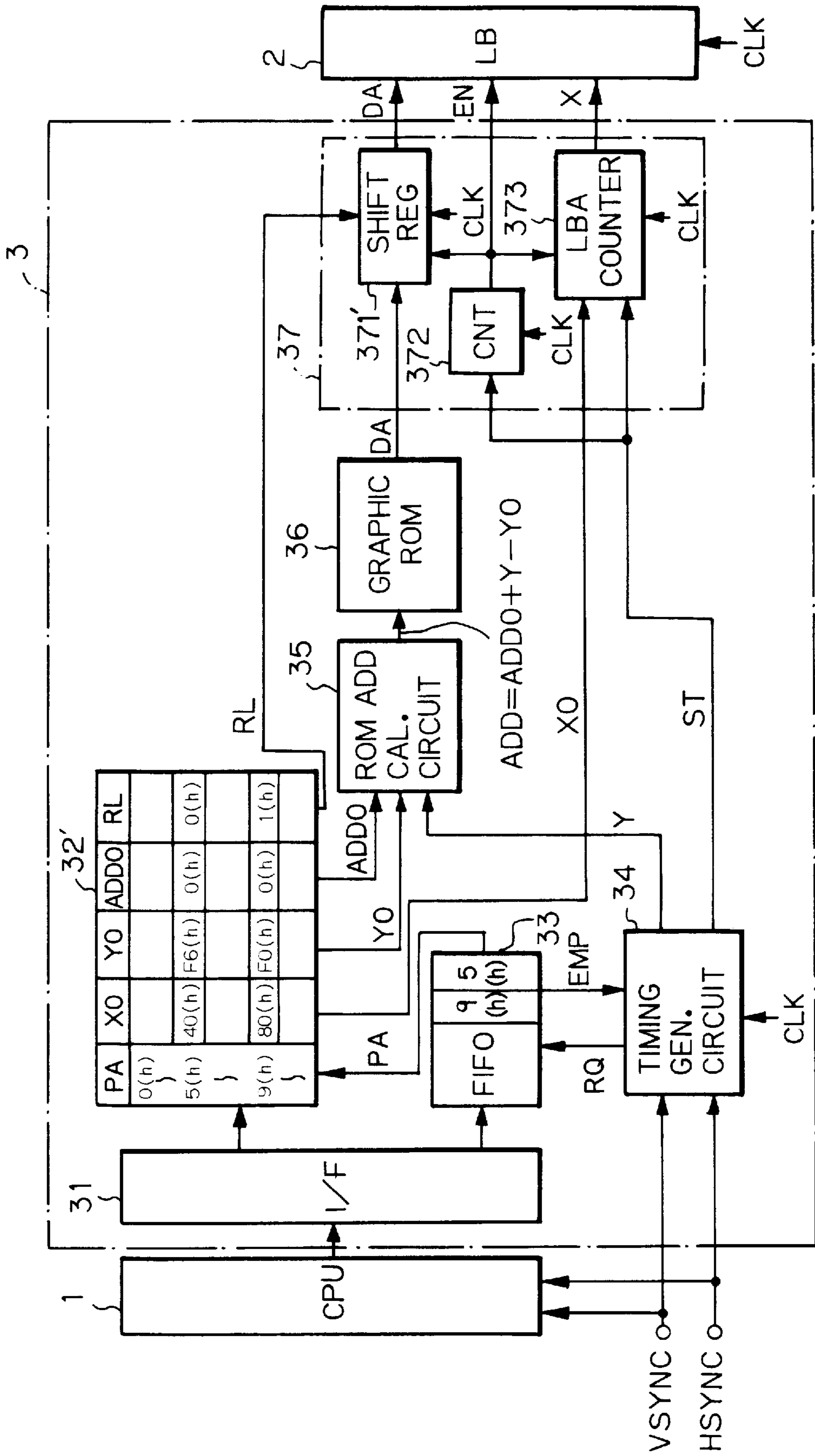
Fig. 10 PRIOR ART
