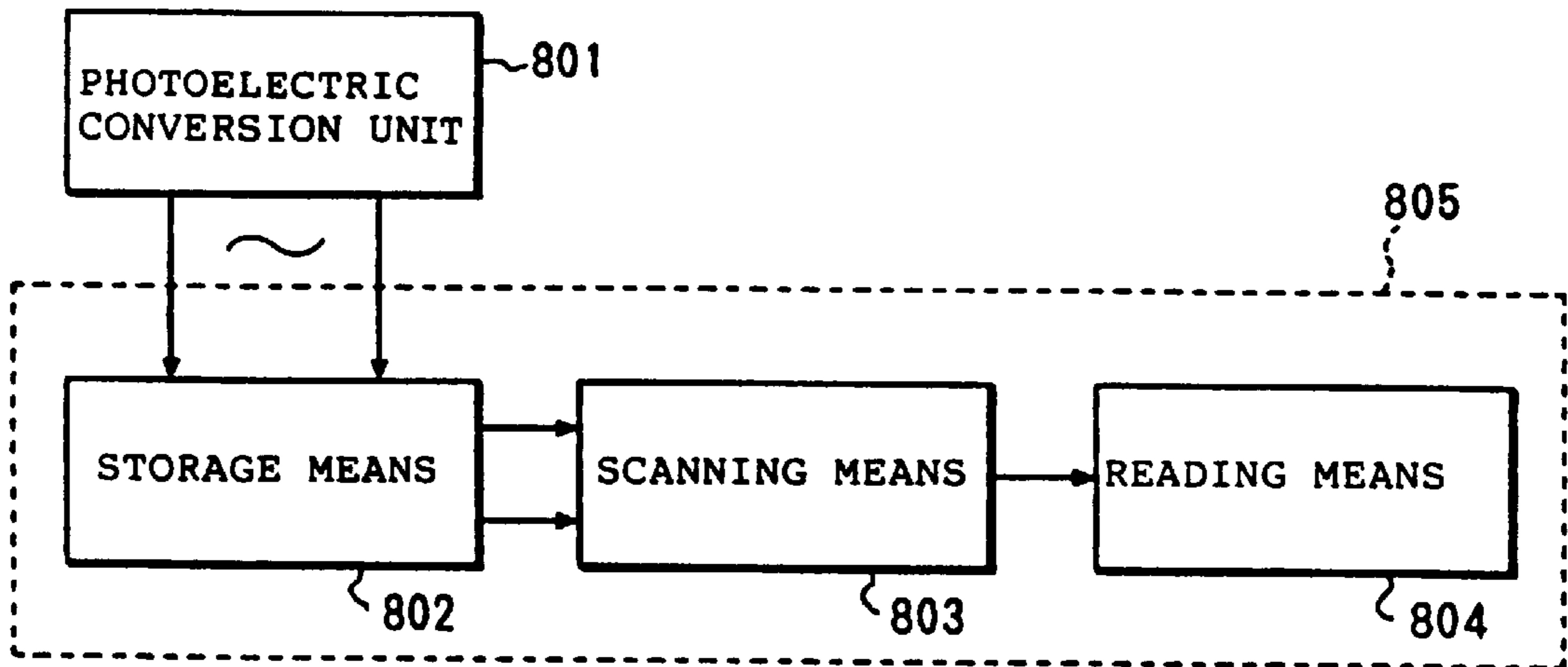
FIG. 31 PRIOR ART
