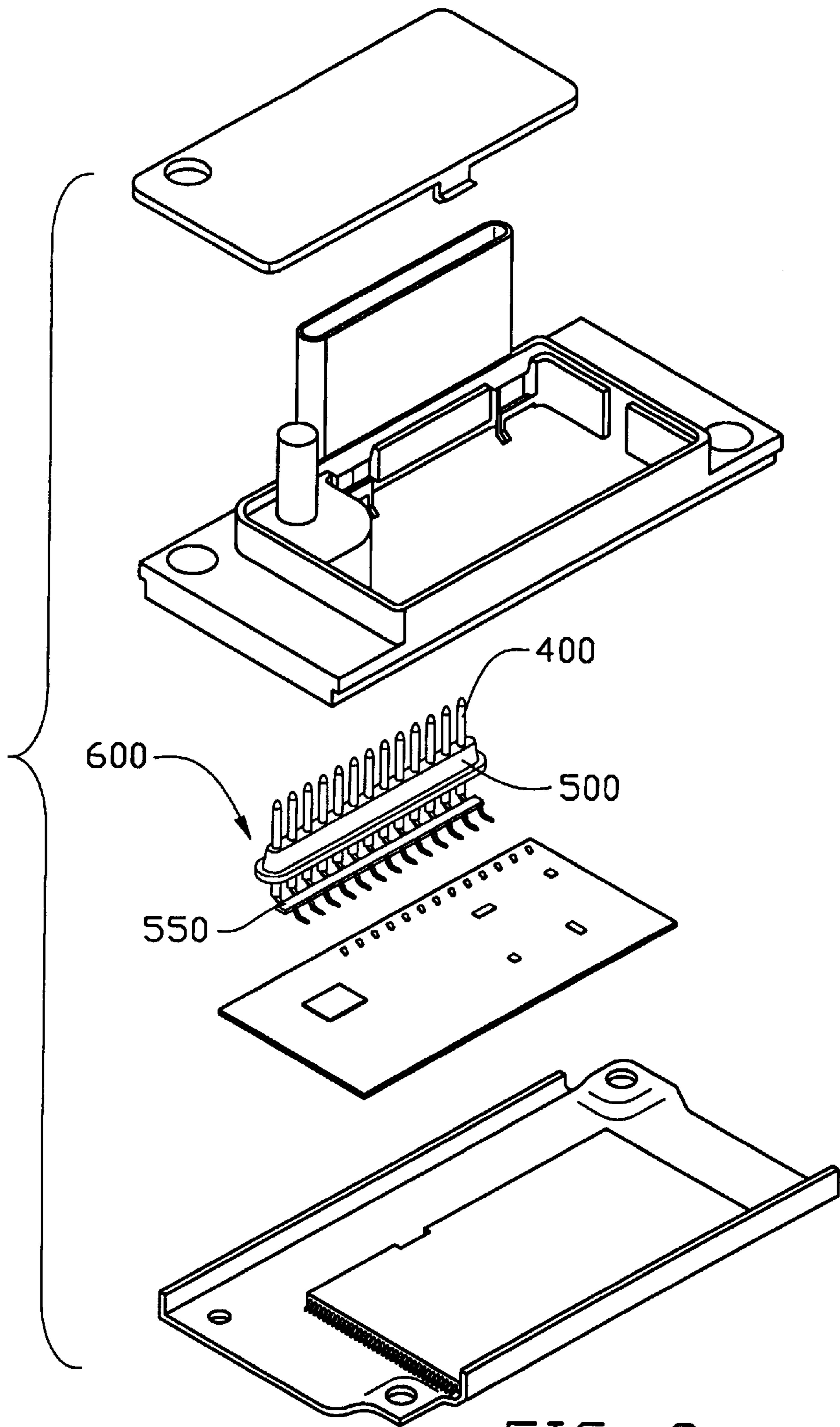
FIG. 2 (PRIOR ART)
