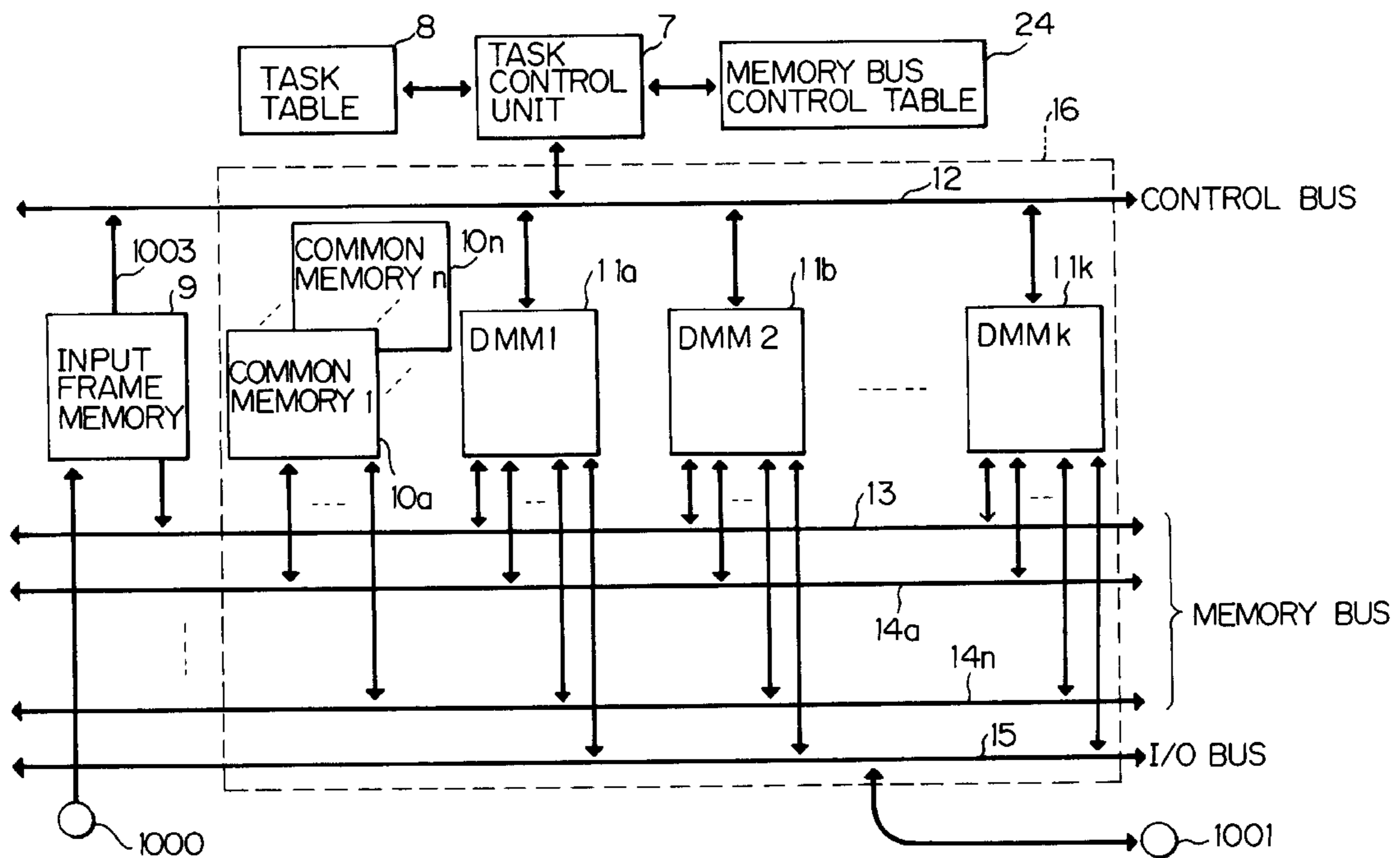
SINGLE-DMM MODULE ARRANGEMENT OF MULTIPROCESSOR TYPE TIME VARYING IMAGE ENCODING SYSTEM
