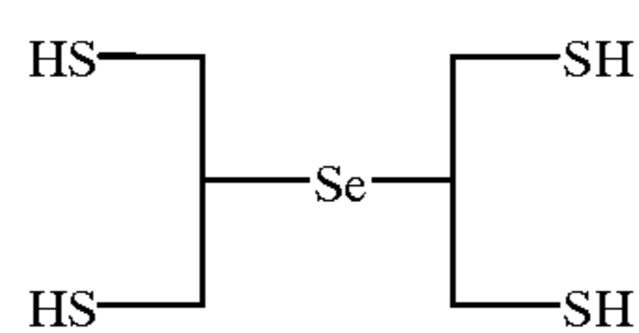
(Elemental analysis)
