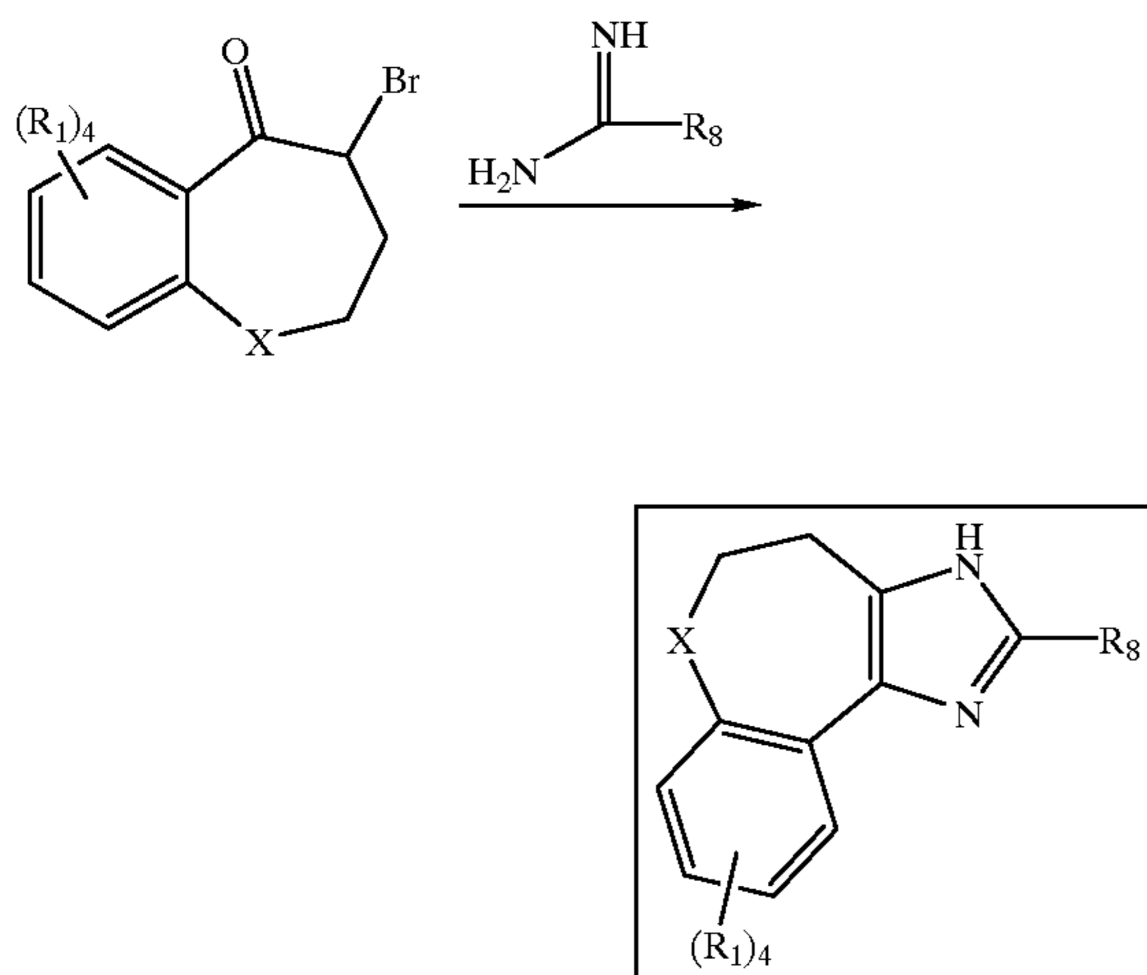
Scheme 4B Synthesis of Tricycles
