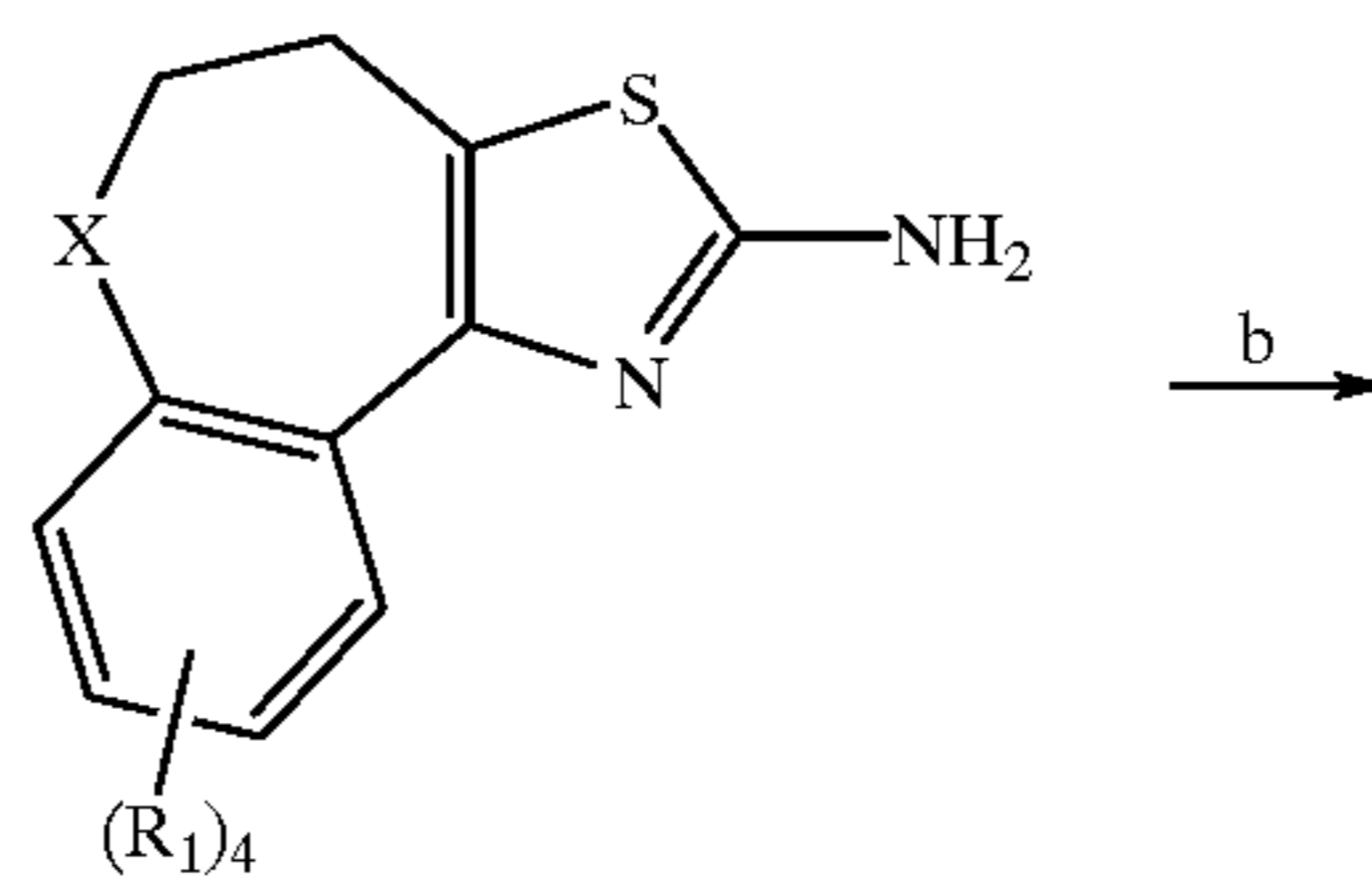
Scheme 3E Synthesis of the Tricycles
