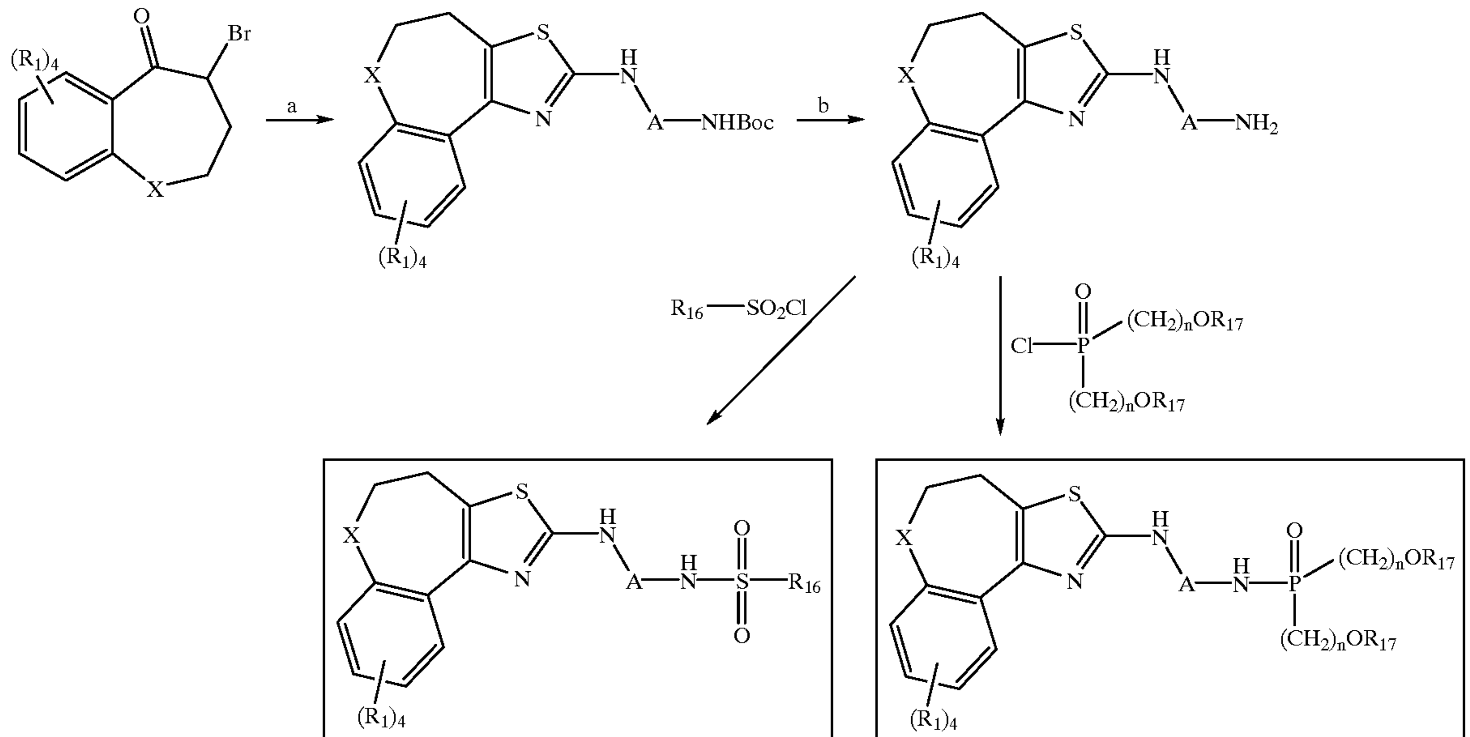
Scheme 3A Synthesis of the Tricycles
