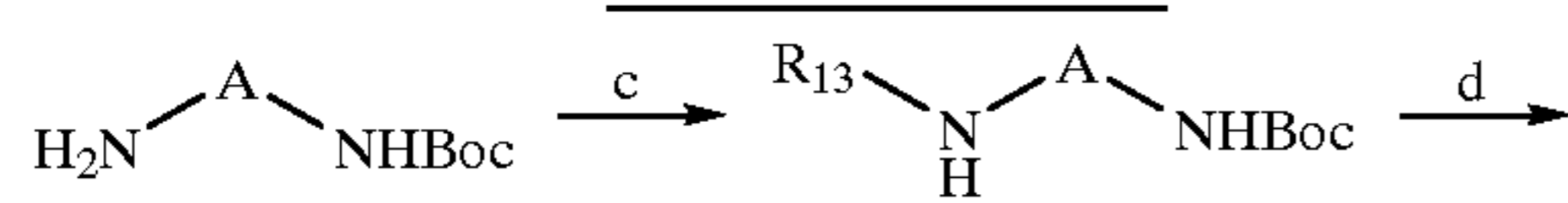
Scheme 1B. Synthesis of Thioureas
