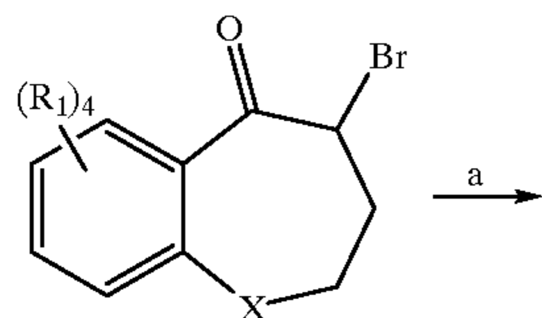
Scheme 3D Synthesis of the Tricycles
