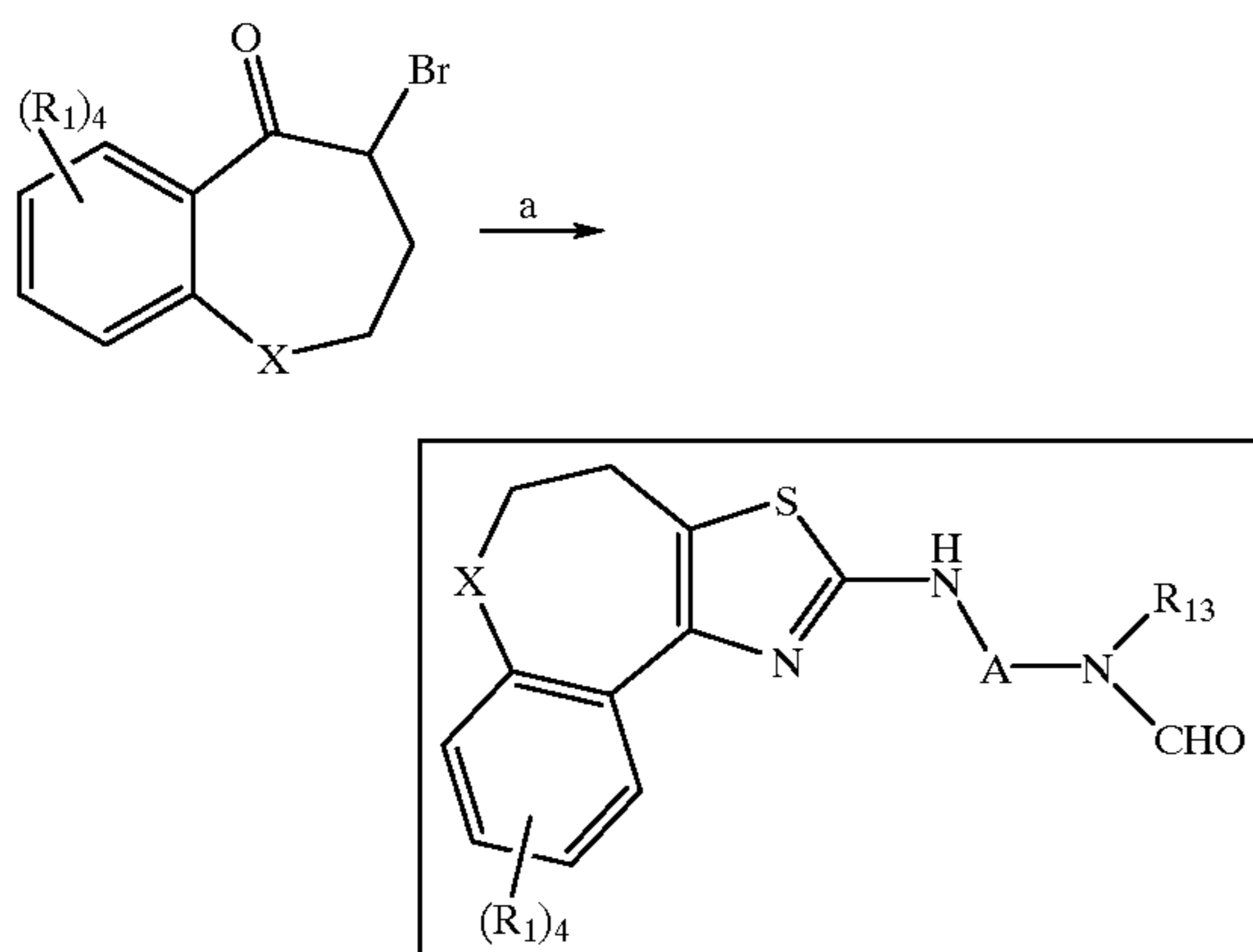
Scheme 3B Synthesis of the Tricycles
