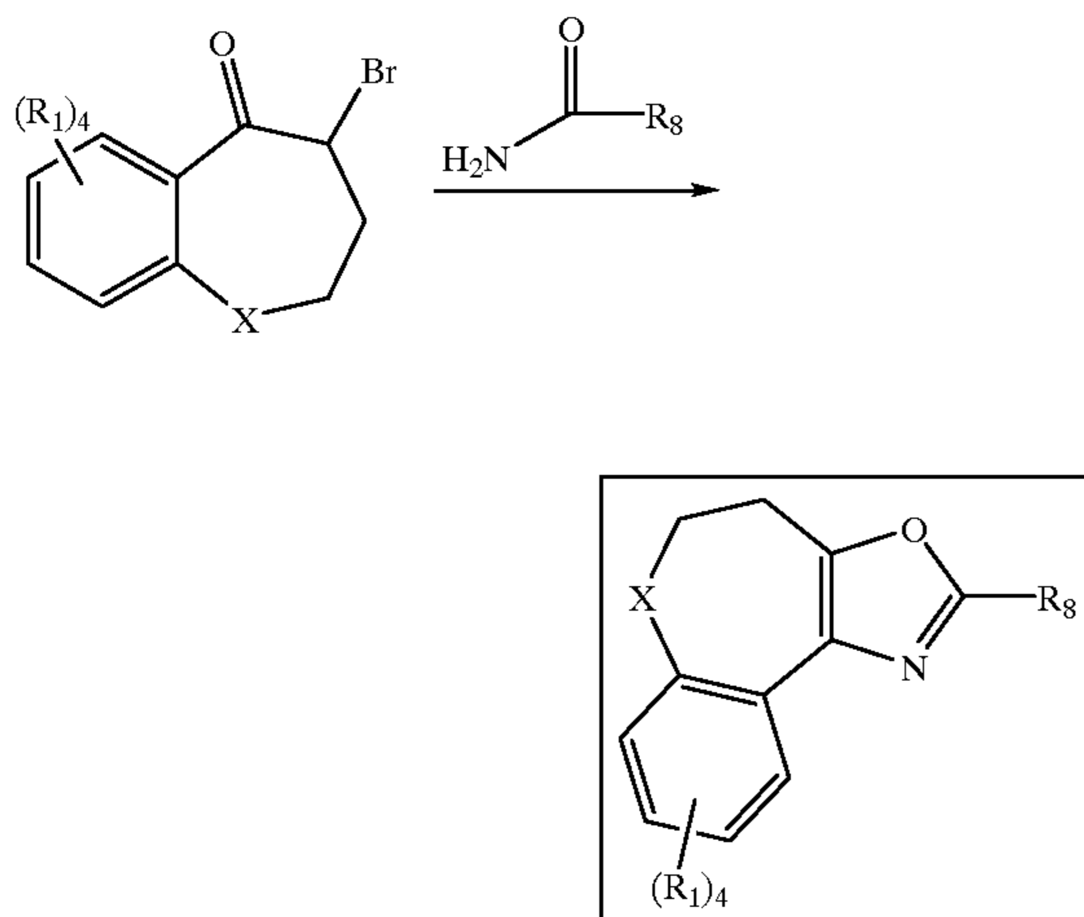
Scheme 4A Synthesis of Tricycles
