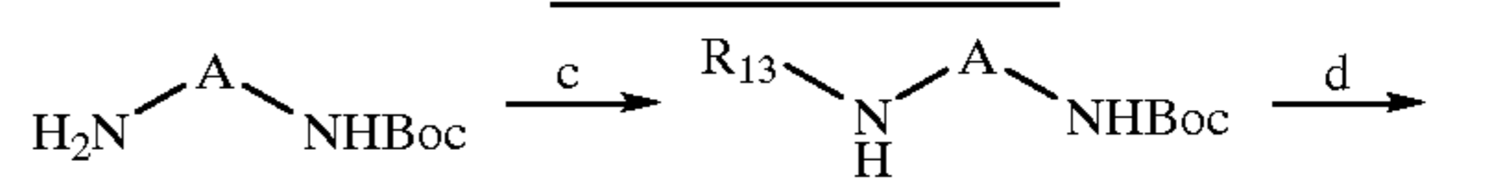
Scheme 1C. Synthesis of Thioureas
