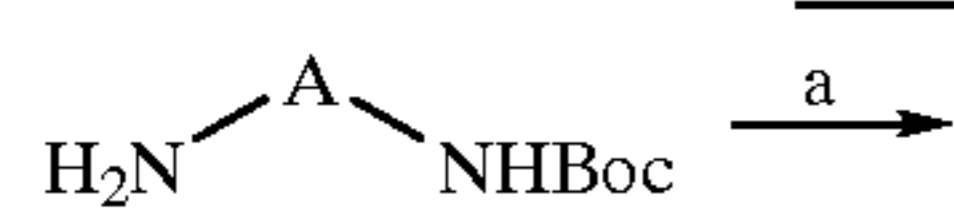
Scheme 1A. Synthesis of Thioureas
