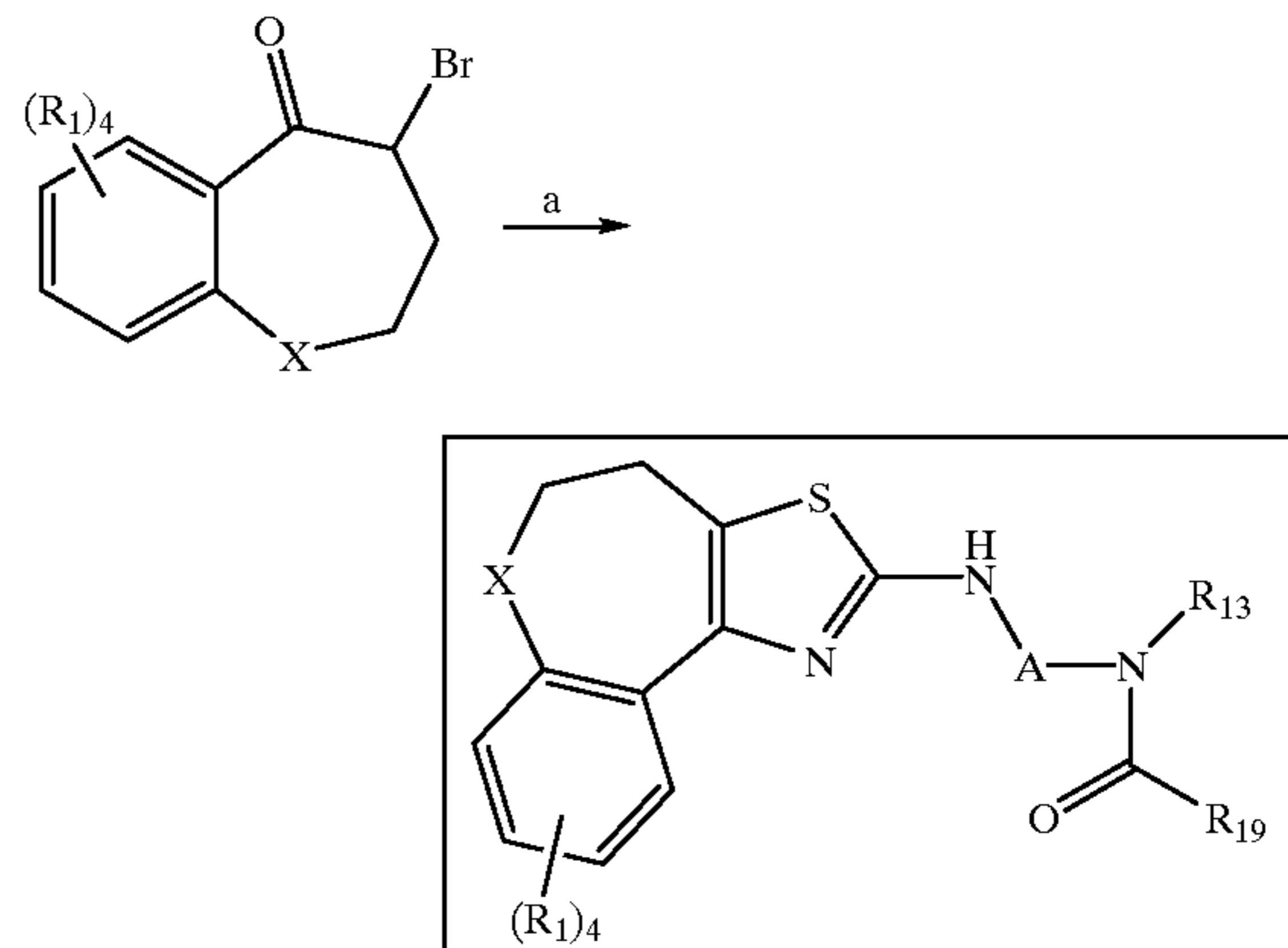
Scheme 3C Synthesis of the Tricycles
