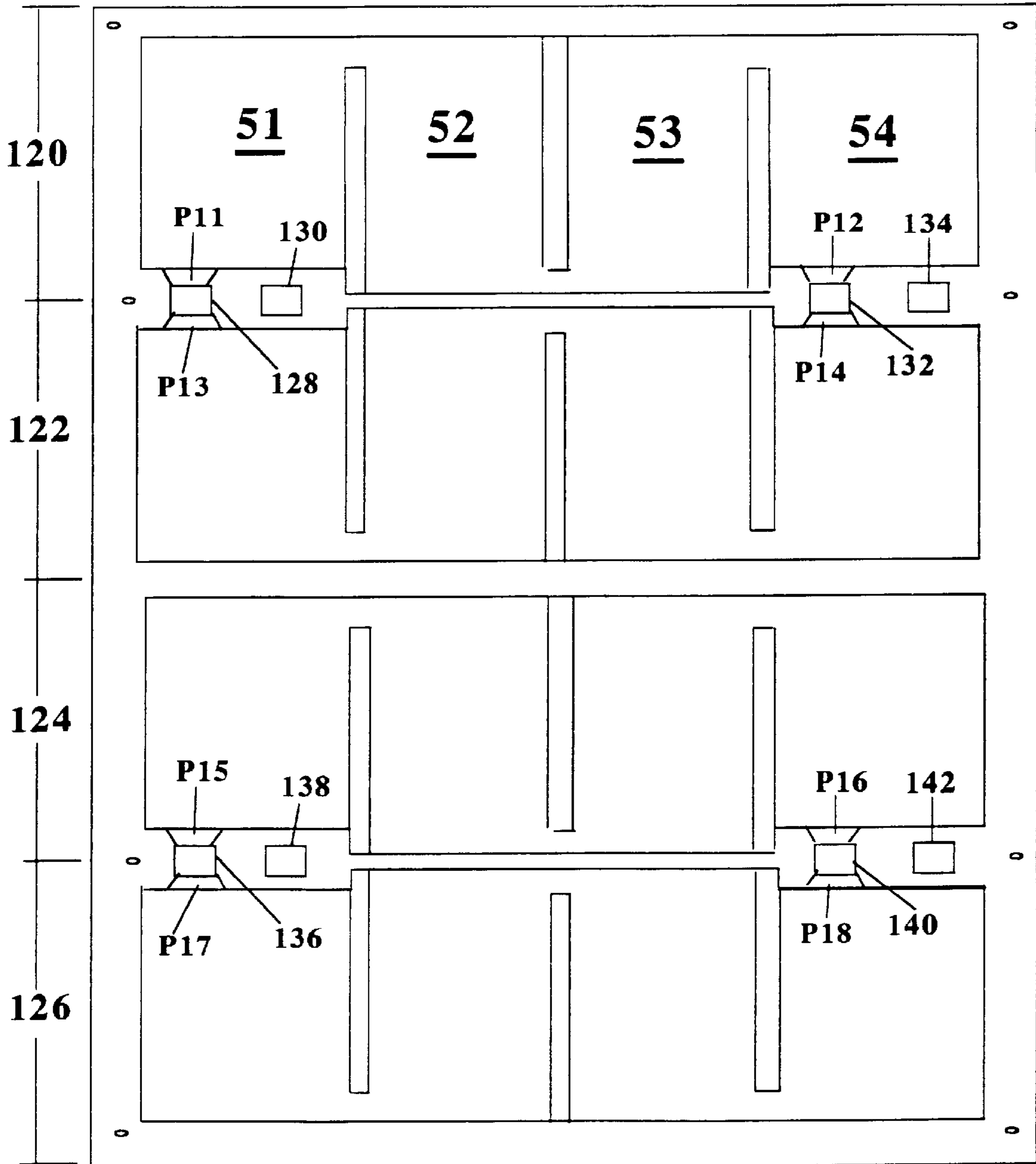
Fig. 5: Gasket with Four Series Flow Paths
