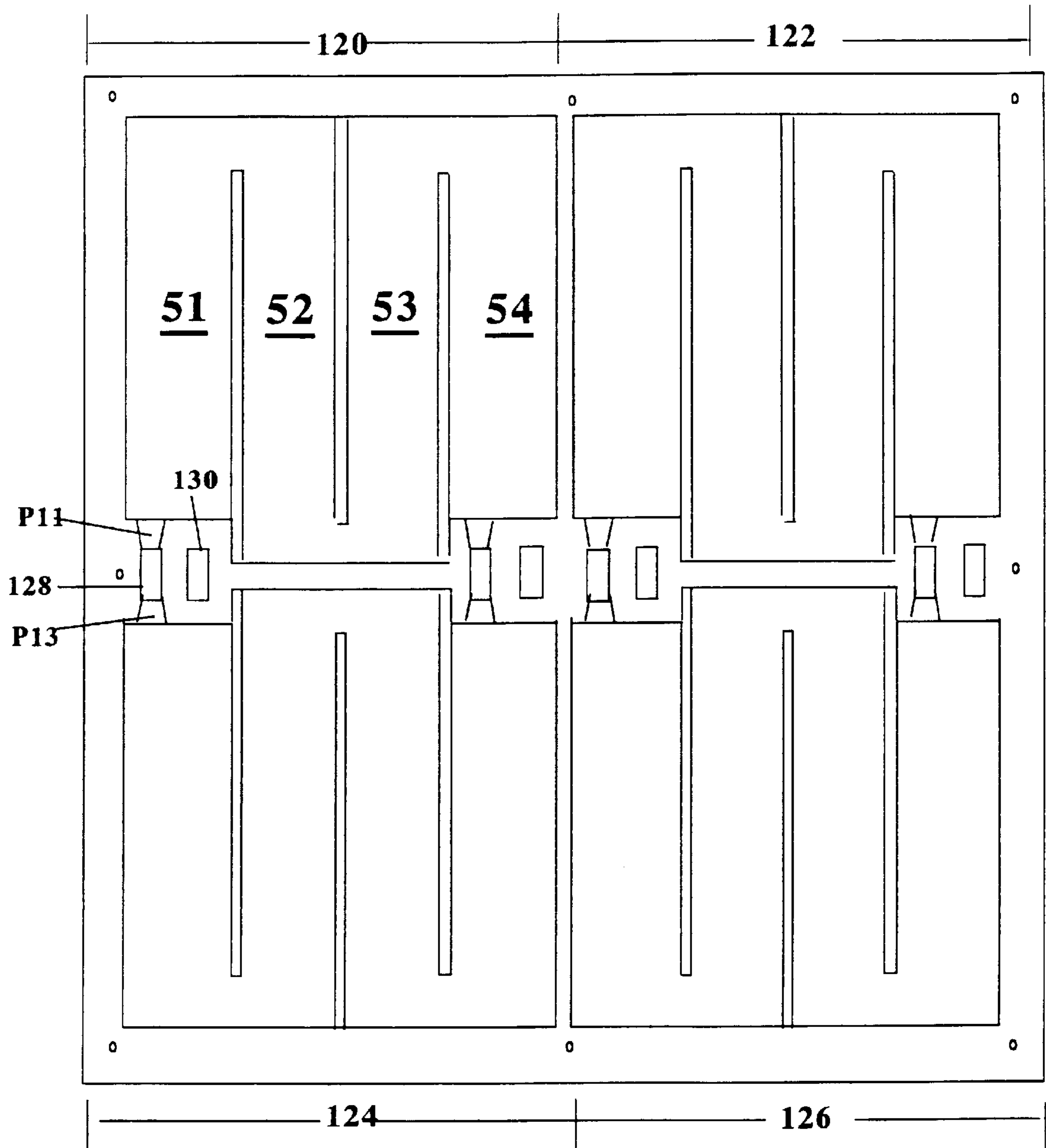
Fig. 5(a): Gasket with Four Series Flow Paths
