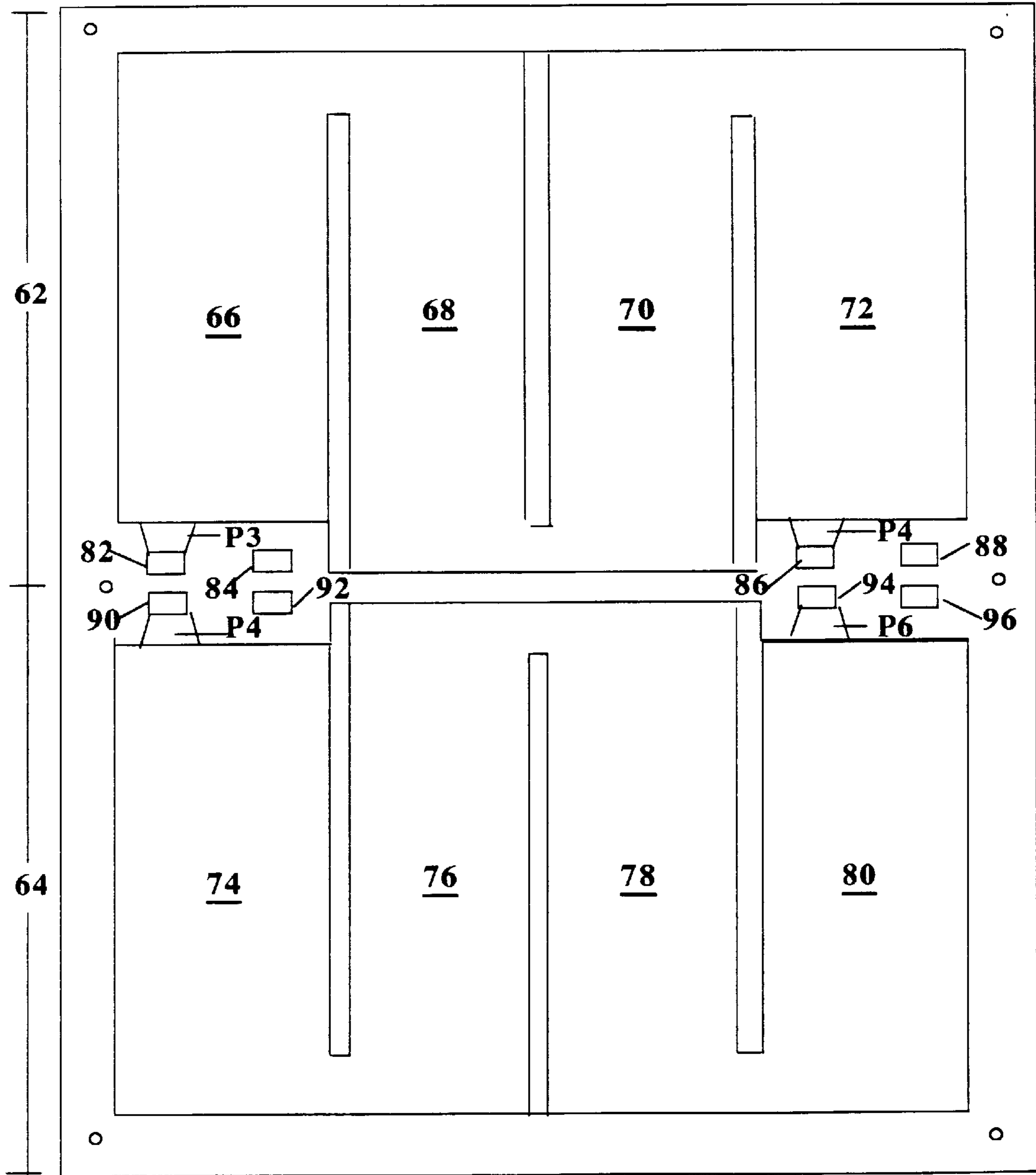
Fig. 2: Gasket with Two Series Flow Paths 8 Manifold holes, 4 ports, 2 serie paths (6 corner alignment holes shown are typical)
