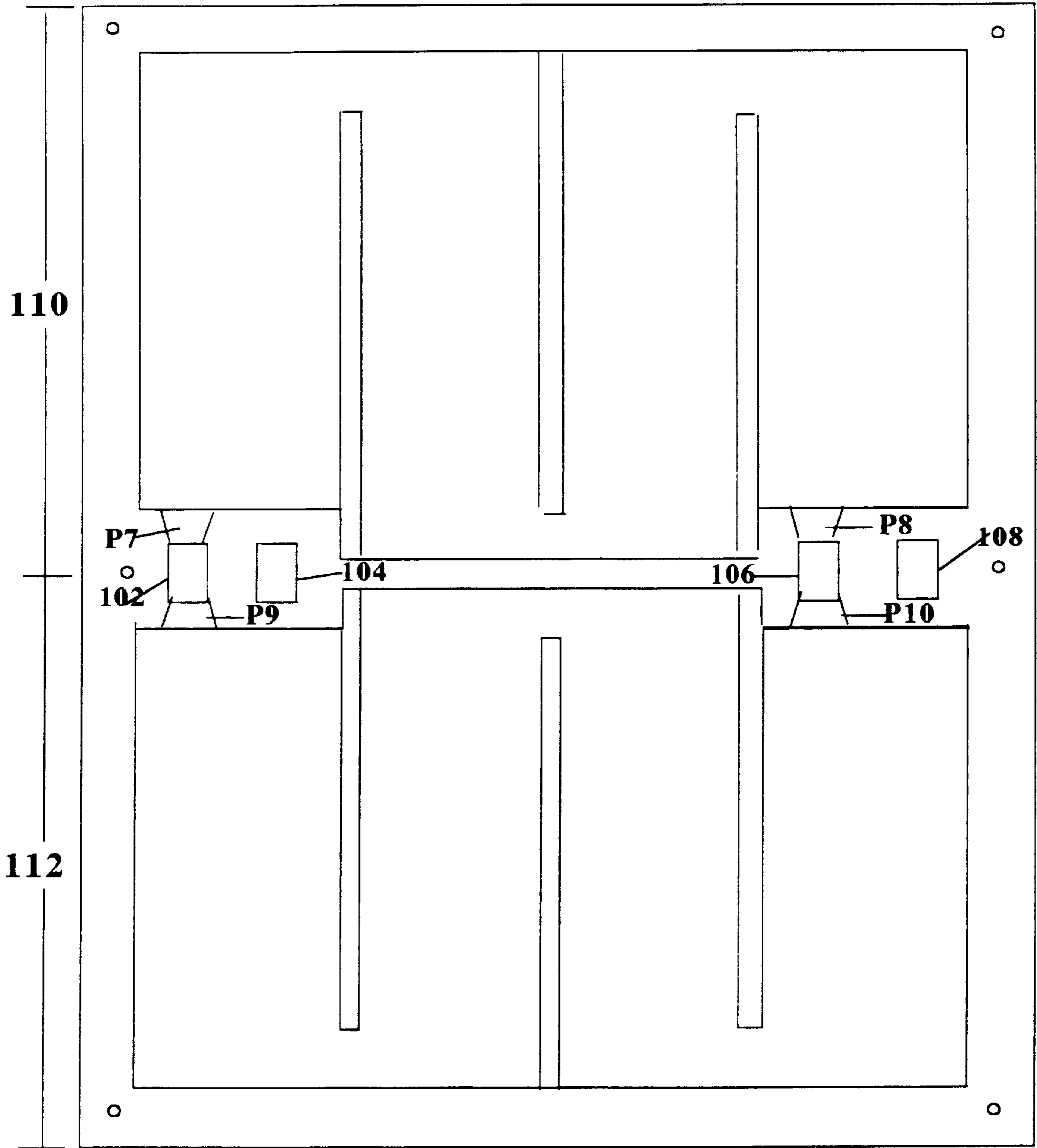
Fig: 4 Gasket with Two Series Flow Paths
