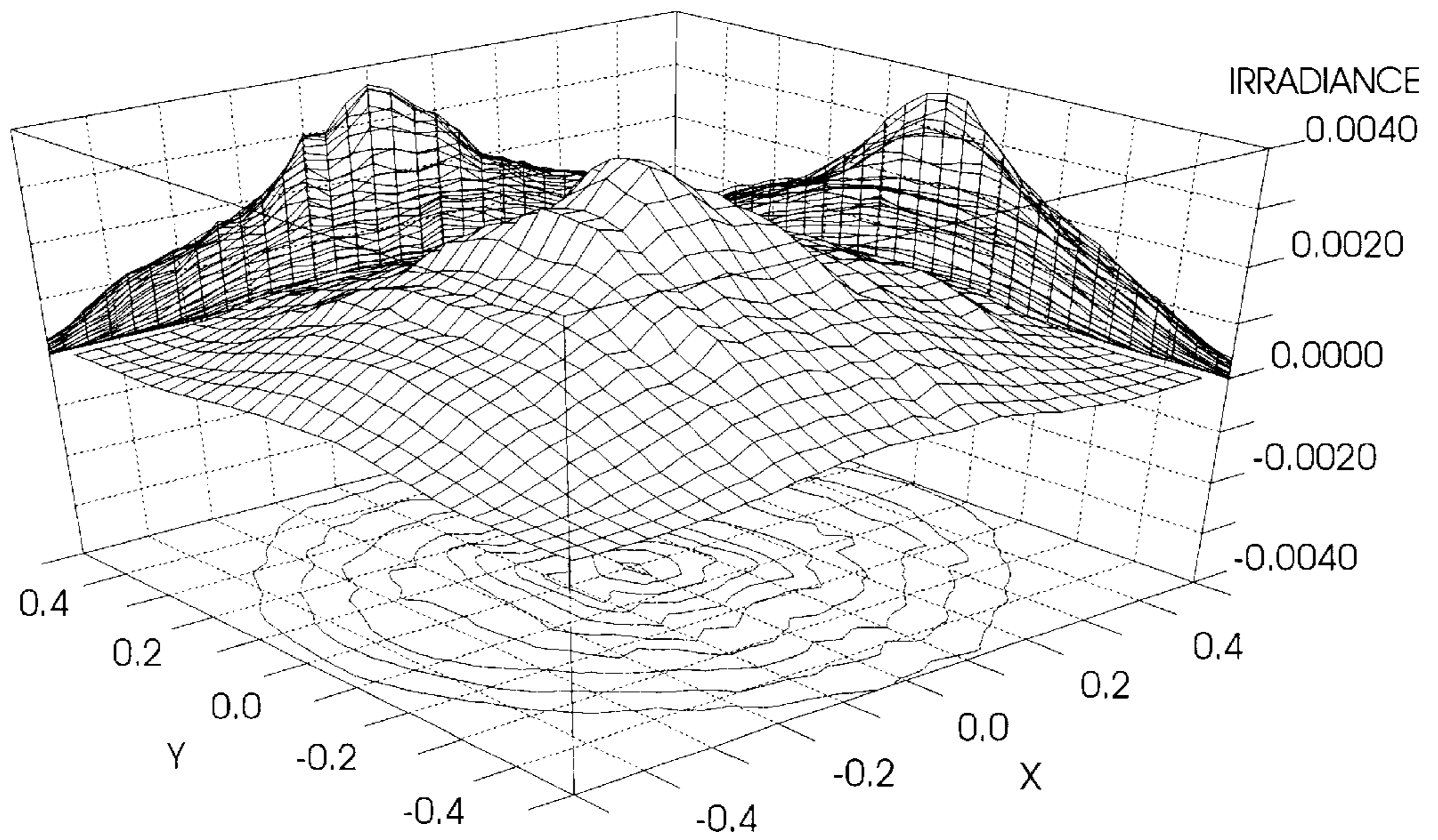
Irradiance in Projection Lens Input Plane
