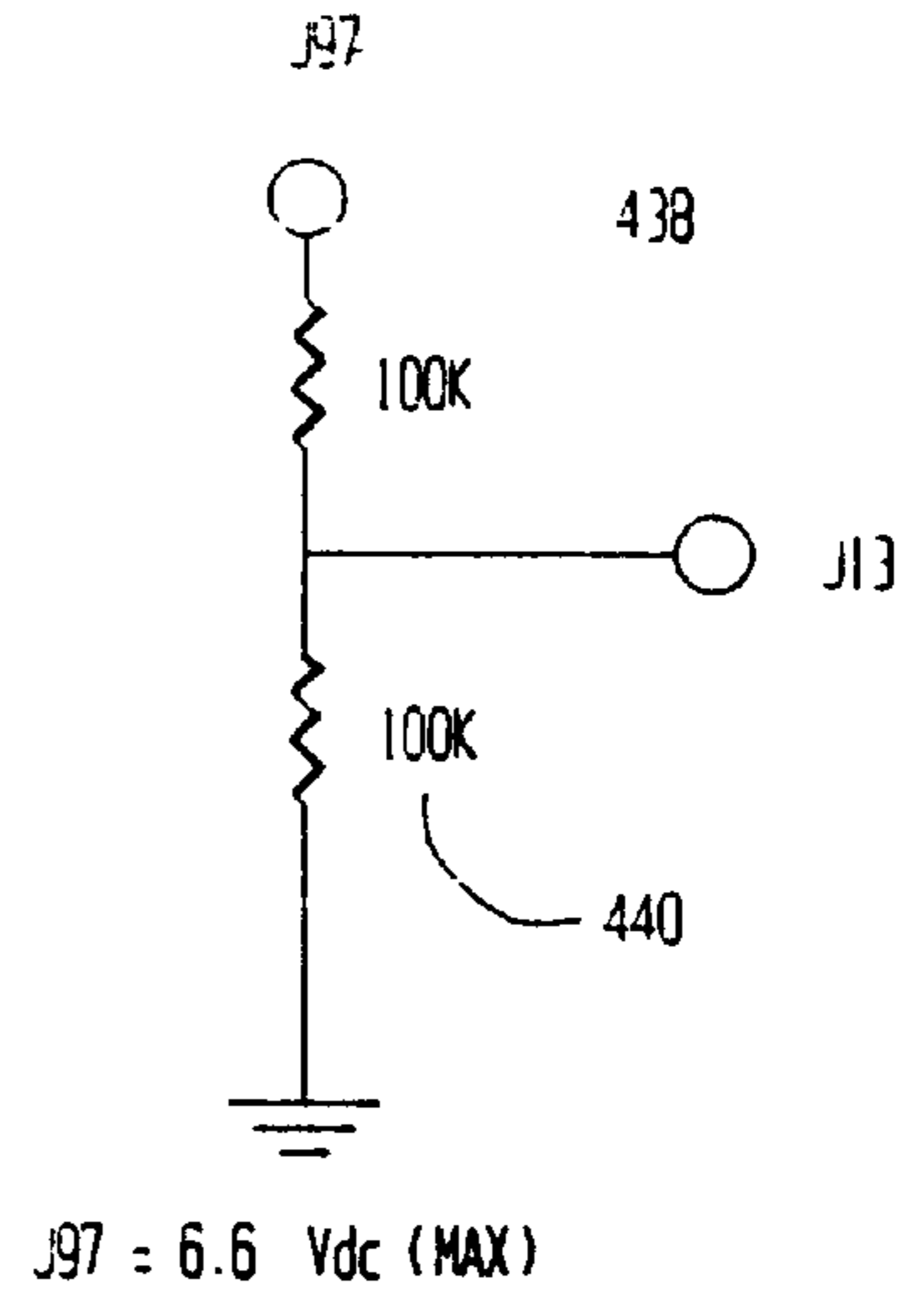
FIG. 33 MAIN BATTERY VOLTAGE 436
