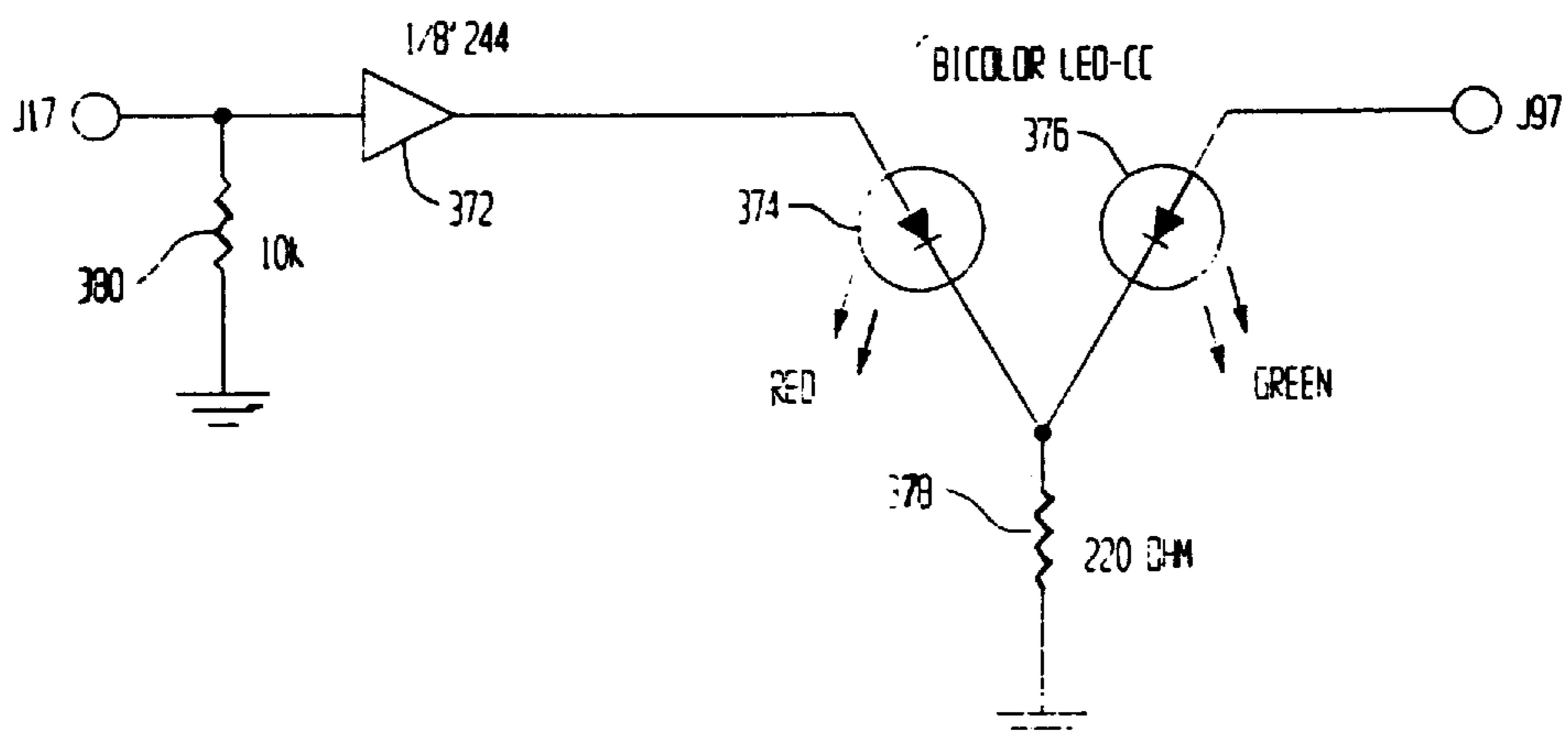
FIG. 26 HARDWARE STATUS LED 370
