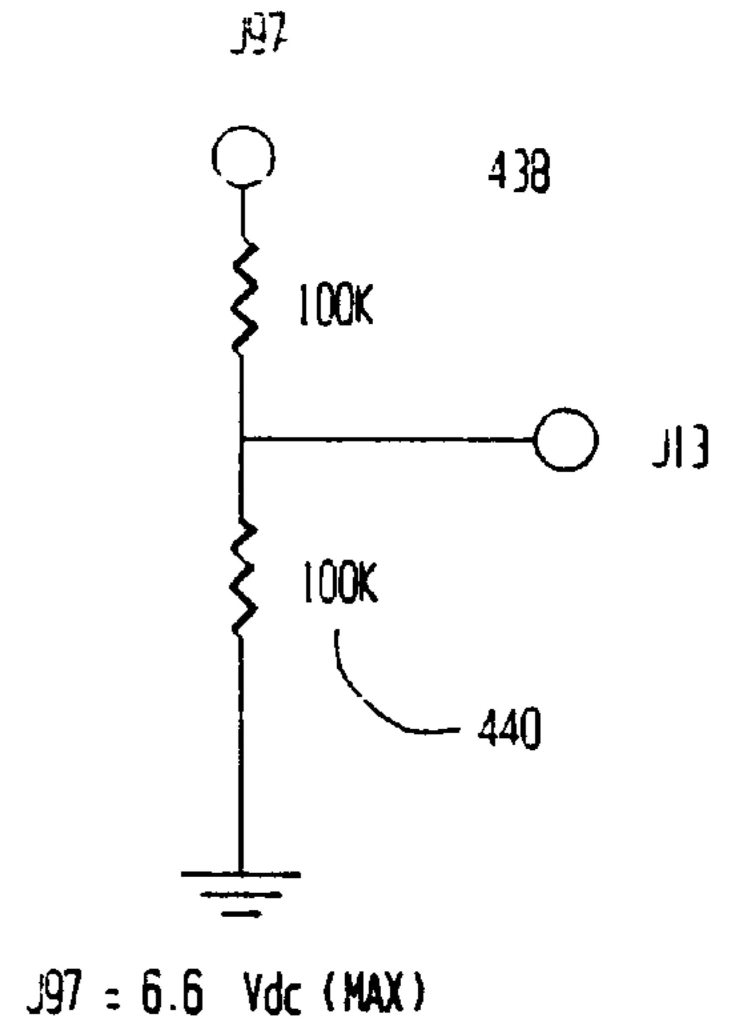
FIG. 33 MAIN BATTERY VOLTAGE 436
