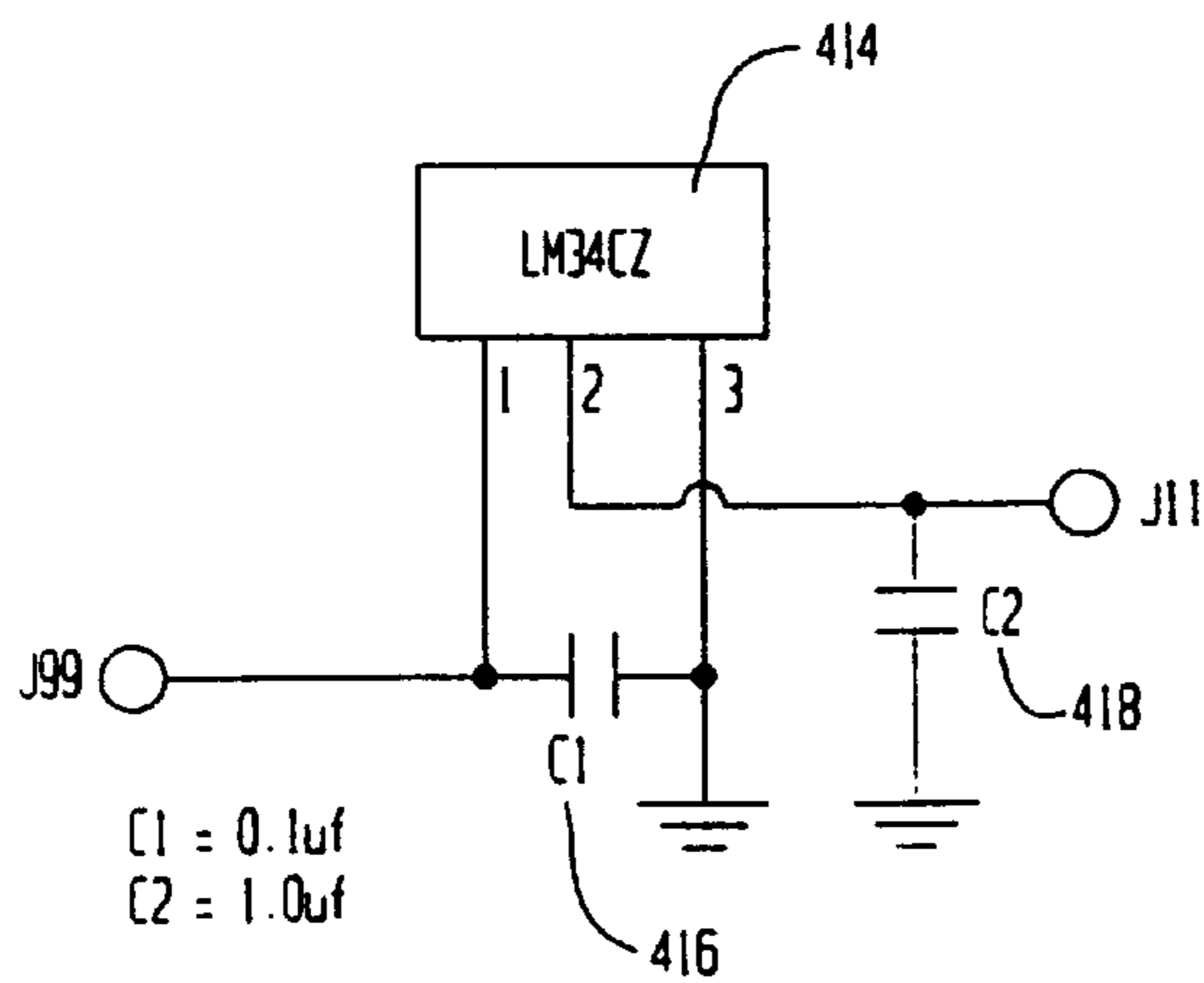
FIG. 30 TEMPERATURE SENSOR: LM34CZ (-40°F TO +230°F) 412
