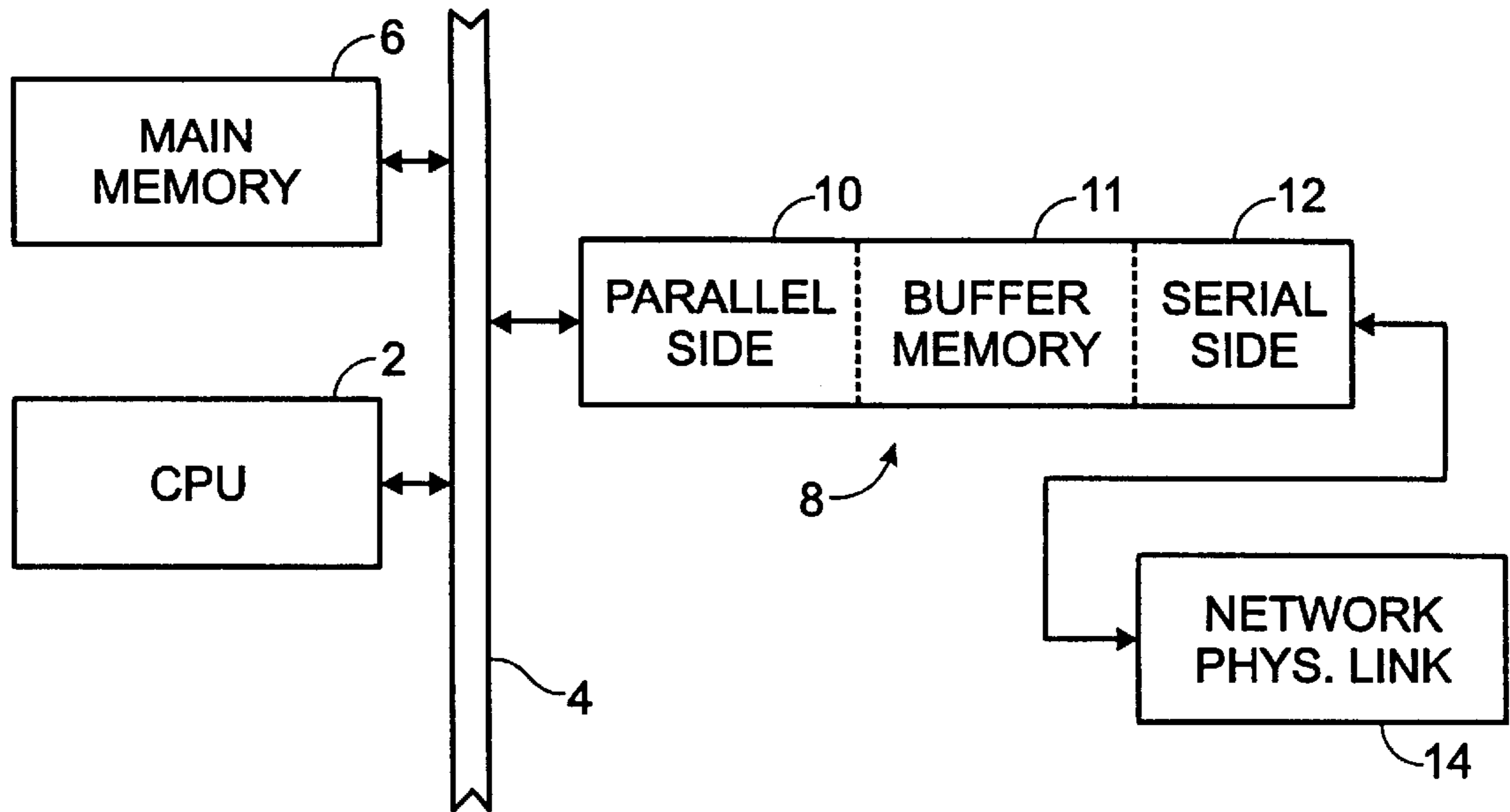
Fig. 1 (PRIOR ART)
