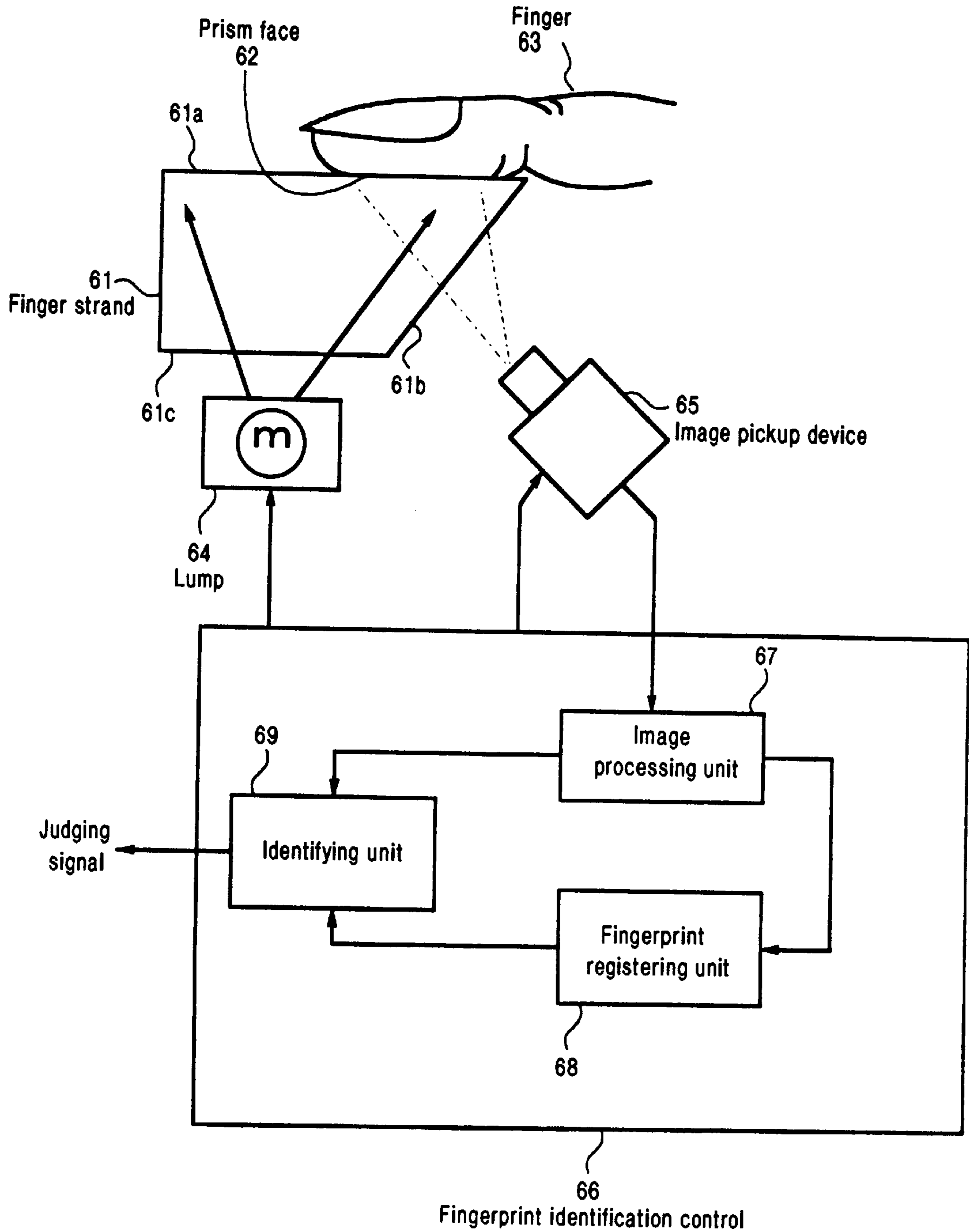
FIG. 18 PRIOR ART
