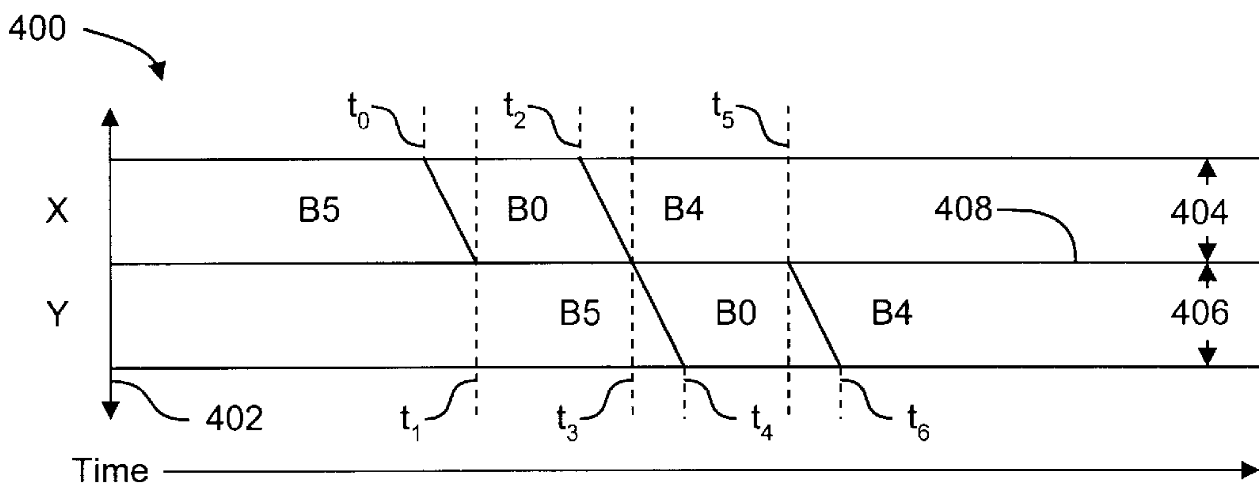
FIG. 4 Prior Art
