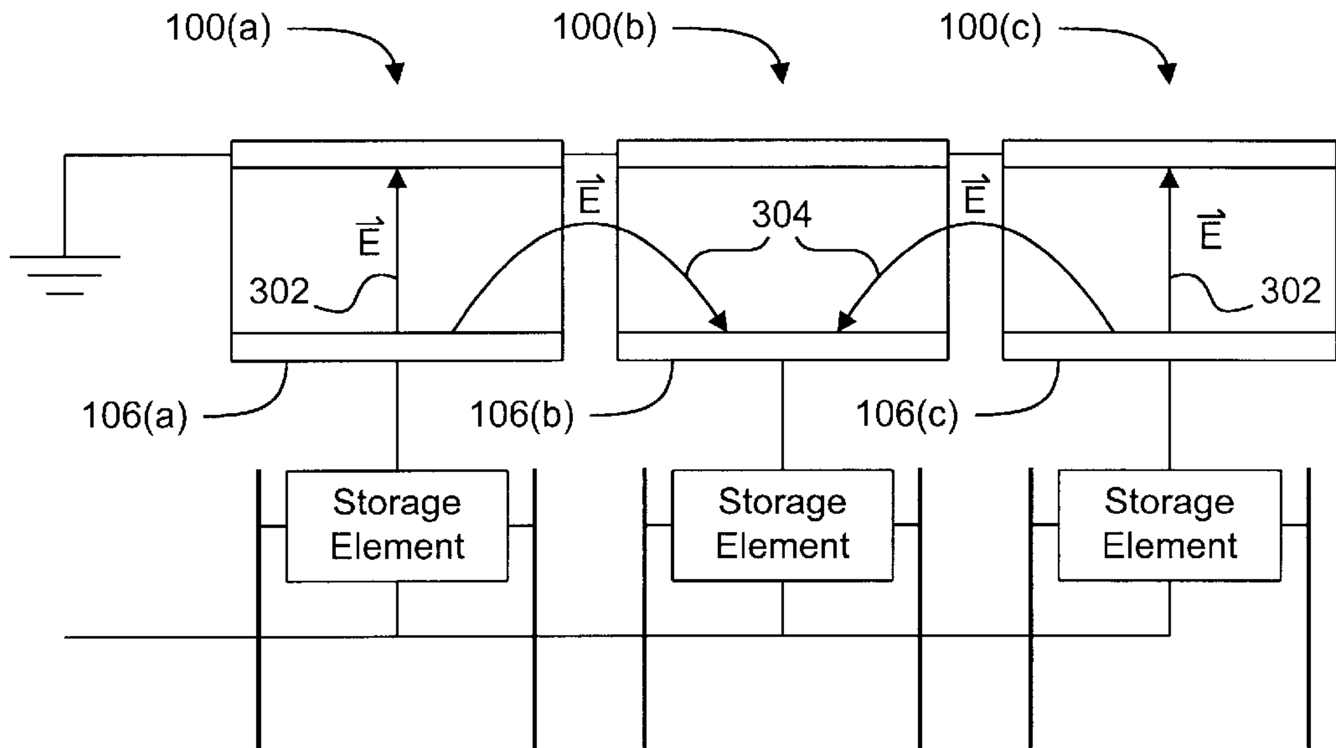
FIG. 3 Prior Art
