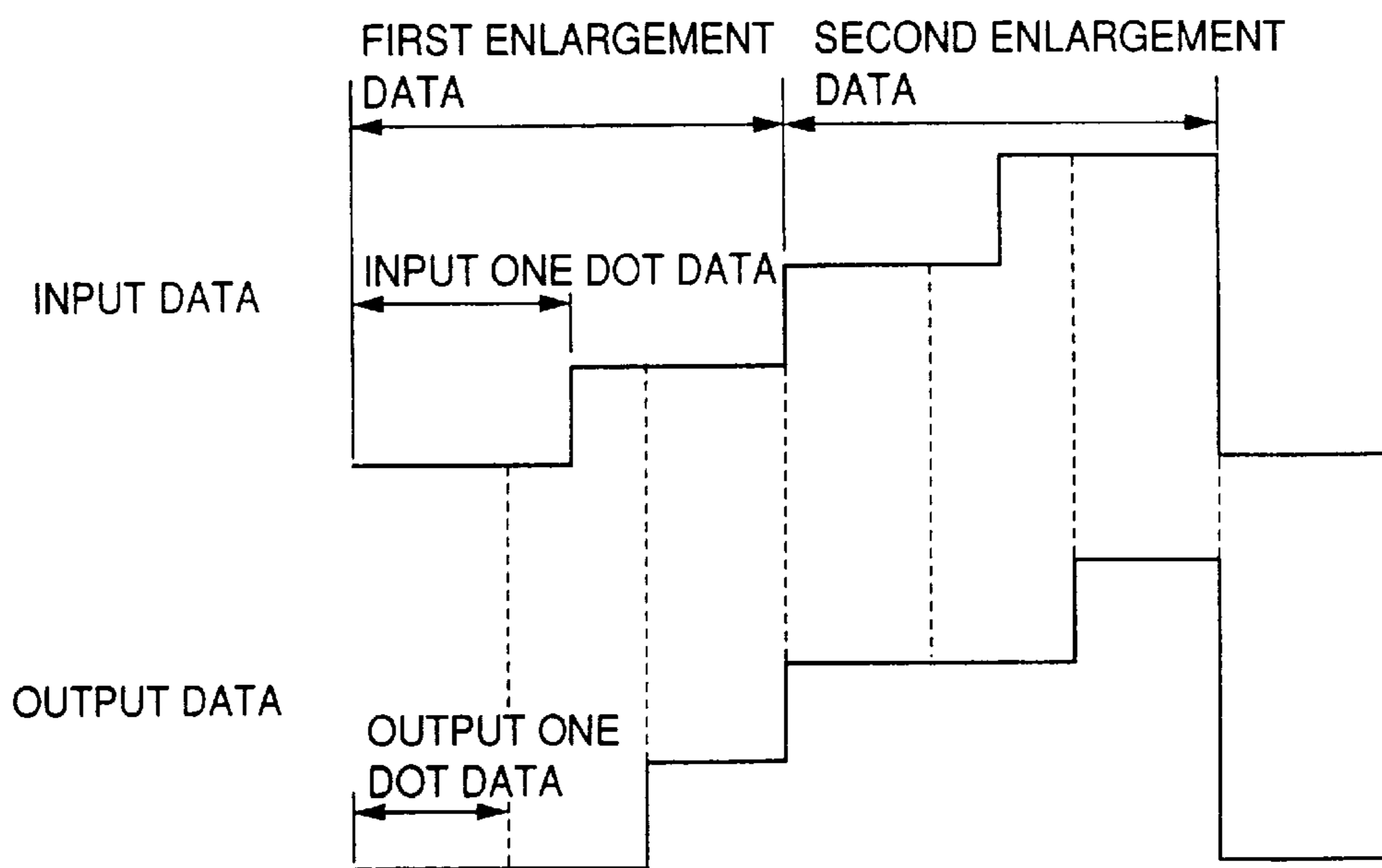
SIMPLE ENLARGEMENT METHOD (2→3)
