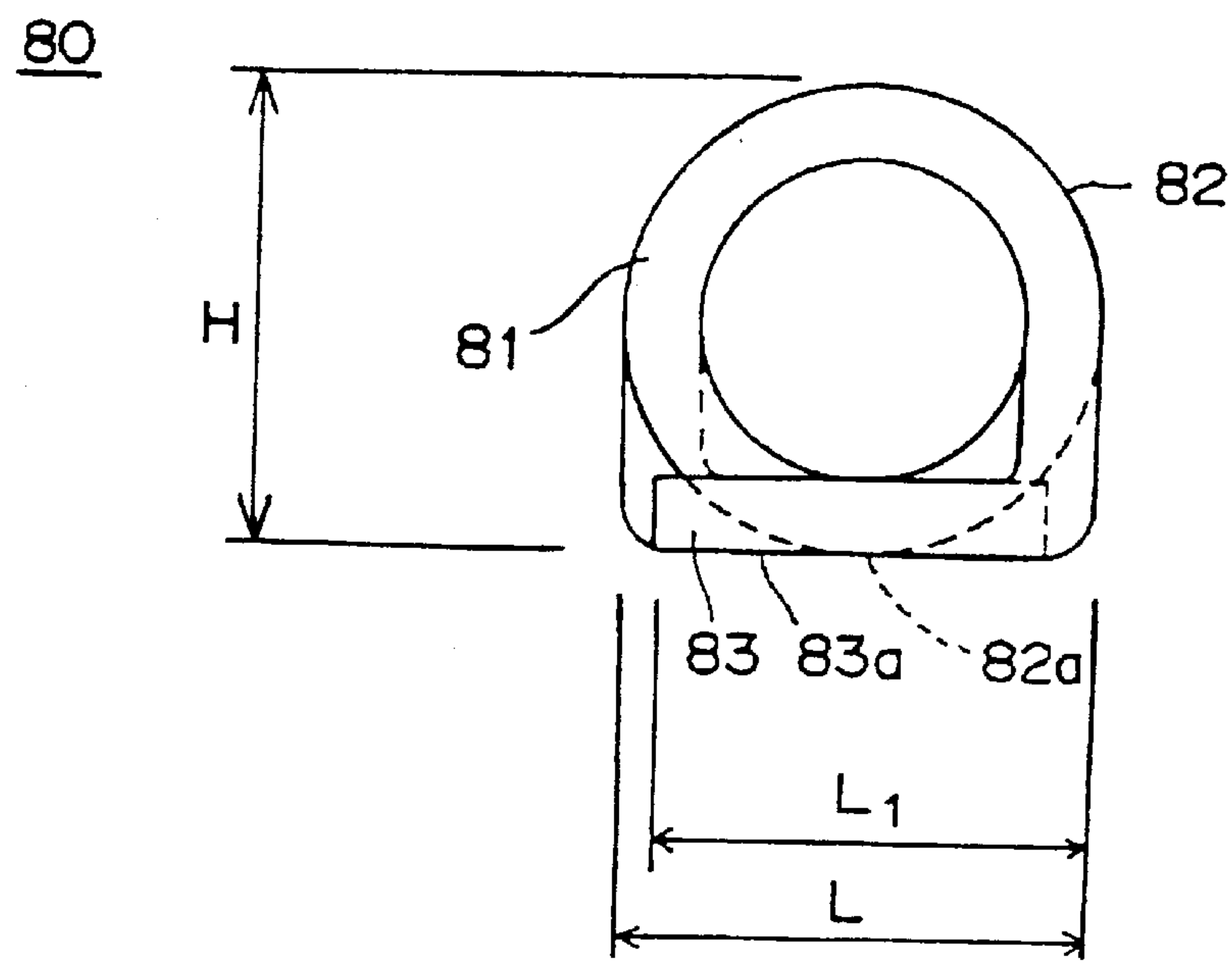
FIG. 12 PRIOR ART
