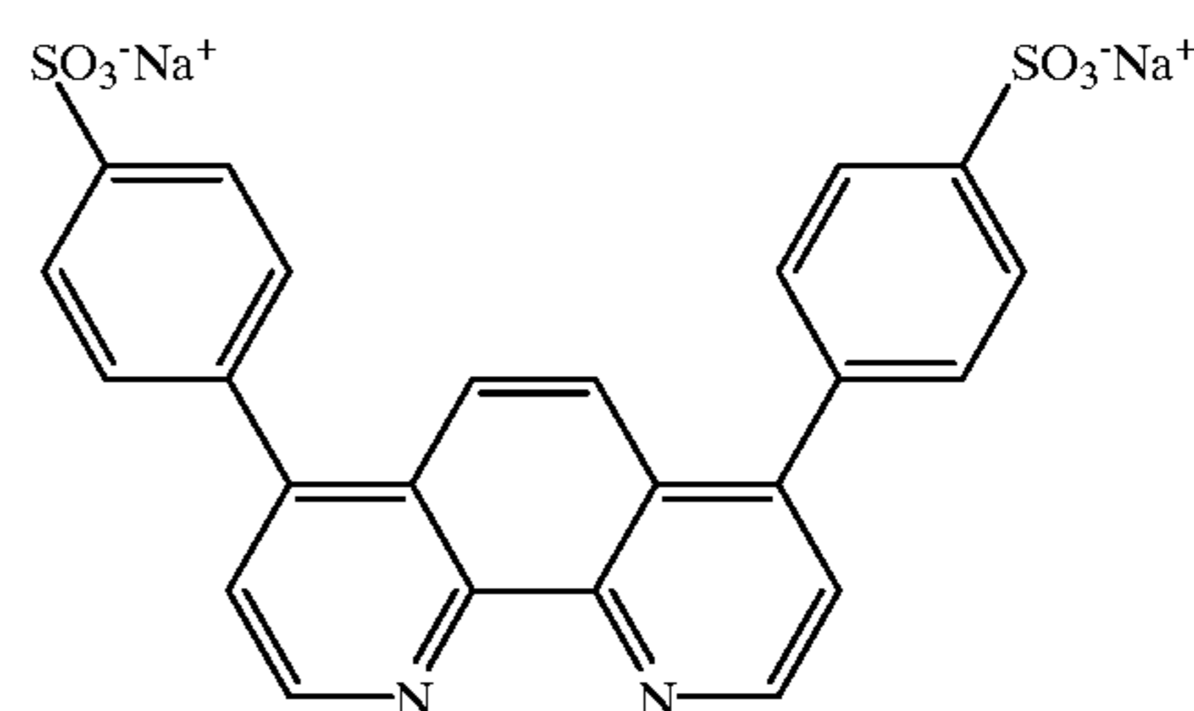
Bathophenanthroline
