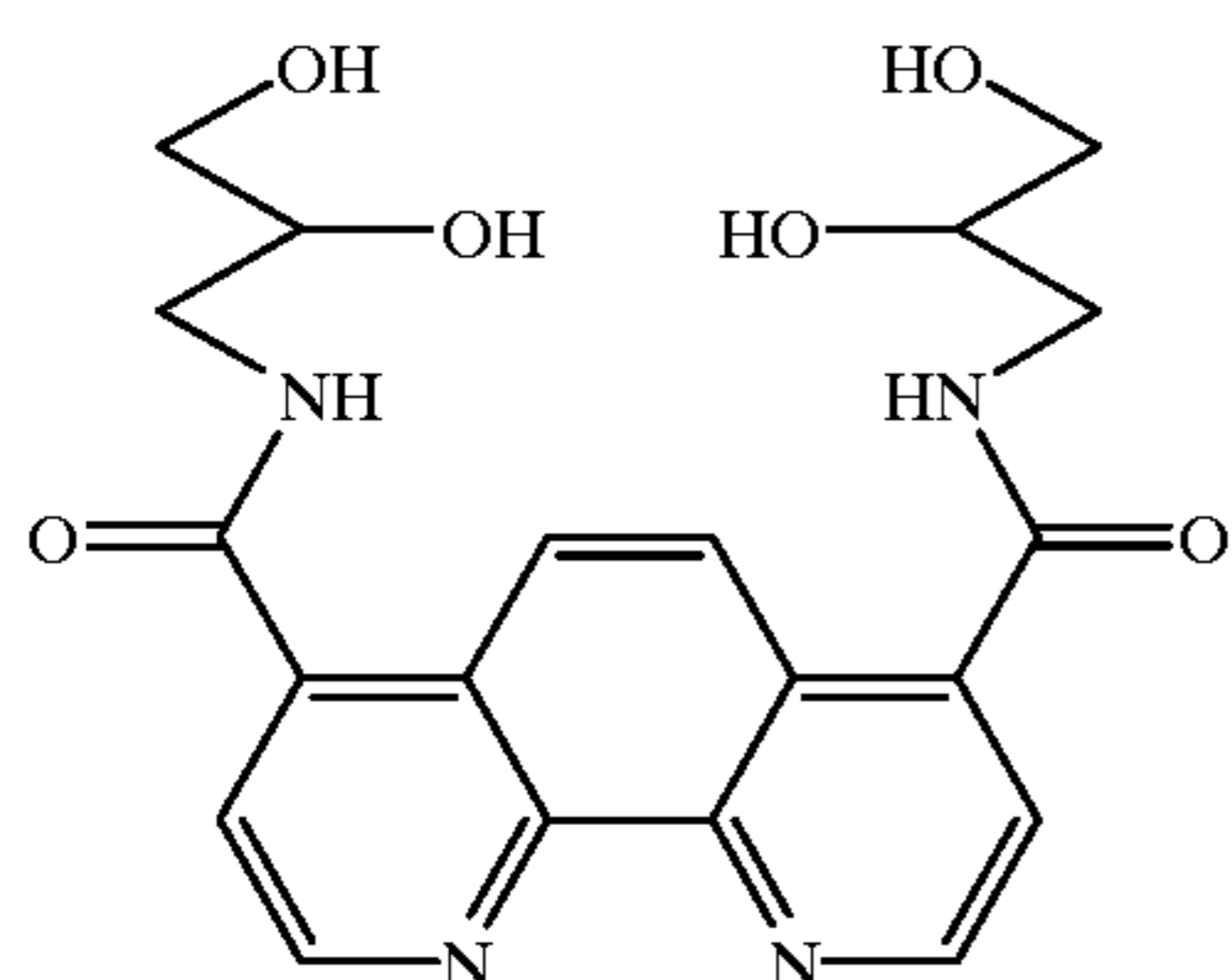
4,7-bis(2,3-dihydroxypropylcarboxamido)-1,10-phenanthroline
