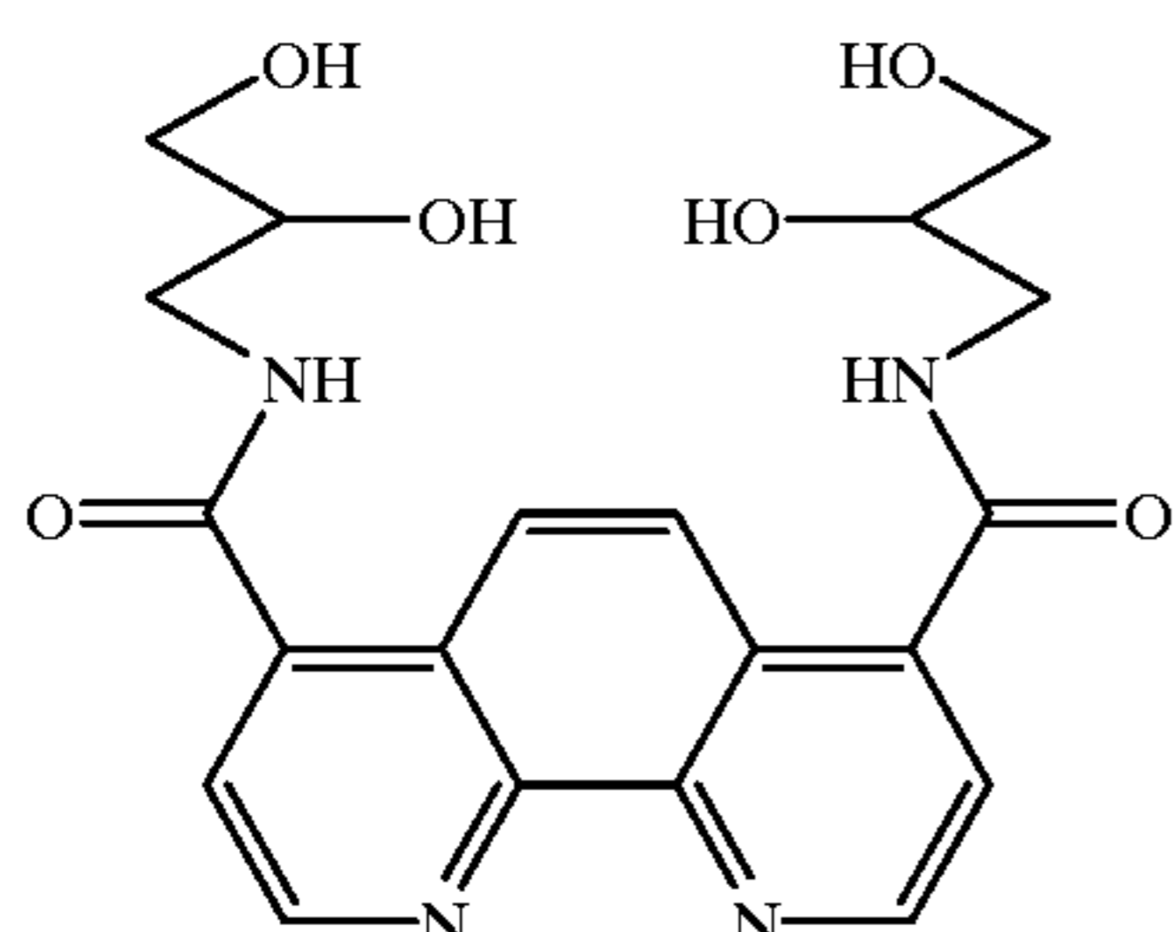
4,7-bis(2,3-dihydroxypropylcarboxamido)-1,10-phenanthroline
