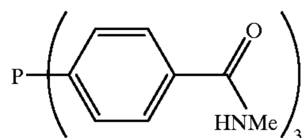
tris(N-methylcarboxamidophenyl)phosphine
