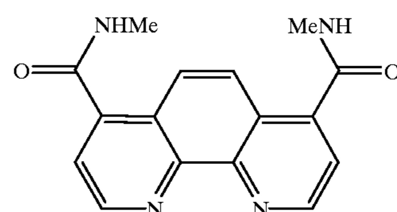
4,7-di-N-methylcarboxamido-1,10-phenanthroline
