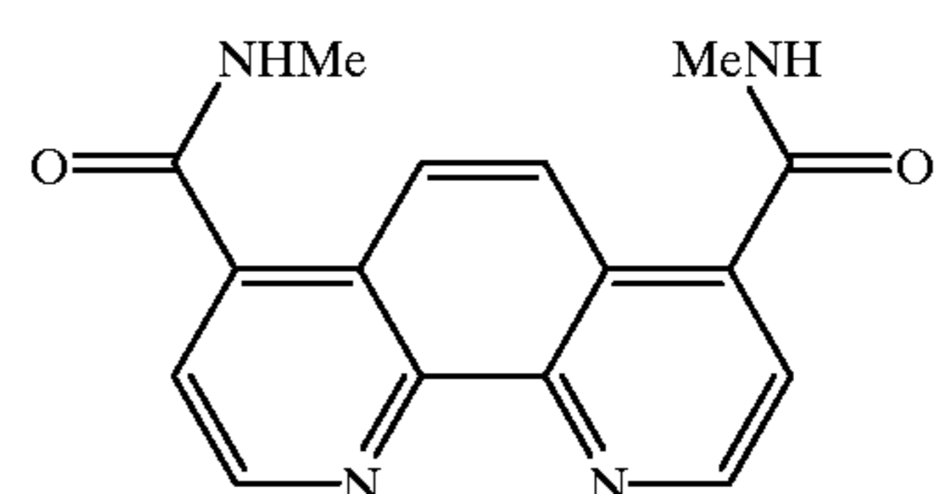
4,7-di-N-methylcarboxamido-1,10-phenanthroline
