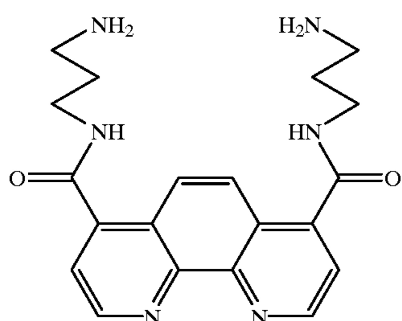
4,7-di-(N-(3-aminopropyl)carboxamido)-1,10-phenanthroline
