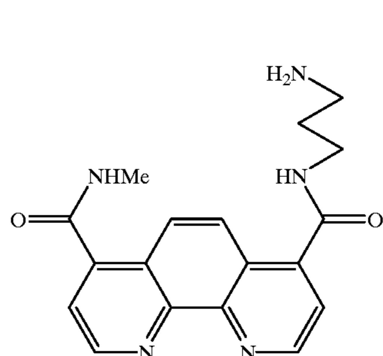
4-N-(3-aminopropyl)carboxamido-7-N-methylcarboxamido-1,10-phenanthroline
