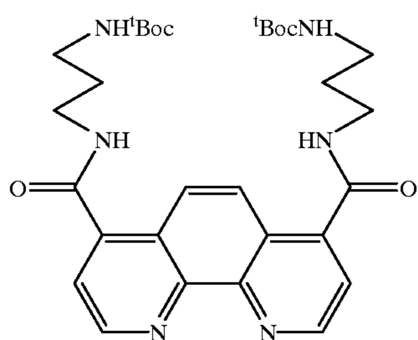
4,7-di-(N-(3-tert-butyloxycarboxamidopropyl)carboxamido)-1,10-phenanthroline
