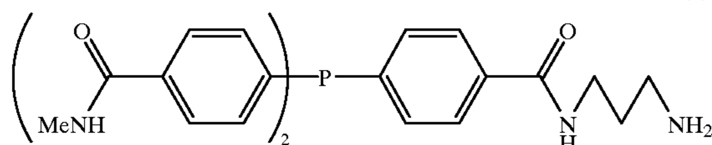
3-amino-N-propylcarboxamidophenyl-bis(N-methylcarboxamidophenyl)phosphine
