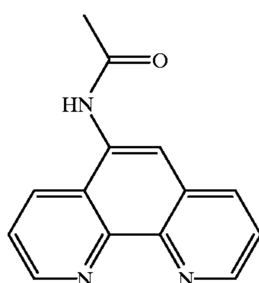
5-acetamido-1,10-phenanthroline
