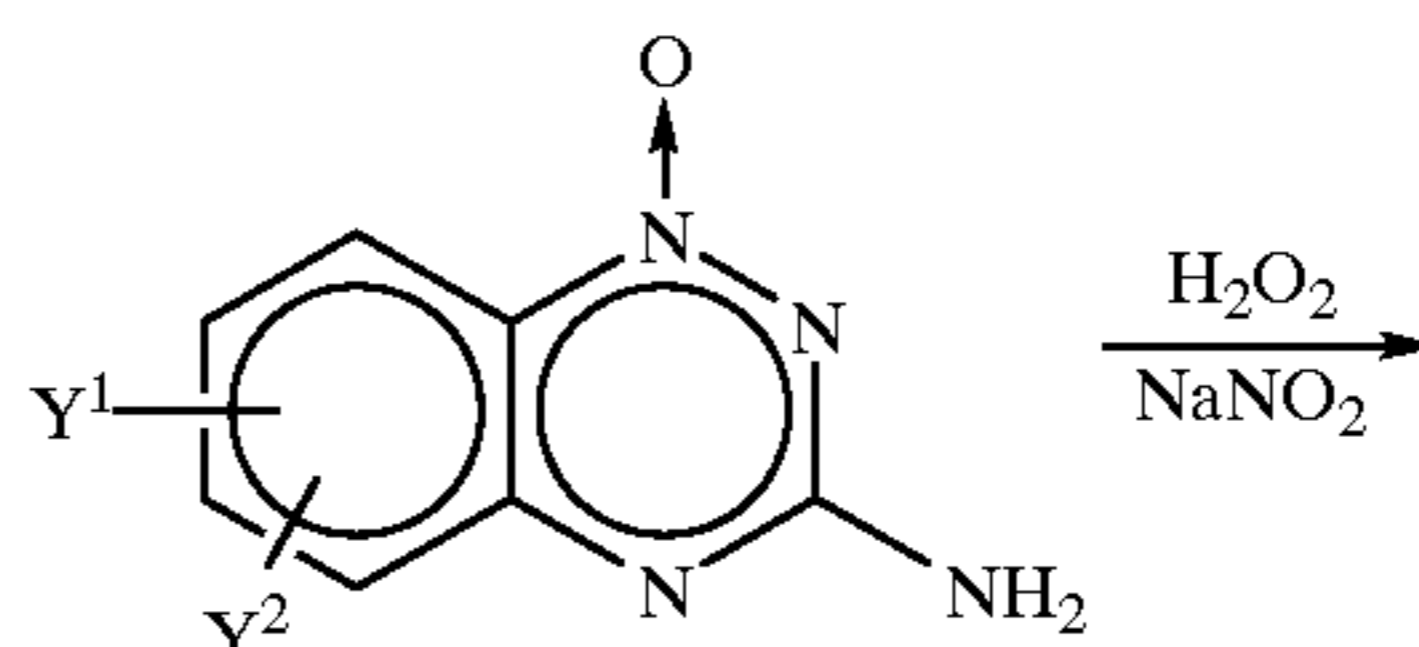
Scheme IV
