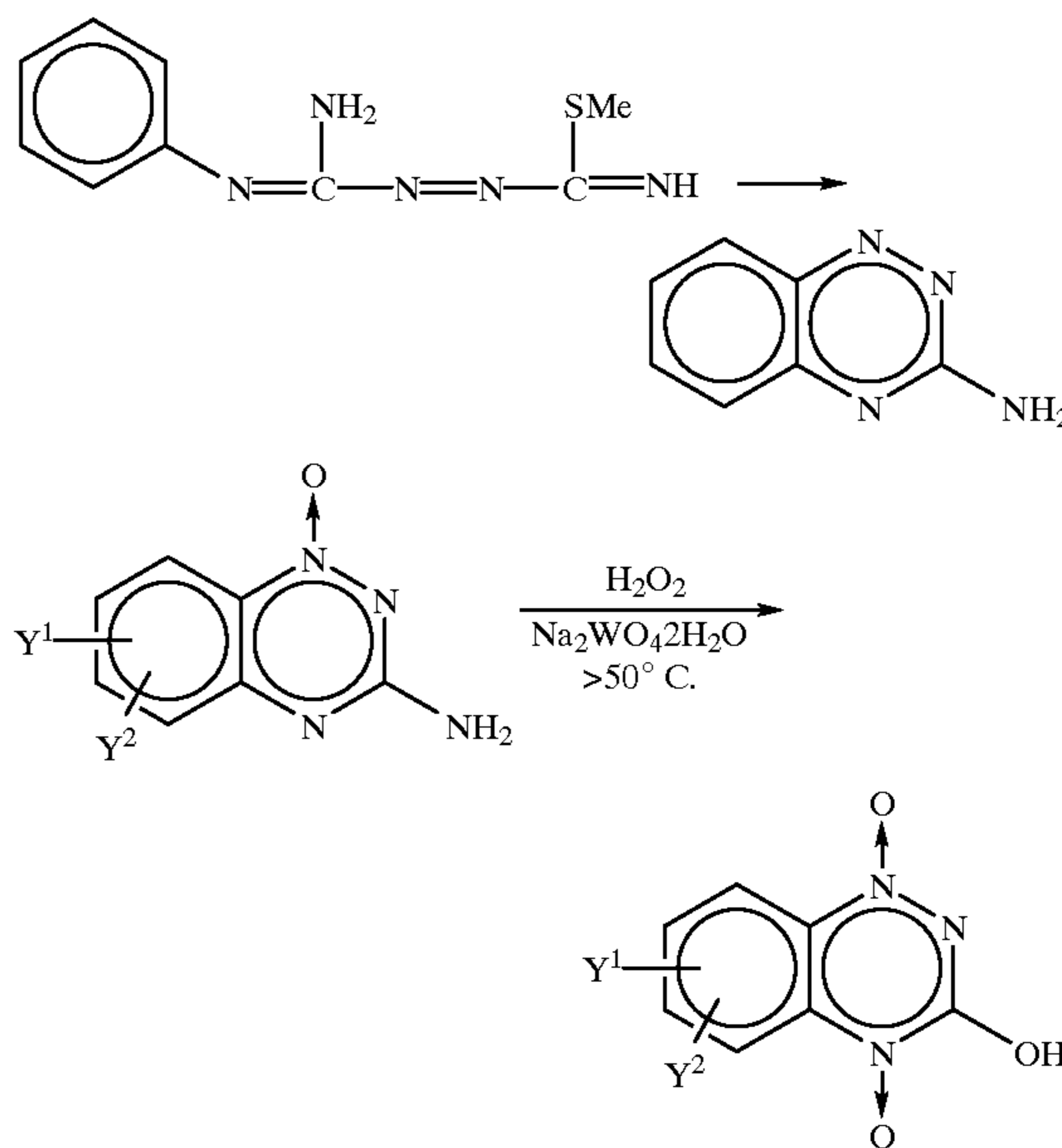
Scheme III
