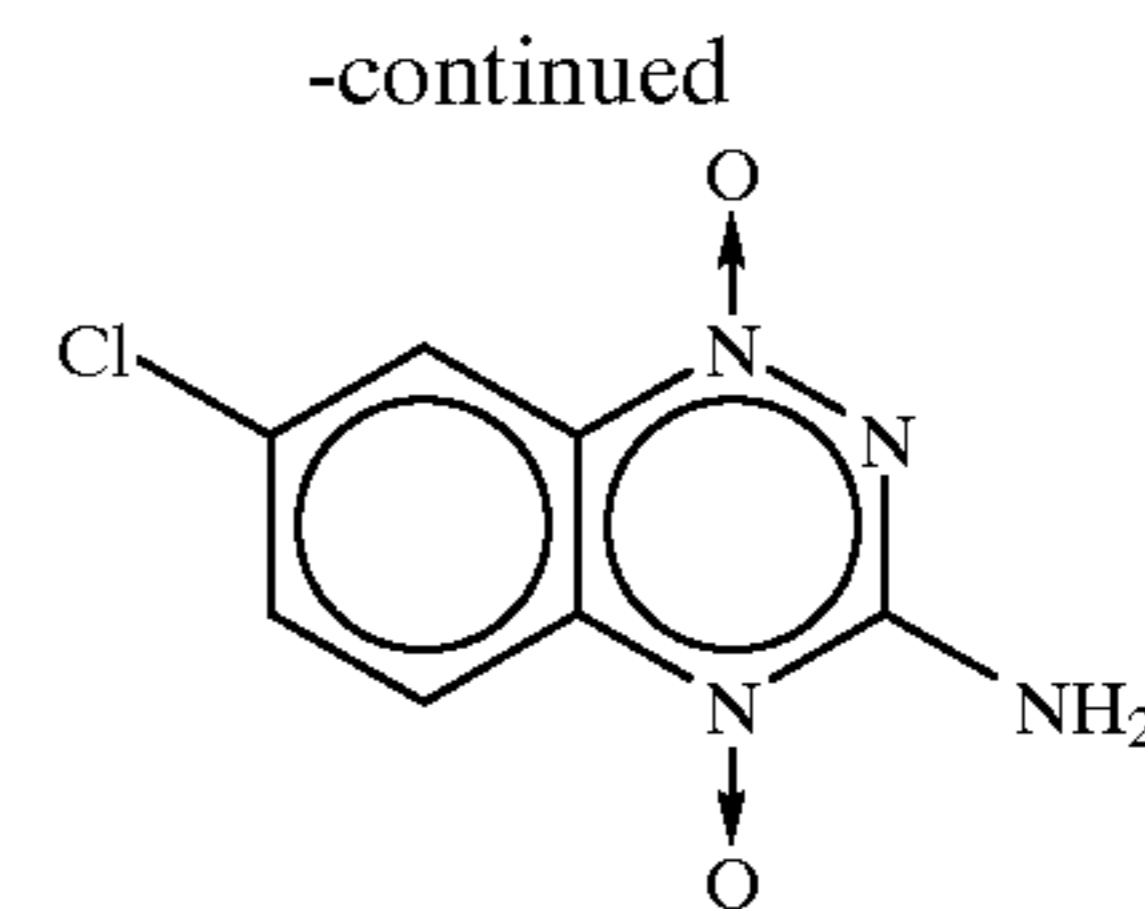
12 7-chloro-3-amino-1,2,4-benzotriazine 1,4-dioxide
