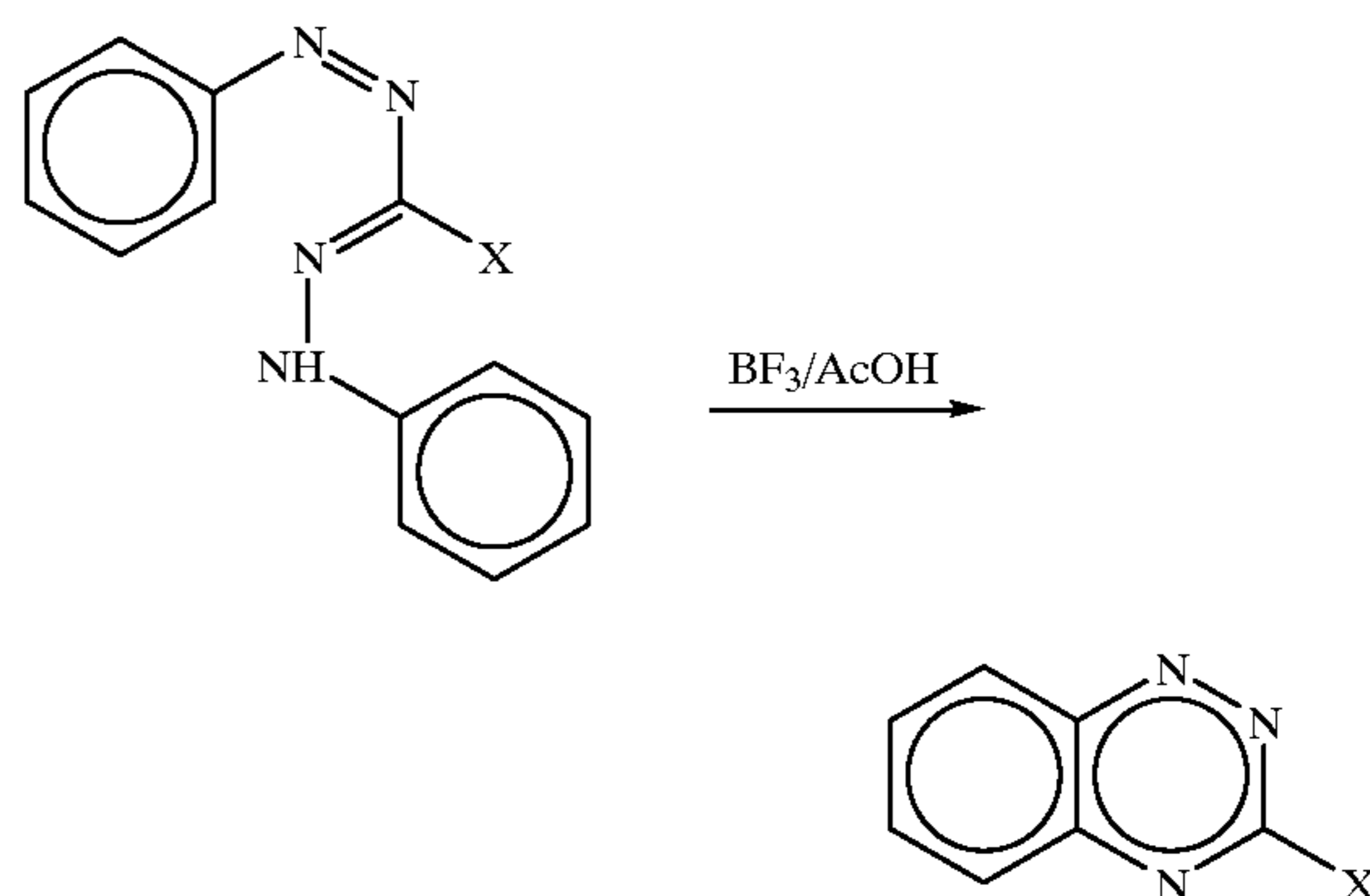
Scheme II
