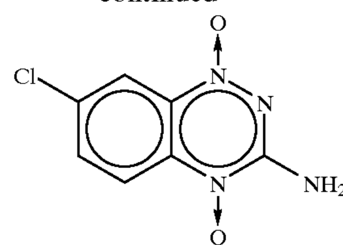
12 7-chloro-3-amino-1,2,4-benzotriazine 1,4-dioxide
