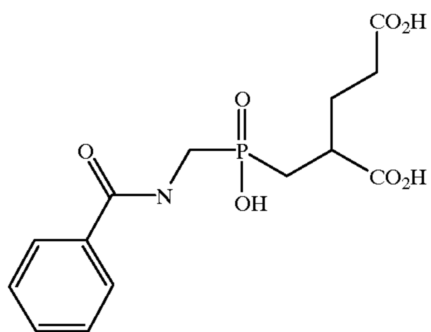
2-[(Phenylcarboxamido)methyl]hydroxyphosphinylmethyl]pentanedioic acid (8);
