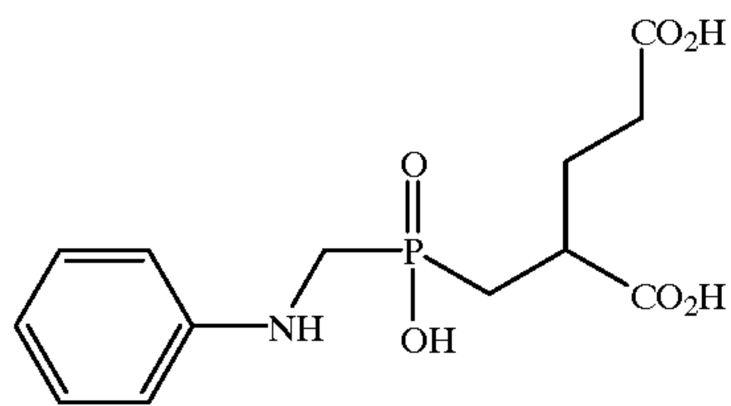
2-[(Phenylamino)methyl]hydroxyphosphinylmethyl]pentanedioic acid (7);
