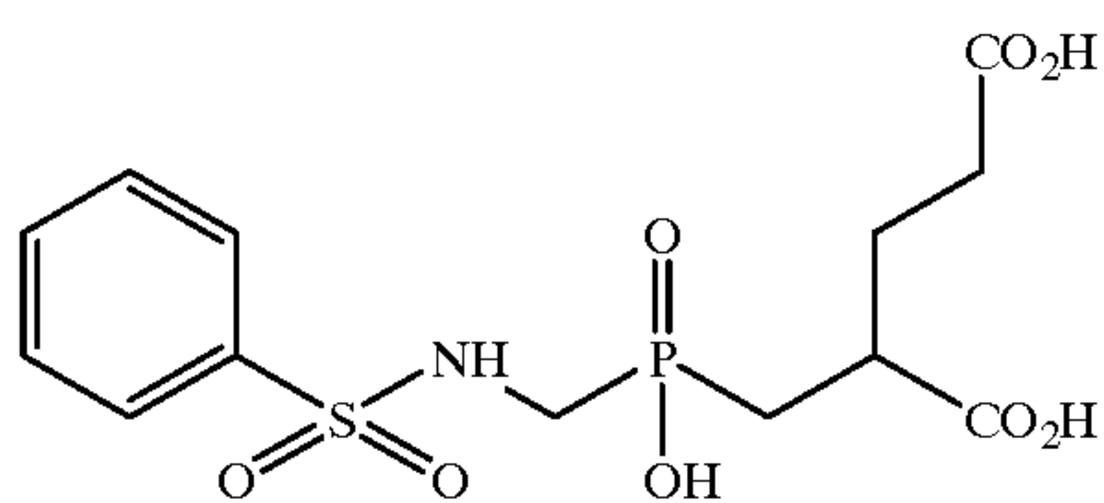
2-[(Phenylsulfonamido)methyl]hydroxyphosphinylmethyl]pentanedioic acid (9);
