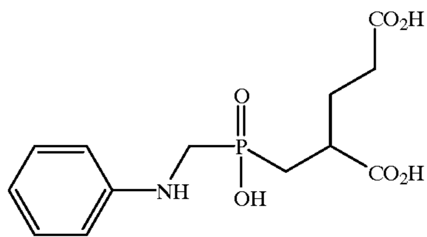
2-[(Phenylamino)methyl]hydroxyphosphinylmethyl]pentanedioic acid (7);
