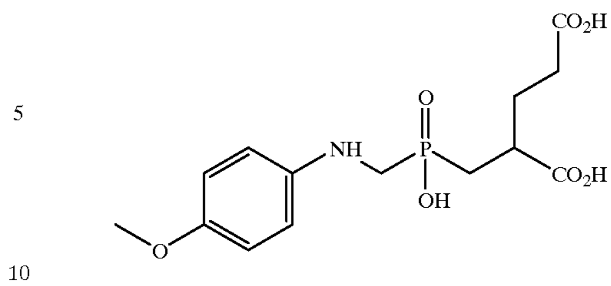
2-[(4-Methoxyphenyl)amino]methyl]hydroxyphosphinylmethyl]pentanedioic acid (11);
