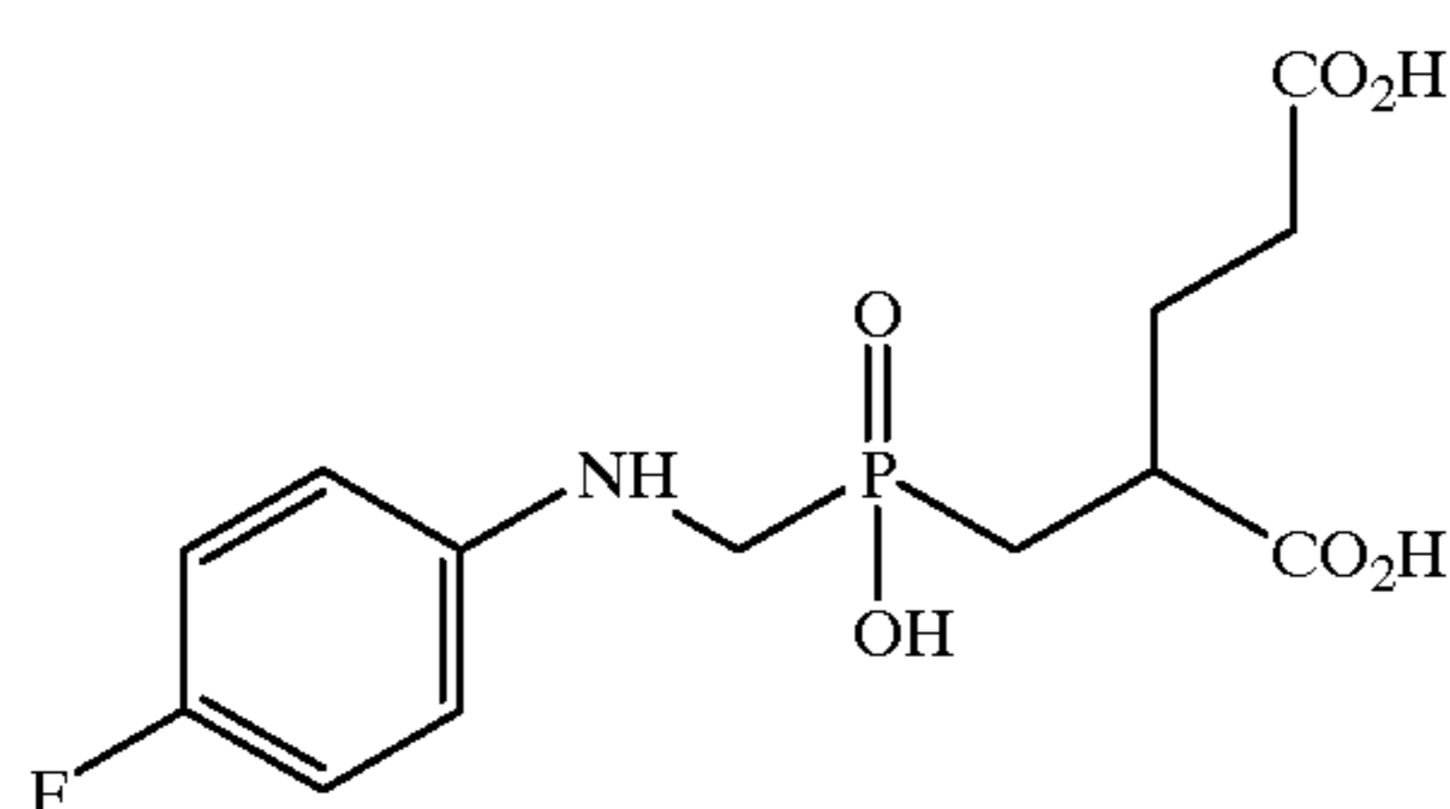
2-[(4-Fluorophenyl)amino]methyl]hydroxyphosphinylmethyl]pentanedioic acid (10);
