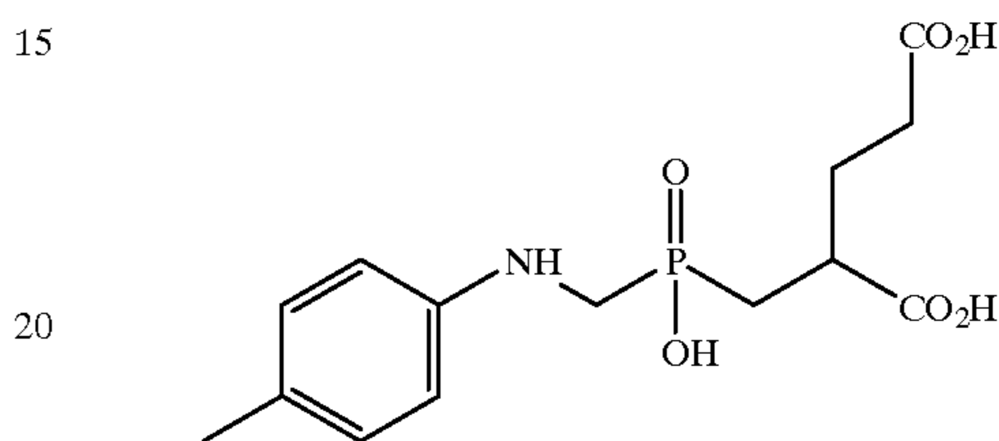
2-[(4-Methylphenyl)amino]methyl]hydroxyphosphinylmethyl]pentanedioic acid (12);
