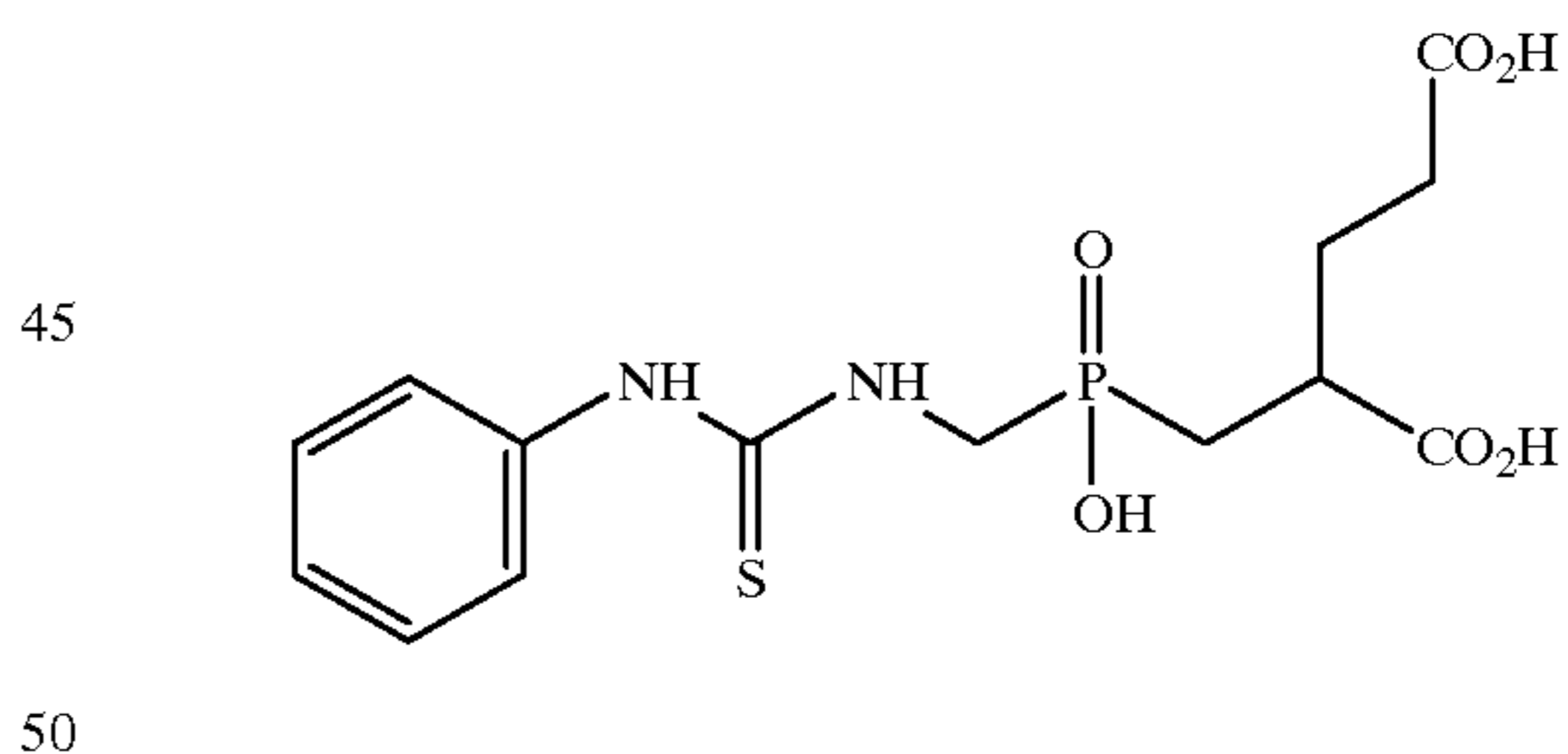
2-[(Thioformanilido)amino]benzyl]hydroxyphosphinylmethyl]pentanedioic acid (14).
