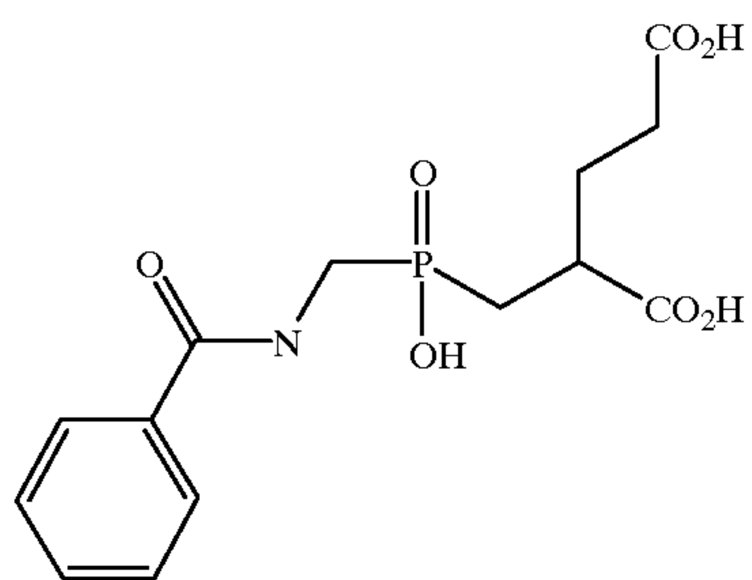
2-[(Phenylcarboxamido)methyl]hydroxyphosphinylmethyl]pentanedioic acid (8);
