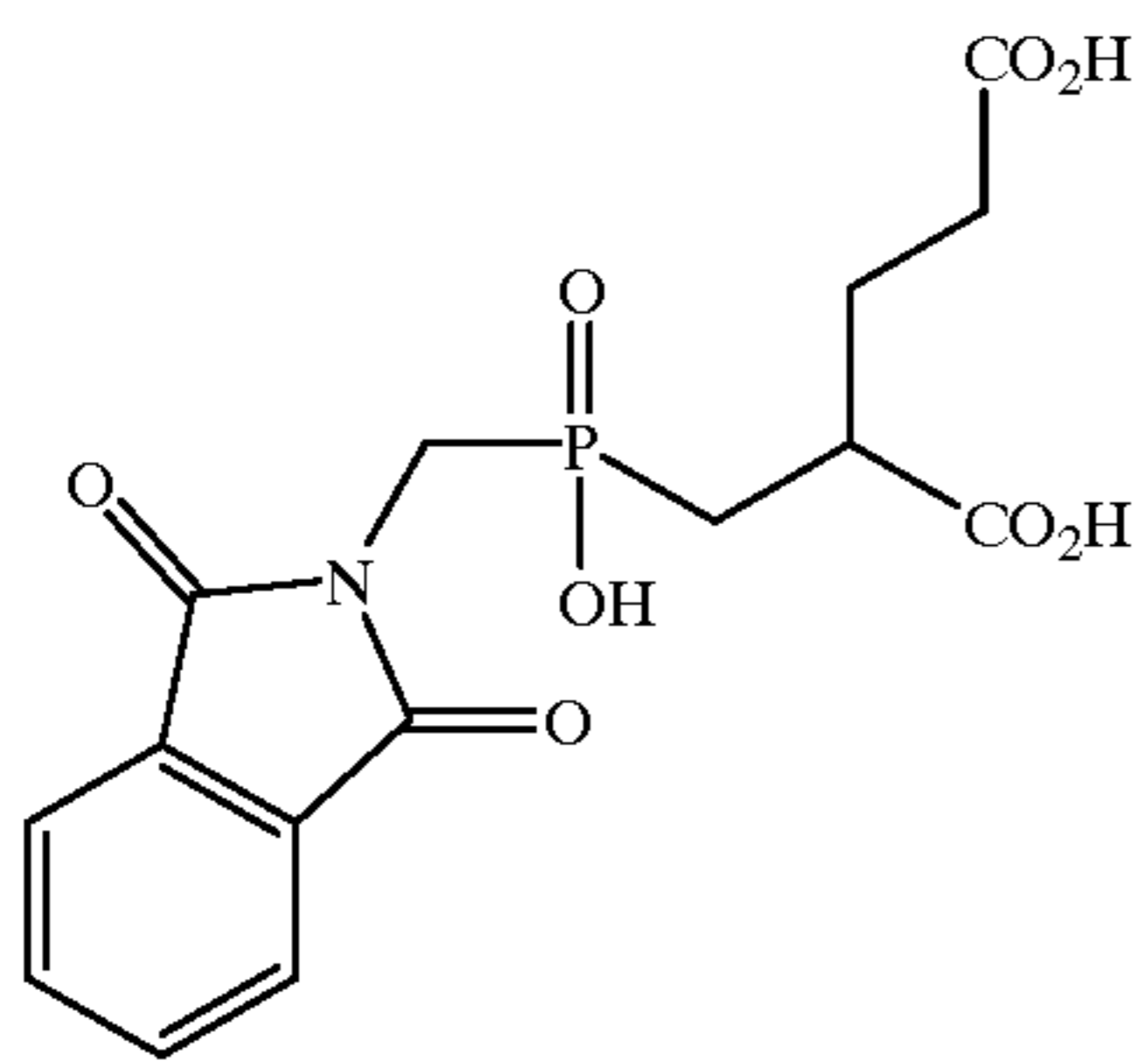
2-[(1,3-Dioxo-2,3-dihydro-1H-2-isoindolyl)methyl]hydroxyphosphinylmethyl]pentanedioic acid (6);
