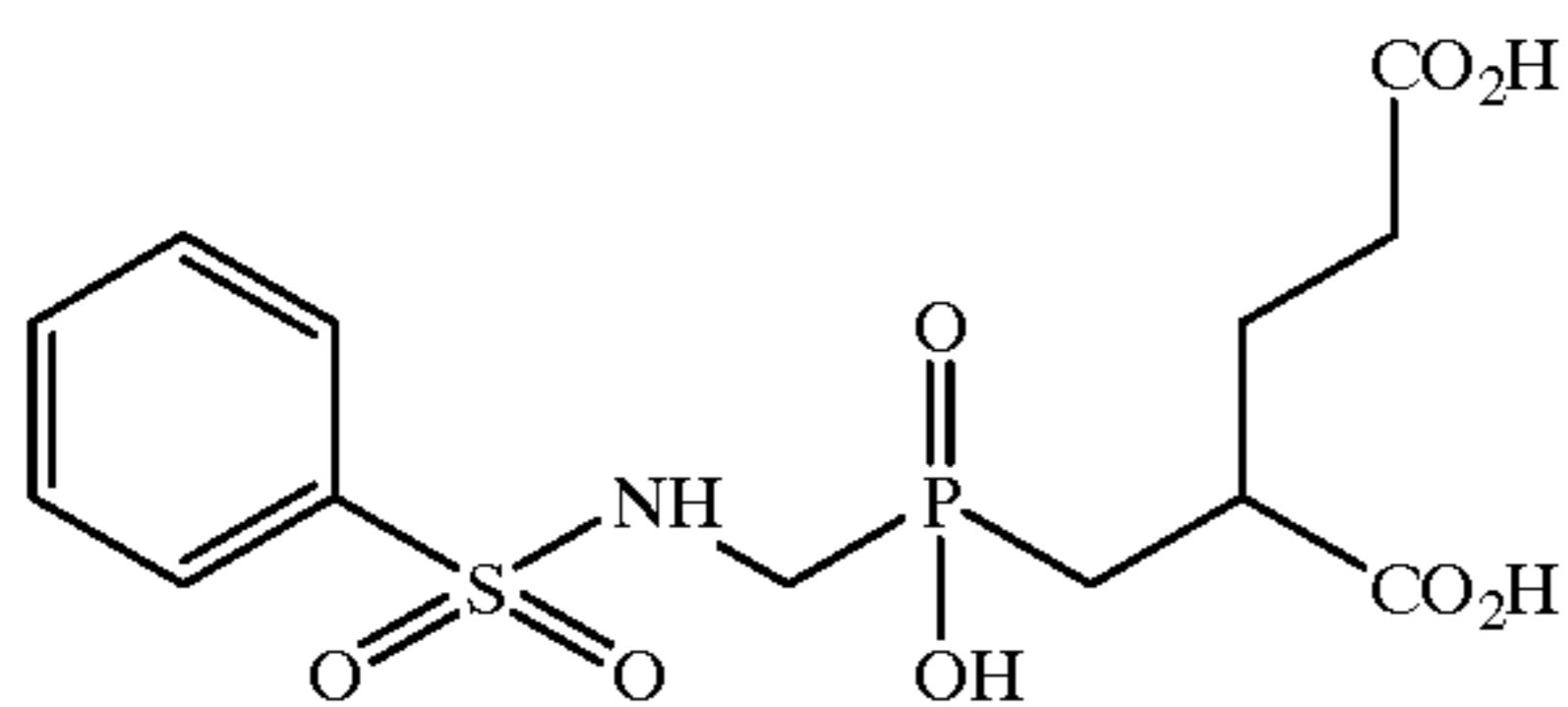
2-[(Phenylsulfonamido)methyl]hydroxyphosphinylmethyl]pentanedioic acid (9);
