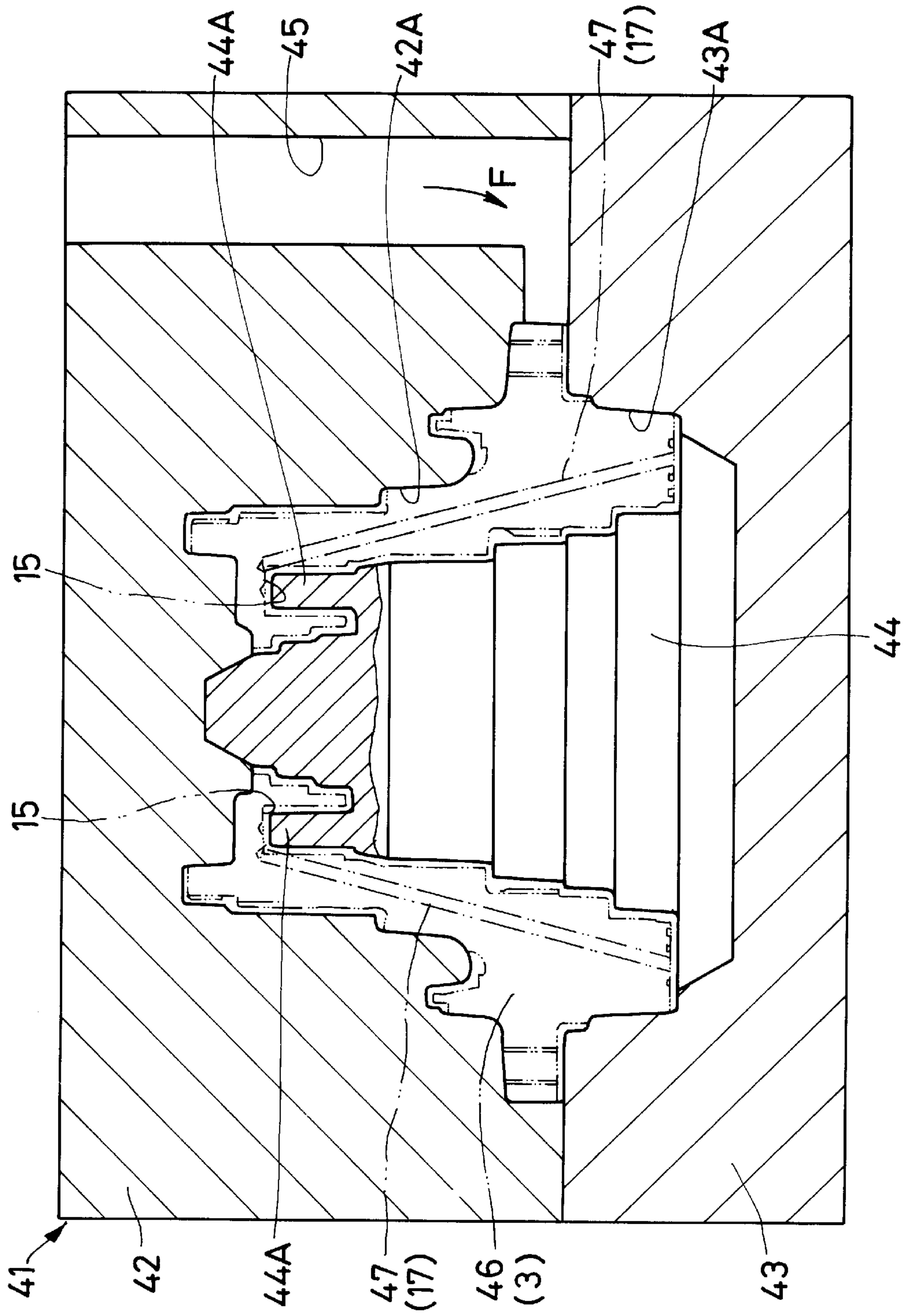
Fig. 9 PRIOR ART
