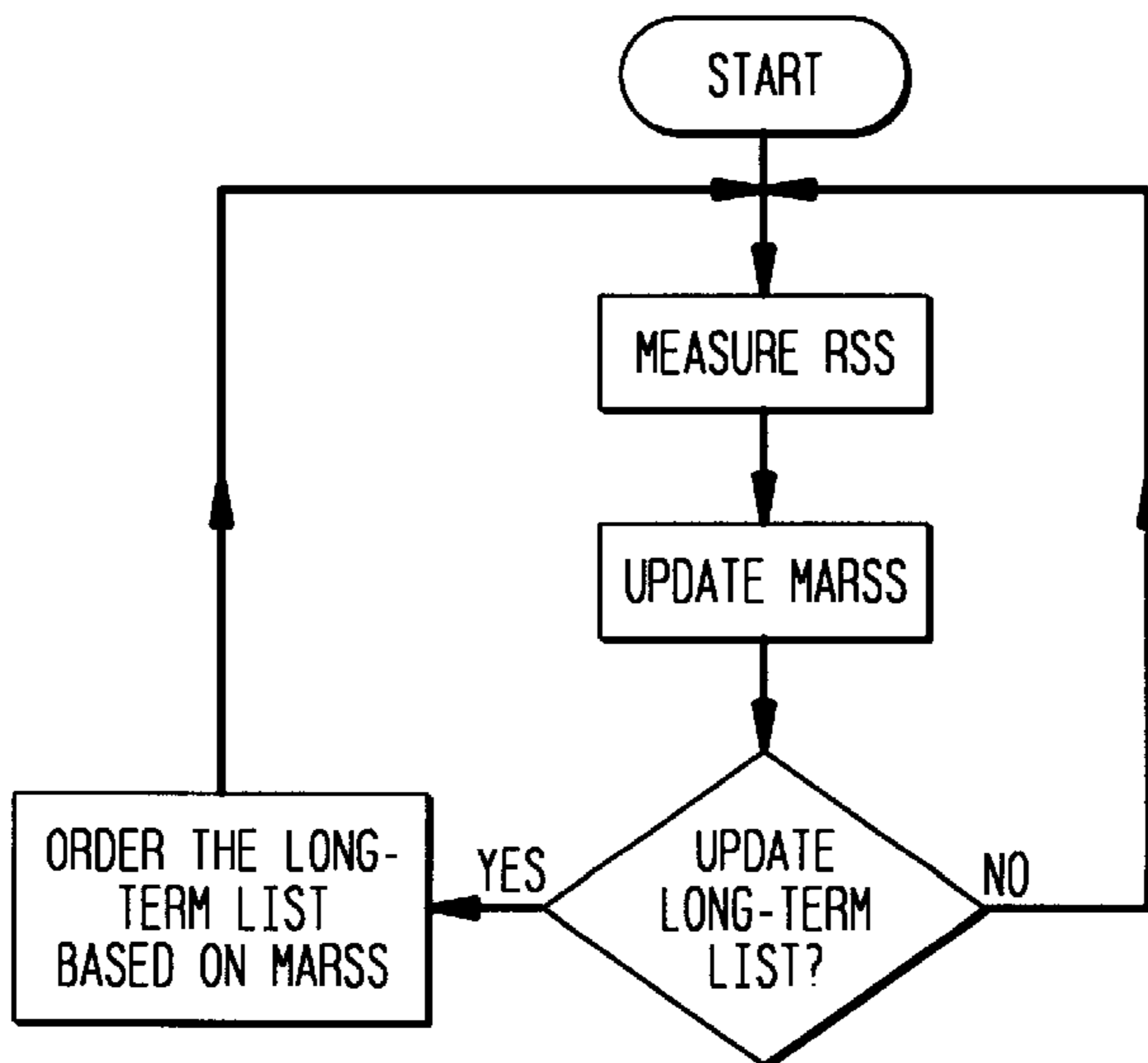
FIG. 8 LONG-TERM PROCESS
