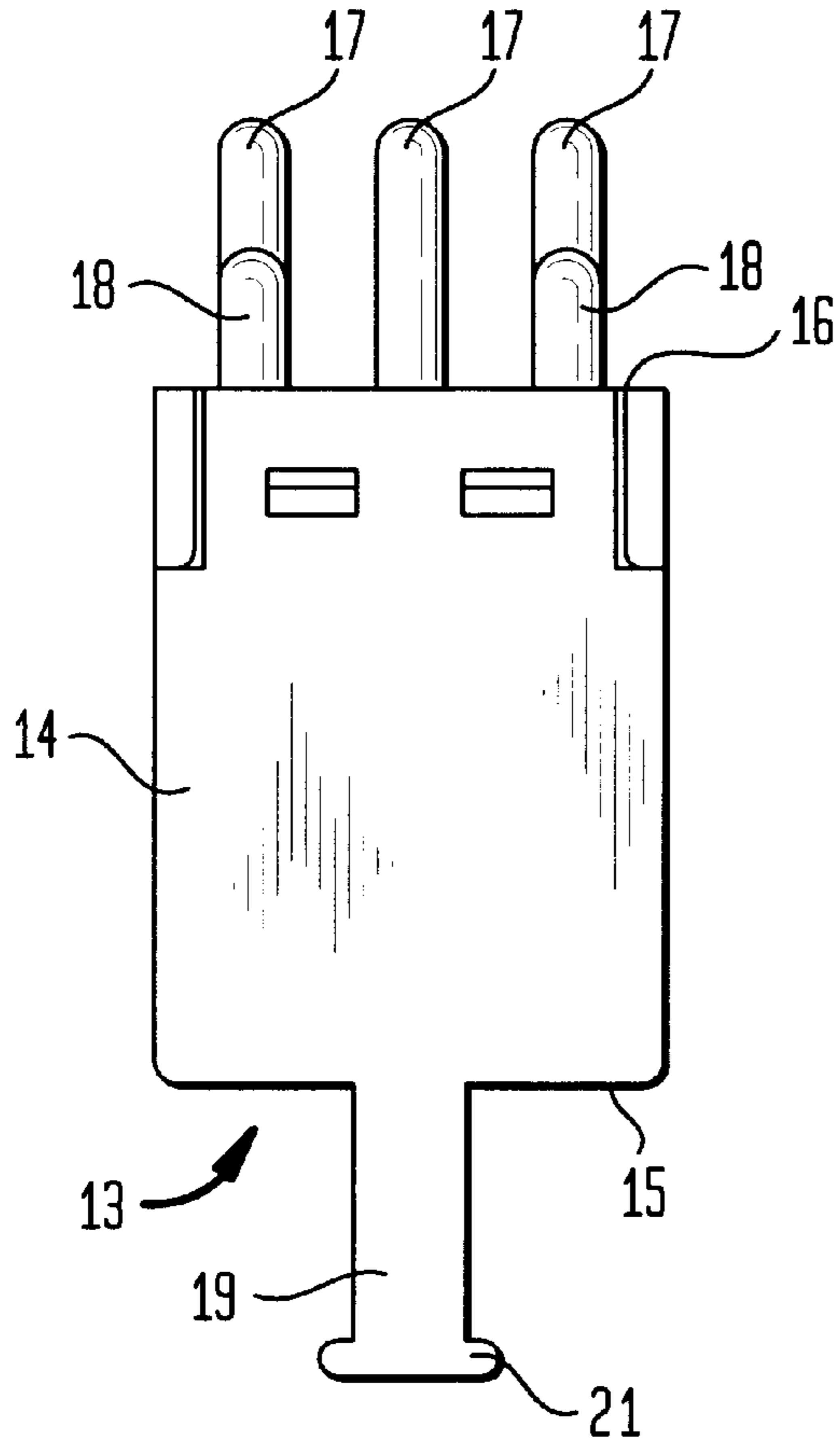
FIG. 2 (PRIOR ART)
