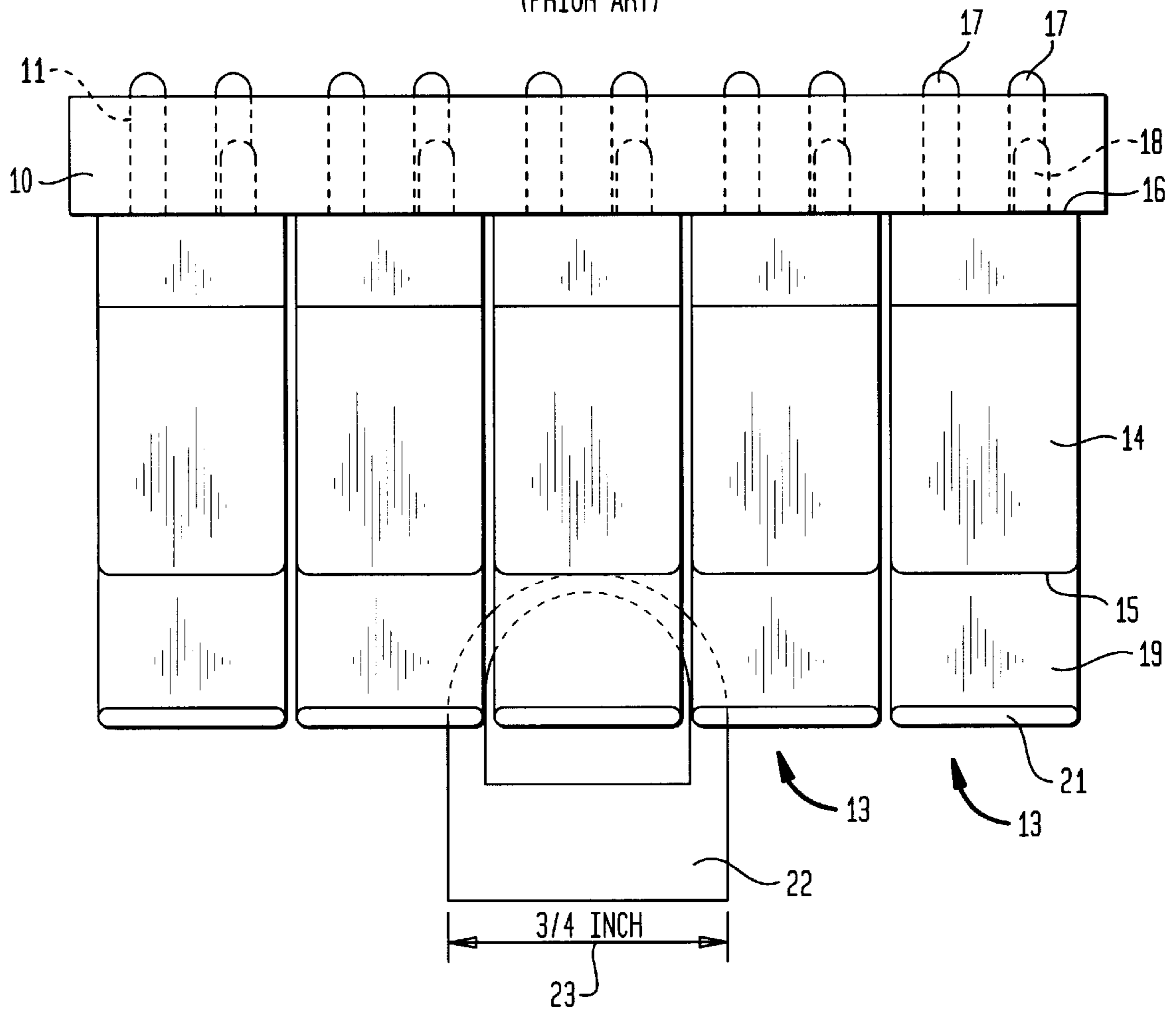
FIG. 5 (PRIOR ART)
