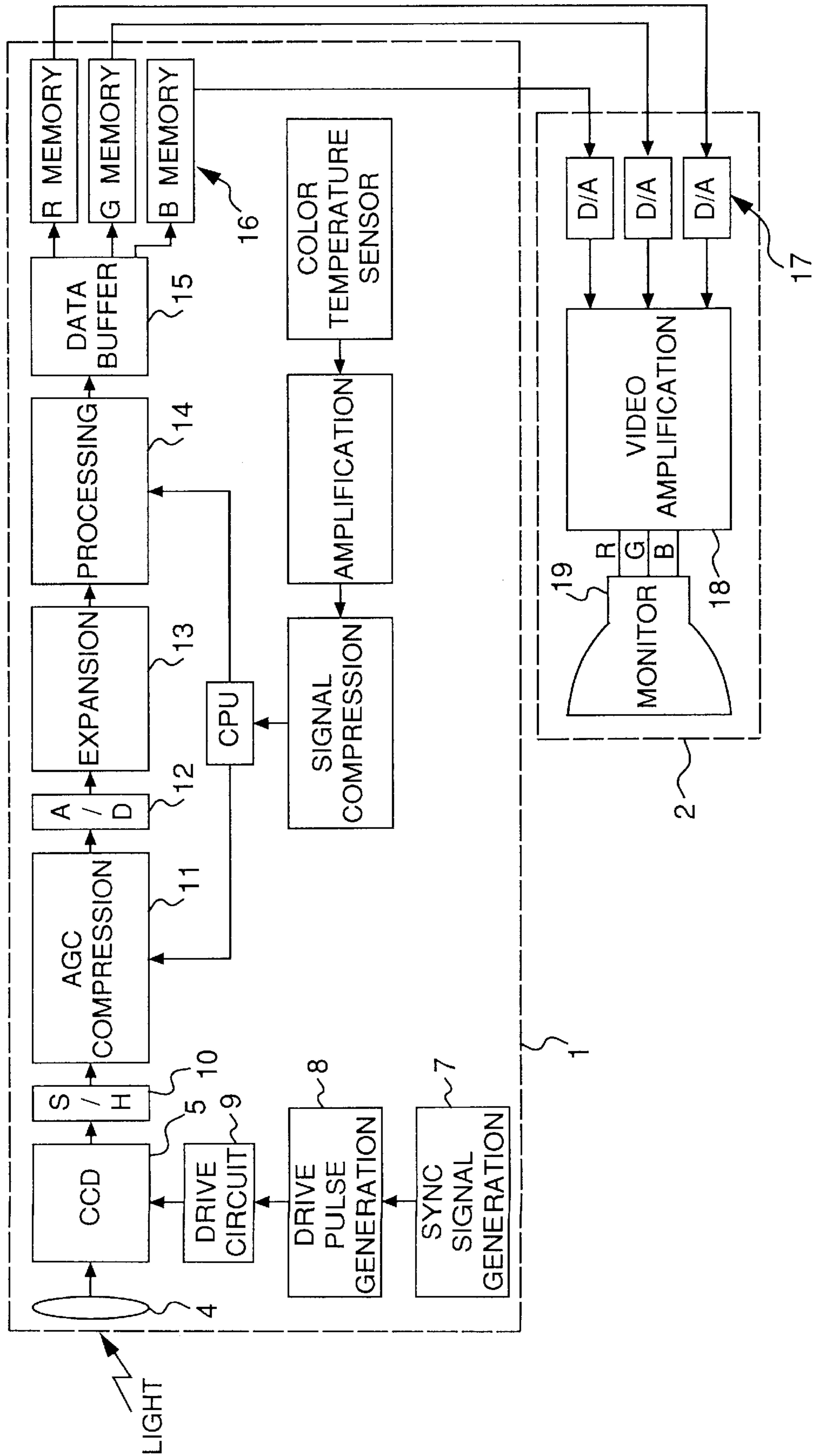
Fig.3 PRIOR ART
